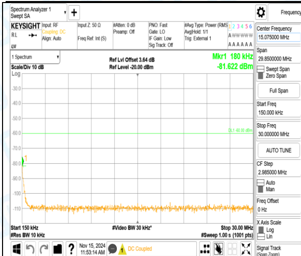
Band40_5MHz_16QAM_38750_1RB#0_1000~3000_1000~3000
