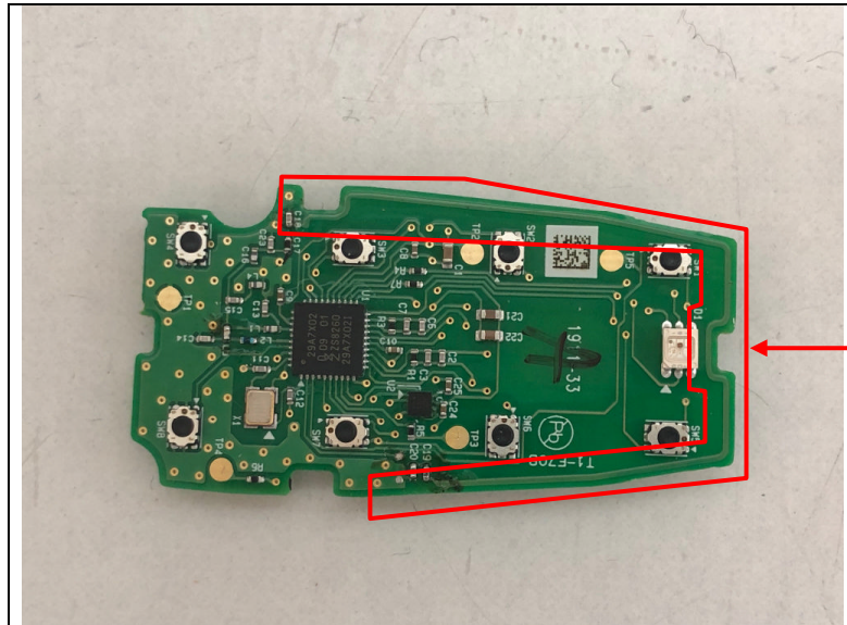
PCB Pattern Antenna
