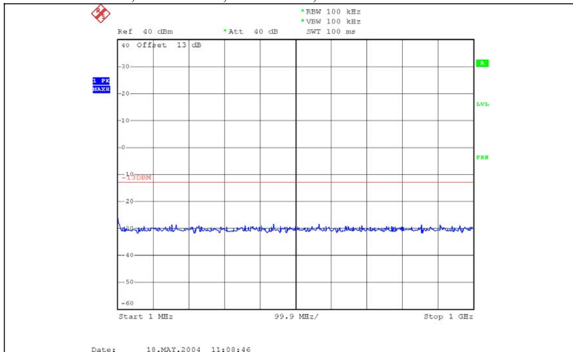
Plot 6.4.19) Out of Band Emissions at Antenna Terminals GMSK, Low channel, 1850.2 MHz, 1 MHz to 1 GHz
