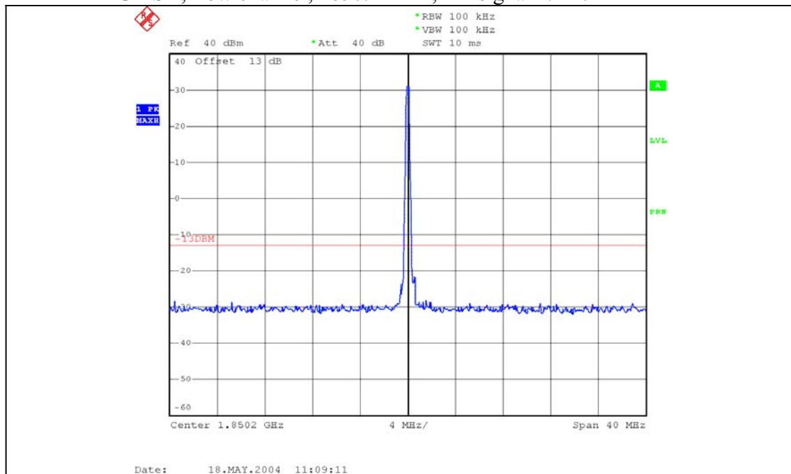
Plot 6.4.20) Out of Band Emissions at Antenna Terminals GMSK, Low channel, 1850.2 MHz, TX signal +/- 20 MHz
