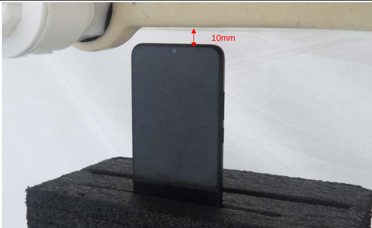
Picture 11: Top Edge, the distance from handset to the bottom of the Phantom is 10mm
