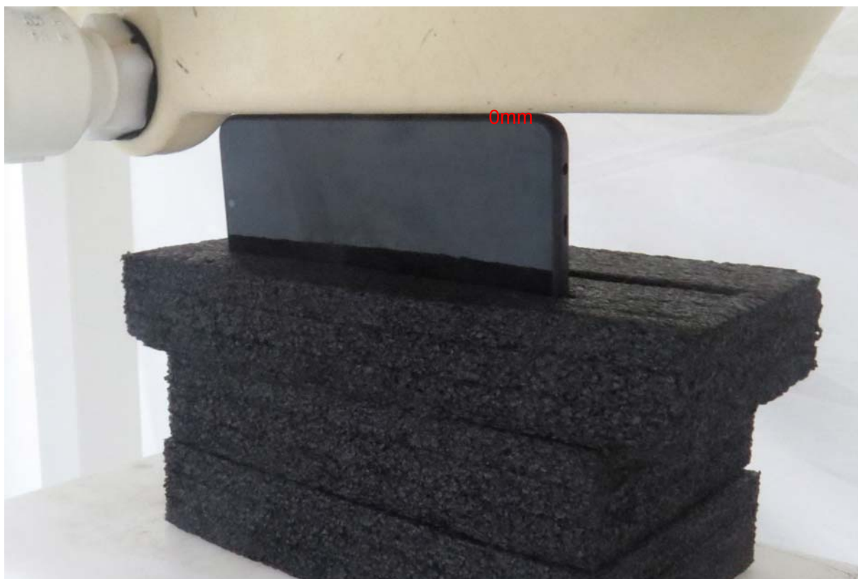
Picture 16: Right Edge, the distance from handset to the bottom of the Phantom is 0mm
