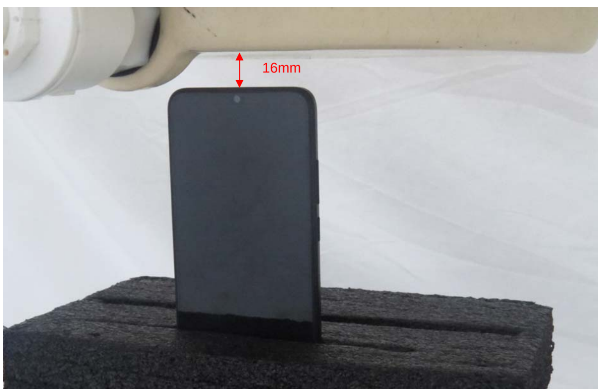
Picture 20: Top Edge, the distance from handset to the bottom of the Phantom is 16mm
