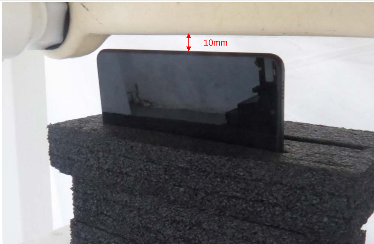
Picture 9: Left Edge, the distance from handset to the bottom of the Phantom is 10mm
