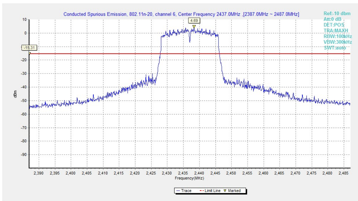
Fig.A.6.1.57 Conducted Spurious Emission (802.11n-HT20, Ch6, Center Frequency)
