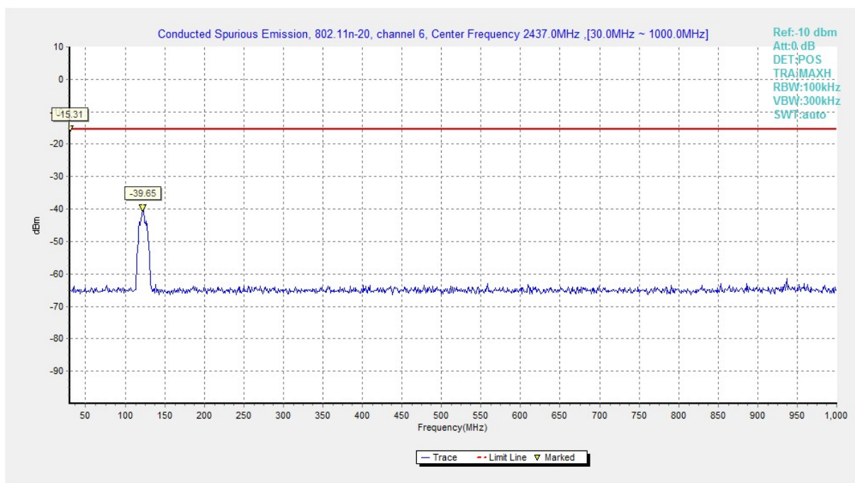
Fig.A.6.1.58 Conducted Spurious Emission (802.11n-HT20, Ch6, 30 MHz-1 GHz)
