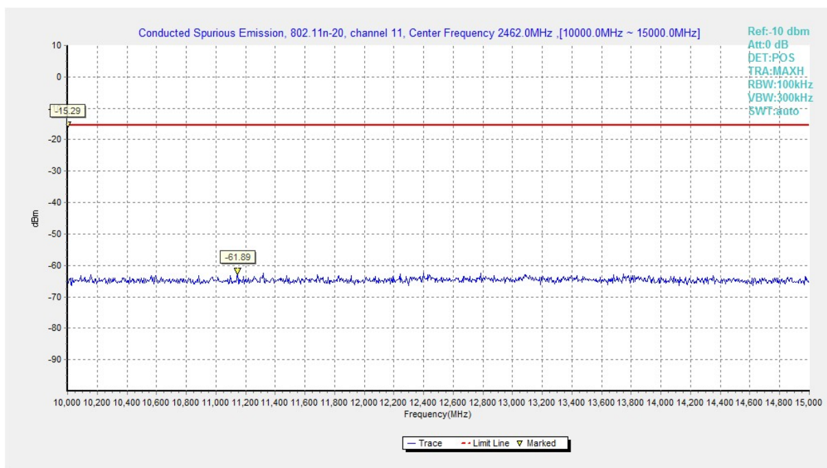
Fig.A.6.1.70 Conducted Spurious Emission (802.11n-HT20, Ch11, 10 GHz-15 GHz)
