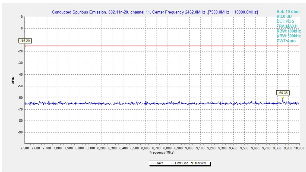
Fig.A.6.1.69 Conducted Spurious Emission (802.11n-HT20, Ch11, 7.5 GHz-10 GHz)
