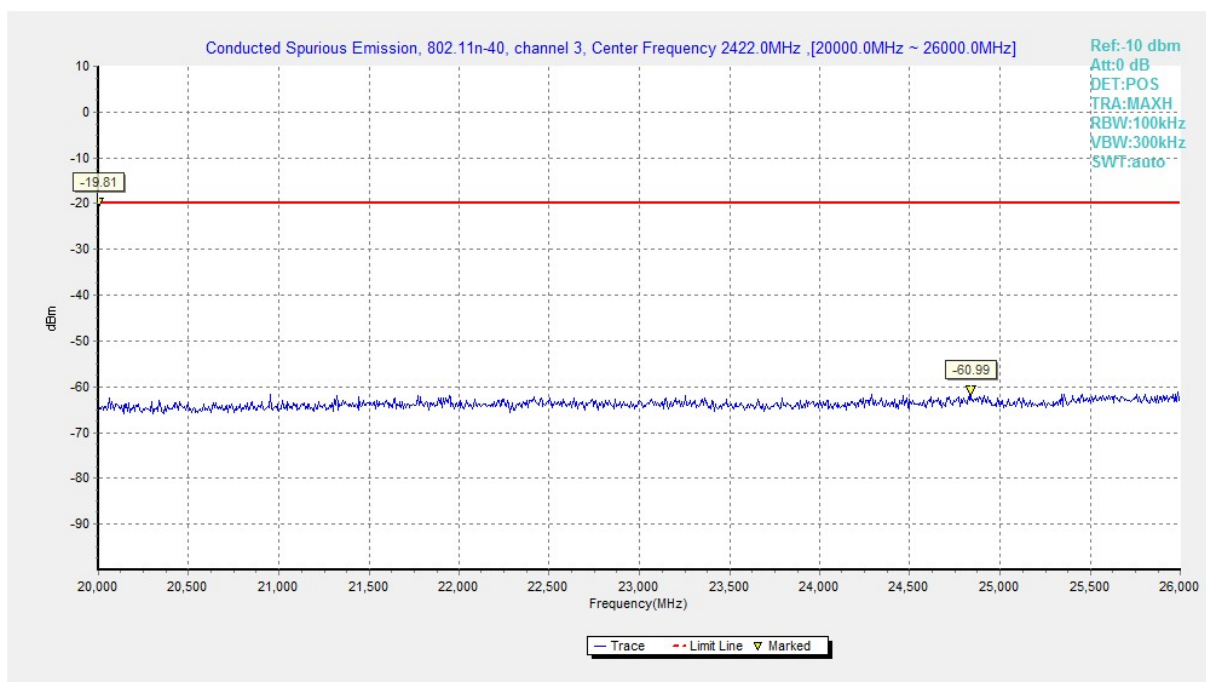
Fig.A.6.1.80 Conducted Spurious Emission (802.11n-HT40, Ch3, 20 GHz-26 GHz)
