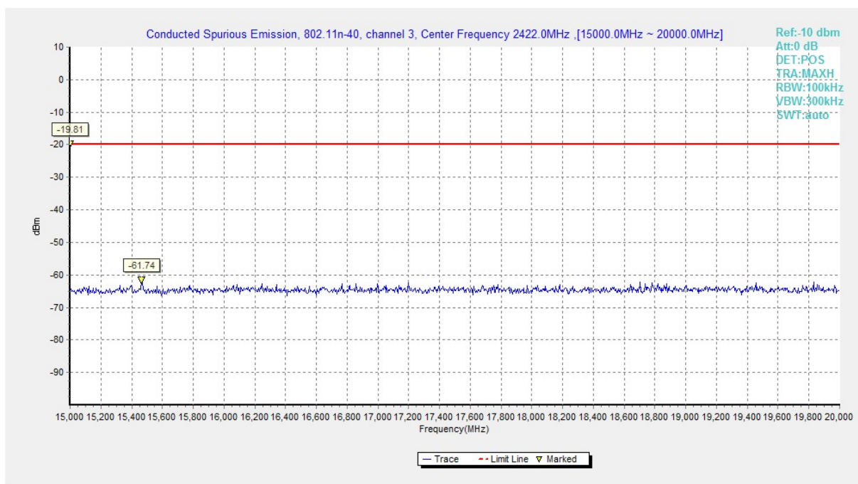
Fig.A.6.1.79 Conducted Spurious Emission (802.11n-HT40, Ch3, 15 GHz-20 GHz)
