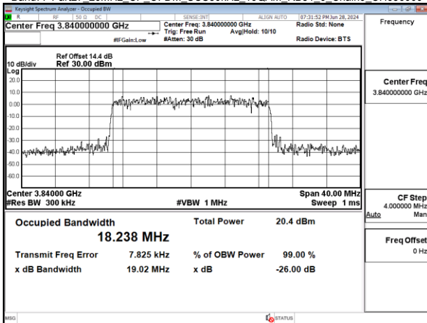
Band77-Part27_20MHz_CP_OFDM_SCS30kHz_16QAM_RB51_0_Chain0_CH656000
