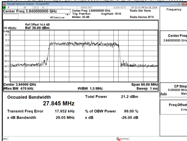
Band77-Part27_30MHz_CP_OFDM_SCS30kHz_QPSK_RB78_0_Chain0_CH656000
