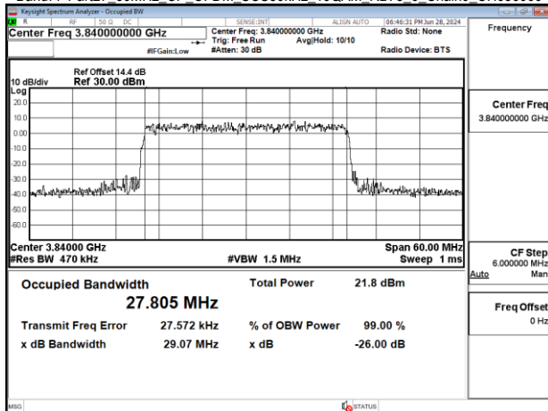
Band77-Part27_30MHz_CP_OFDM_SCS30kHz_16QAM_RB78_0_Chain0_CH656000
