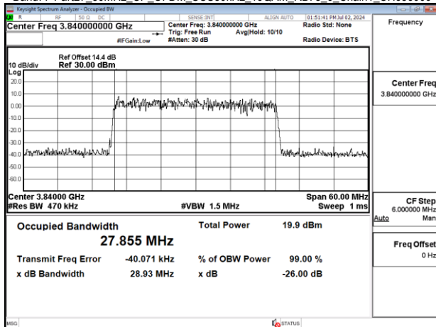
Band77-Part27_30MHz_CP_OFDM_SCS30kHz_16QAM_RB78_0_Chain1_CH656000
