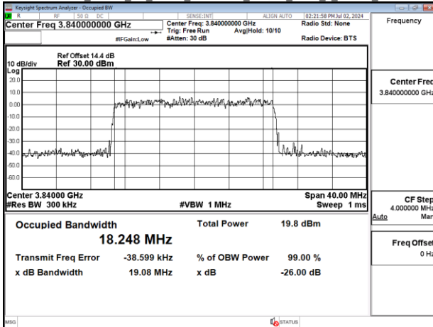
Band77-Part27_20MHz_CP_OFDM_SCS30kHz_64QAM_RB51_0_Chain1_CH656000
