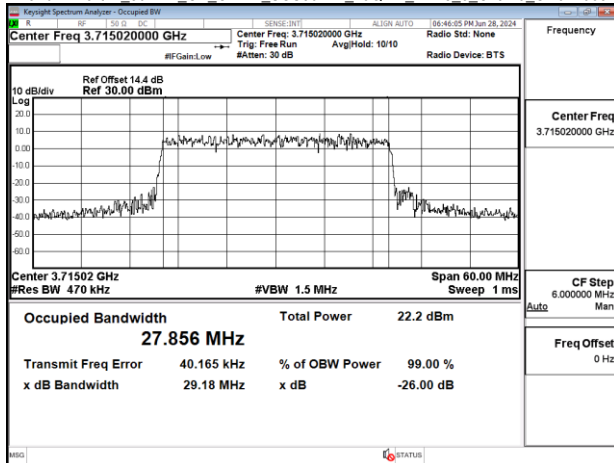
Band77-Part27_30MHz_CP_OFDM_SCS30kHz_16QAM_RB78_0_Chain0_CH656000
