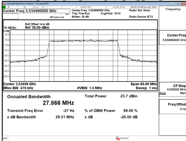
Band77-Part27_30MHz_CP_OFDM_SCS30kHz_16QAM_RB78_0_Chain0_CH647668
