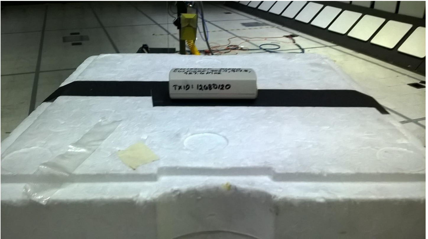
Figure 4 - Radiated Emissions Test Setup, 1 – 19 GHz
