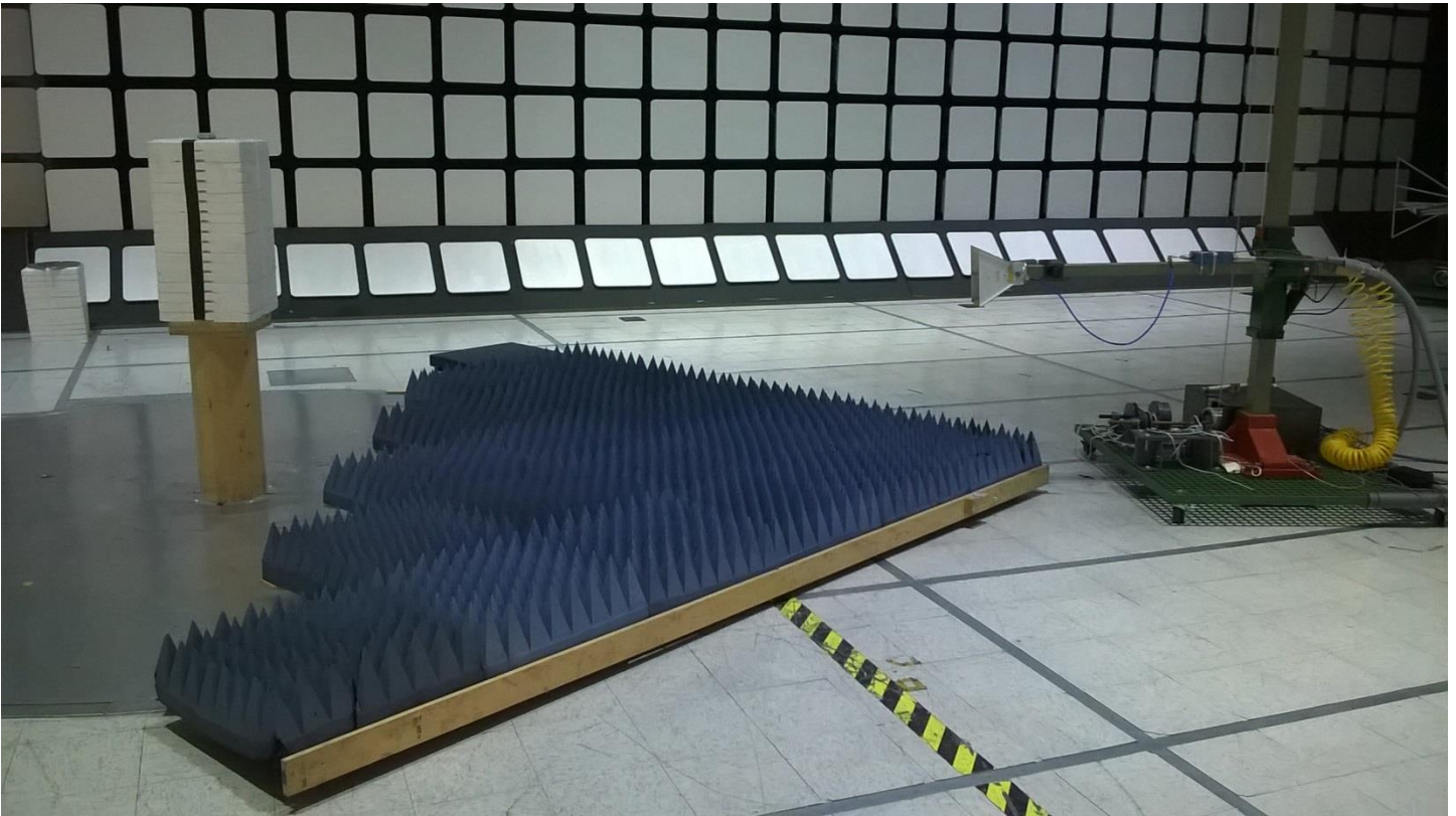
Figure 3 - Radiated Emissions Test Setup, 1 – 19 GHz
