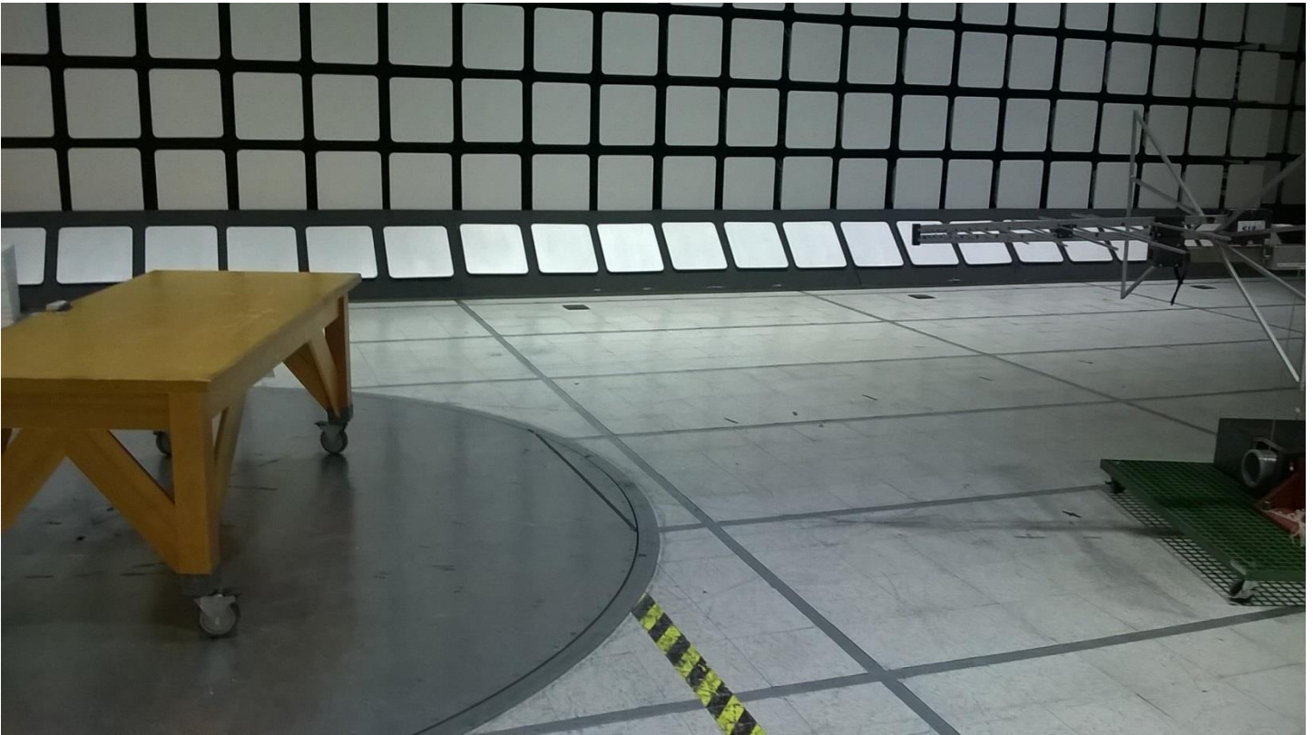
Figure 1 – Radiated Emissions Test Setup, 30MHz – 1GHz
