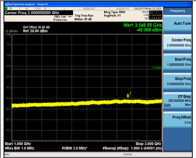
Band5_3MHz_QPSK_20635_15RB#0_1000~3000_1000~3000
