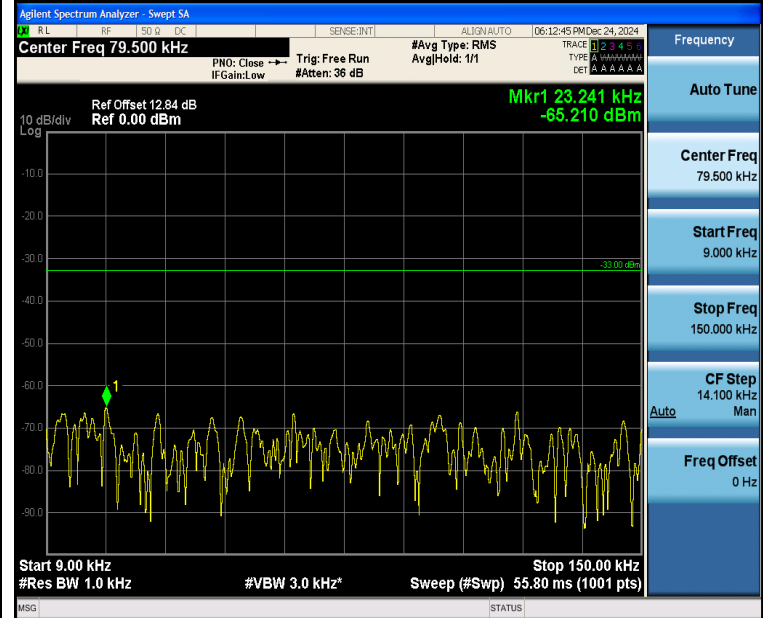
Band5_3MHz_16QAM_20415_1RB#0_0.009~0.15_0.009~0.15
