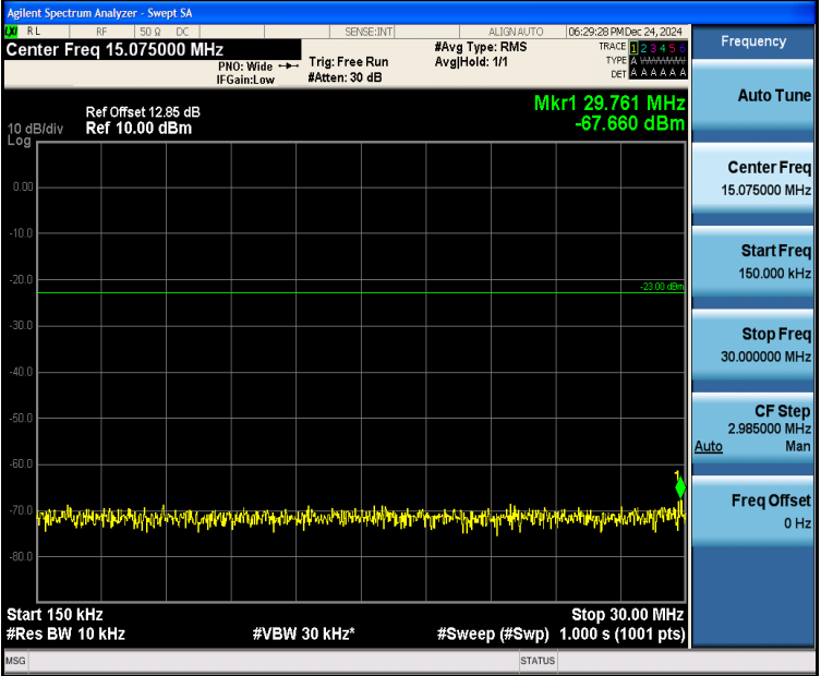
Band5_3MHz_QPSK_20635_15RB#0_0.15~30_0.15~30
