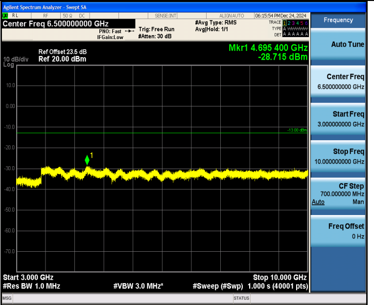
Band5_3MHz_16QAM_20415_1RB#14_3000~10000_3000~10000
