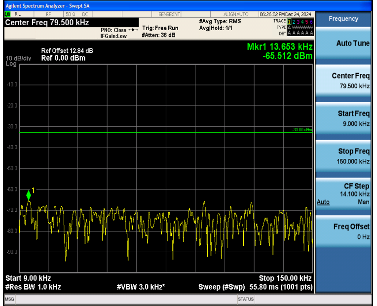
Band5_3MHz_16QAM_20635_1RB#0_0.009~0.15_0.009~0.15
