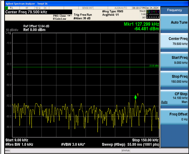
Band5_3MHz_QPSK_20525_1RB#0_0.009~0.15_0.009~0.15
