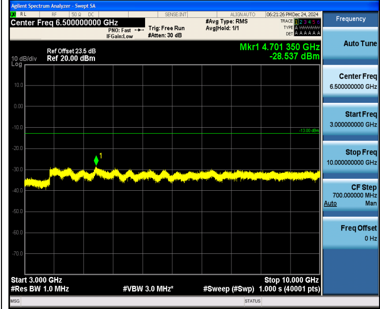
Band5_3MHz_QPSK_20525_1RB#14_3000~10000_3000~10000
