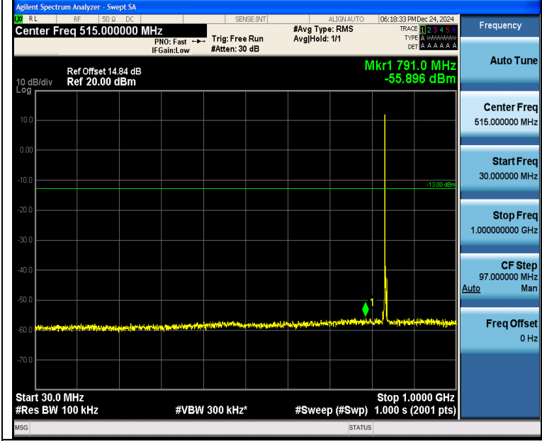
Band5_3MHz_QPSK_20525_1RB#0_30~1000_30~1000
