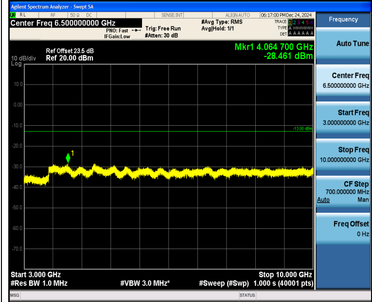
Band5_3MHz_QPSK_20415_15RB#0_3000~10000_3000~10000
