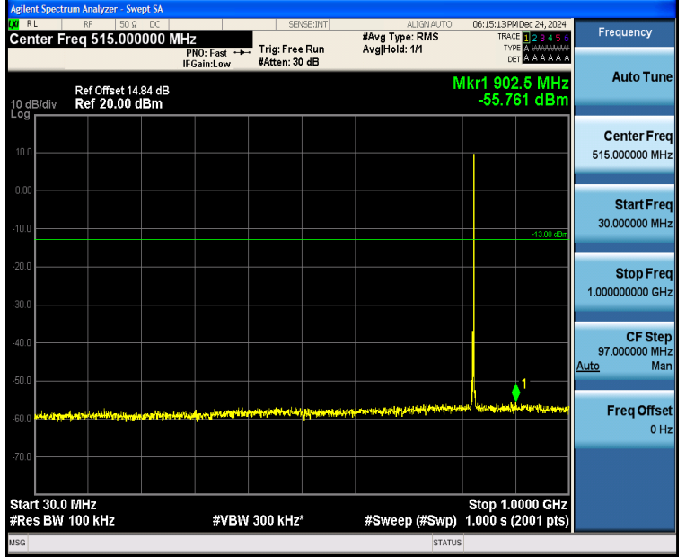
Band5_3MHz_16QAM_20415_1RB#14_30~1000_30~1000
