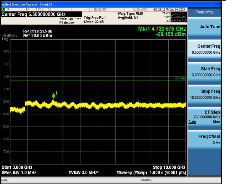
Band5_3MHz_16QAM_20635_1RB#14_3000~10000_3000~10000
