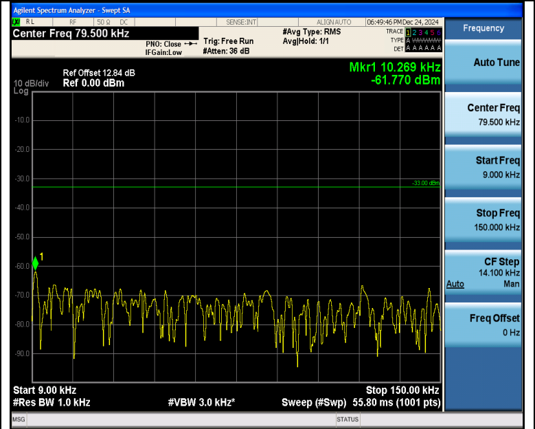
Band5_5MHz_16QAM_20425_1RB#0_0.009~0.15_0.009~0.15
