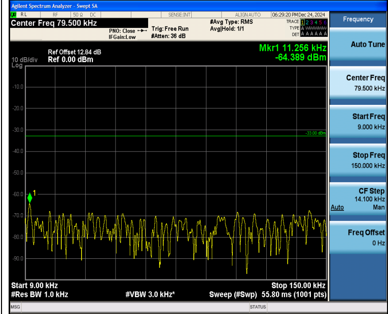
Band5_3MHz_QPSK_20635_15RB#0_0.009~0.15_0.009~0.15
