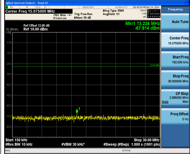
Band5_5MHz_16QAM_20425_1RB#0_0.15~30_0.15~30
