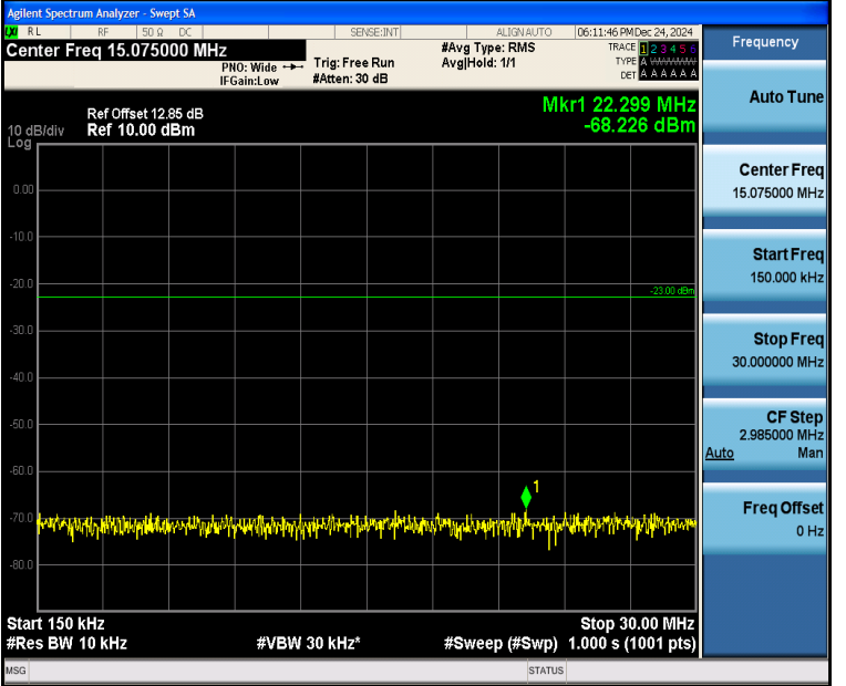
Band5_3MHz_QPSK_20415_1RB#0_0.15~30_0.15~30
