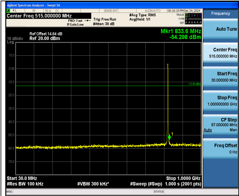
Band5_3MHz_QPSK_20415_15RB#0_30~1000_30~1000
