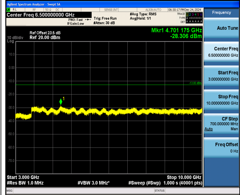
Band5_3MHz_QPSK_20635_15RB#0_3000~10000_3000~10000
