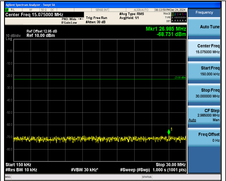
Band5_3MHz_QPSK_20415_1RB#14_0.15~30_0.15~30
