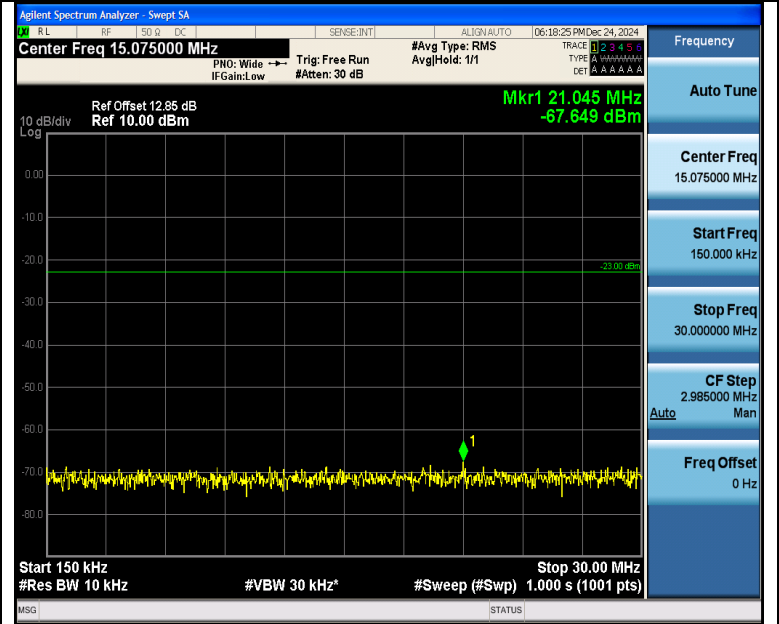
Band5_3MHz_QPSK_20525_1RB#0_0.15~30_0.15~30
