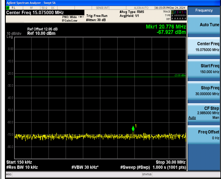
Band5_3MHz_QPSK_20415_1RB#14_0.15~30_0.15~30
