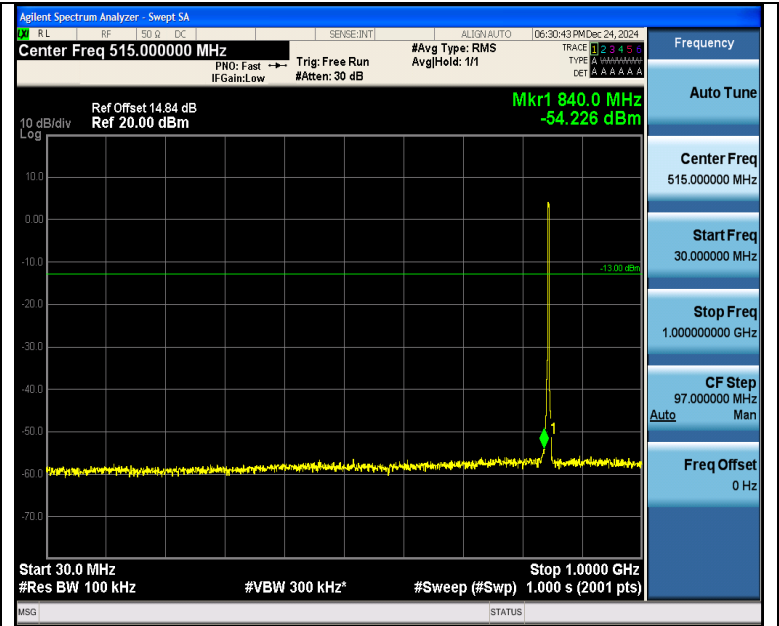
Band5_3MHz_16QAM_20635_15RB#0_30~1000_30~1000
