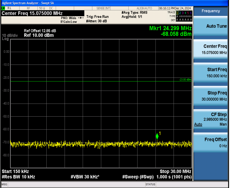
Band5_3MHz_QPSK_20415_15RB#0_0.15~30_0.15~30
