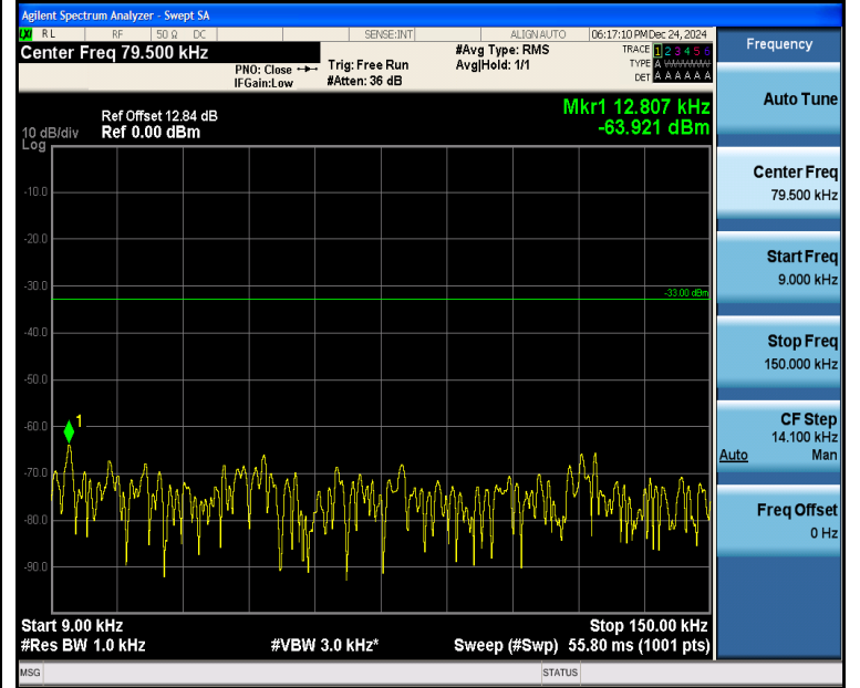
Band5_3MHz_16QAM_20415_15RB#0_0.009~0.15_0.009~0.15
