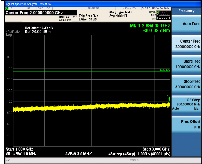
Band5_3MHz_16QAM_20635_1RB#14_1000~3000_1000~3000
