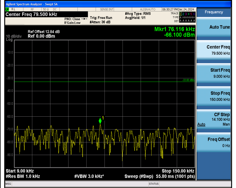
Band5_3MHz_16QAM_20635_15RB#0_0.009~0.15_0.009~0.15
