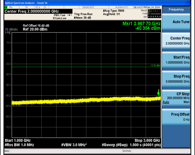
Band5_3MHz_QPSK_20415_1RB#14_1000~3000_1000~3000
