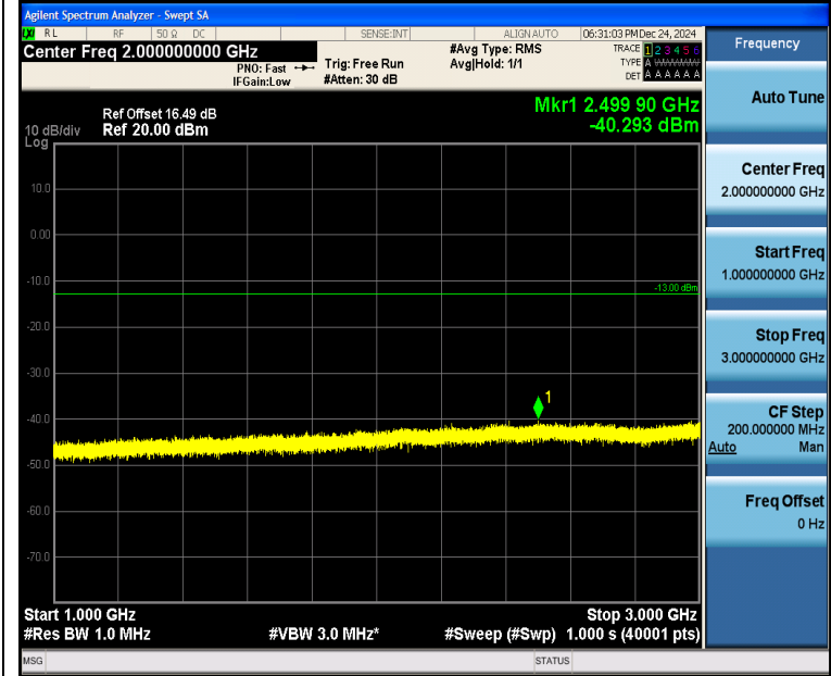
Band5_3MHz_16QAM_20635_15RB#0_1000~3000_1000~3000
