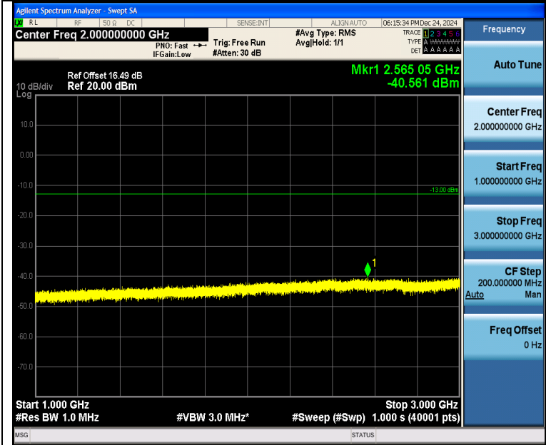
Band5_3MHz_16QAM_20415_1RB#14_1000~3000_1000~3000
