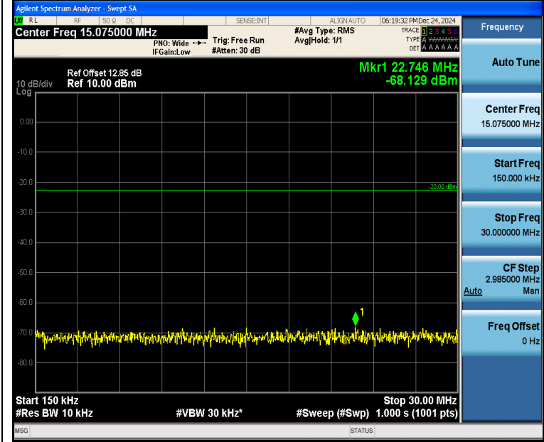
Band5_3MHz_16QAM_20525_1RB#0_0.15~30_0.15~30
