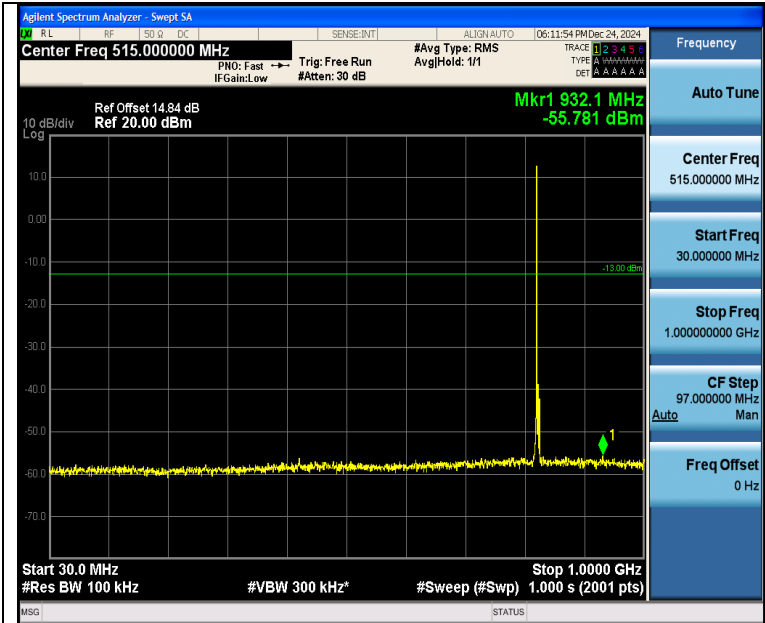
Band5_3MHz_QPSK_20415_1RB#0_30~1000_30~1000
