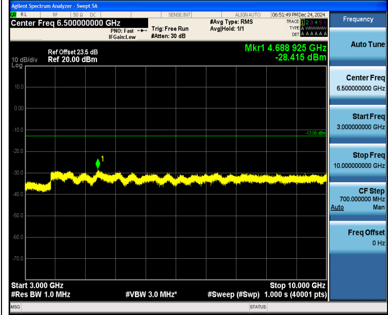
Band5_5MHz_QPSK_20425_1RB#24_3000~10000_3000~10000
