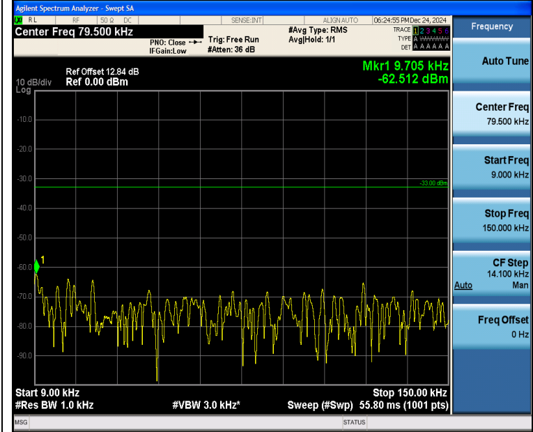
Band5_3MHz_QPSK_20635_1RB#0_0.009~0.15_0.009~0.15
