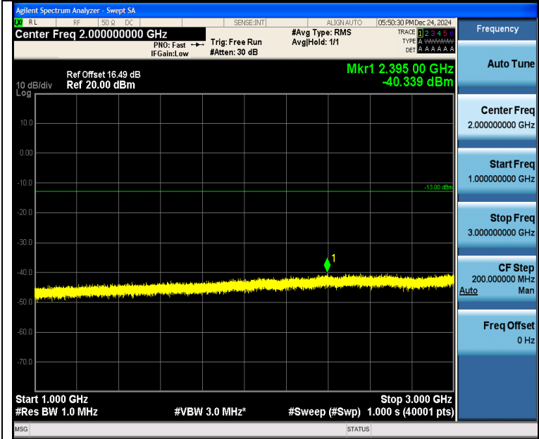
Band5_1.4MHz_16QAM_20643_6RB#0_1000~3000_1000~3000
