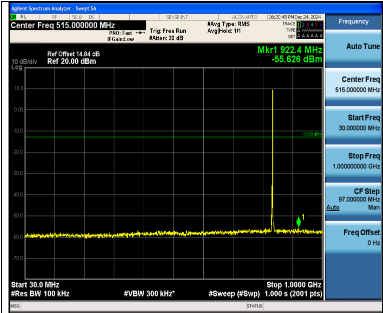
Band5_3MHz_QPSK_20525_1RB#14_30~1000_30~1000
