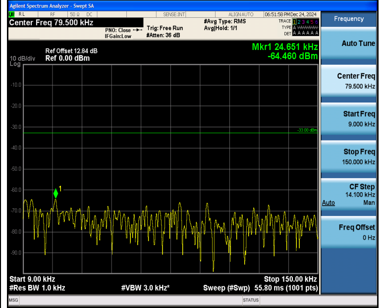
Band5_5MHz_16QAM_20425_1RB#24_0.009~0.15_0.009~0.15
