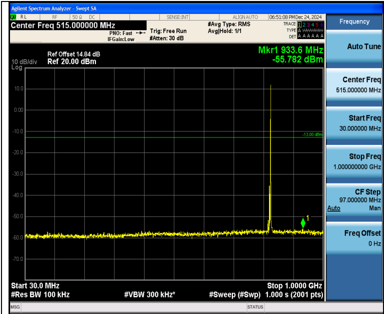
Band5_5MHz_QPSK_20425_1RB#24_30~1000_30~1000
