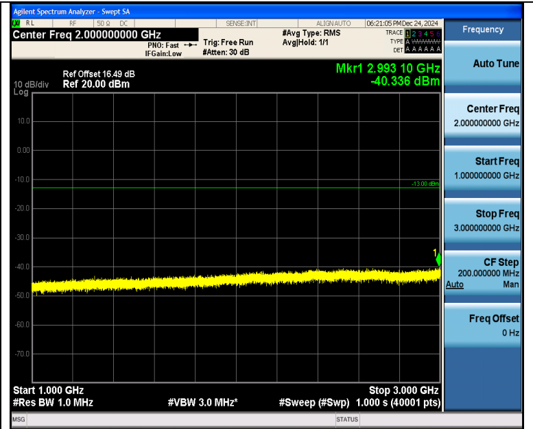
Band5_3MHz_QPSK_20525_1RB#14_1000~3000_1000~3000
