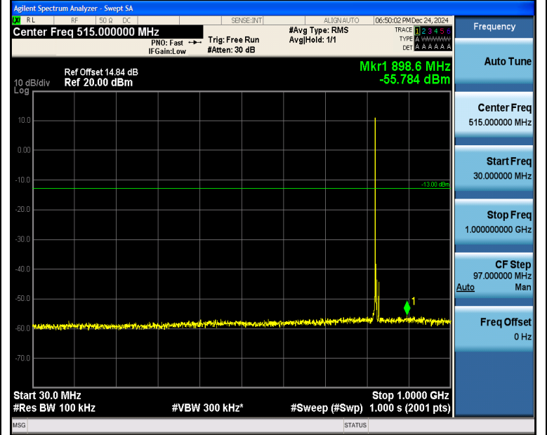
Band5_5MHz_16QAM_20425_1RB#0_30~1000_30~1000
