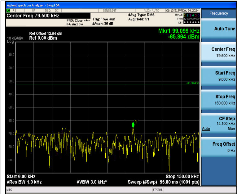
Band5_3MHz_QPSK_20415_1RB#14_0.009~0.15_0.009~0.15
