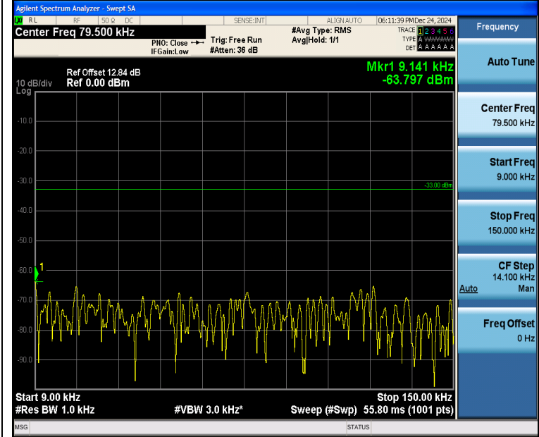
Band5_3MHz_QPSK_20415_1RB#0_0.009~0.15_0.009~0.15
