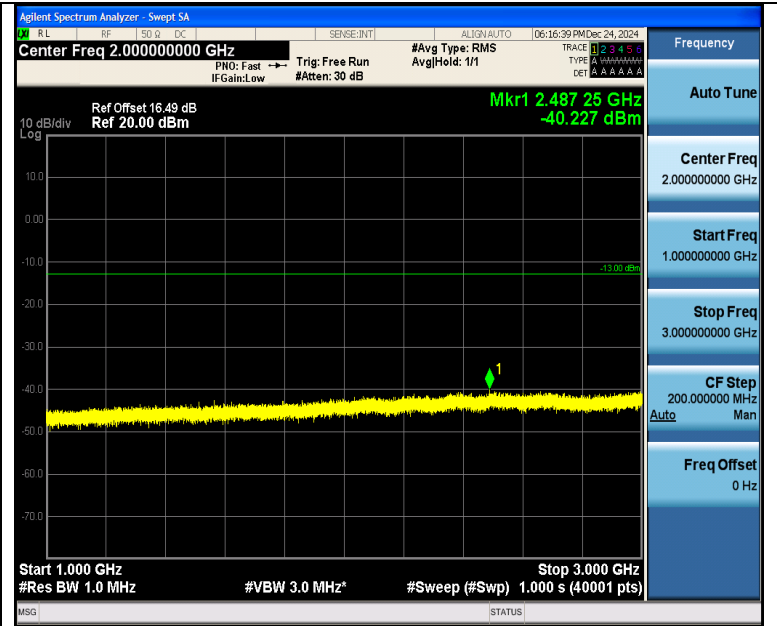
Band5_3MHz_QPSK_20415_15RB#0_1000~3000_1000~3000
