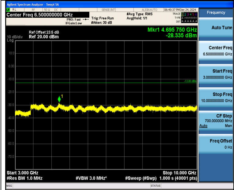
Band5_5MHz_QPSK_20425_1RB#0_3000~10000_3000~10000
