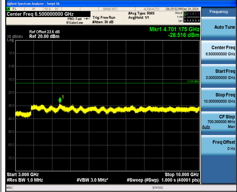
Band5_3MHz_QPSK_20635_1RB#0_3000~10000_3000~10000
