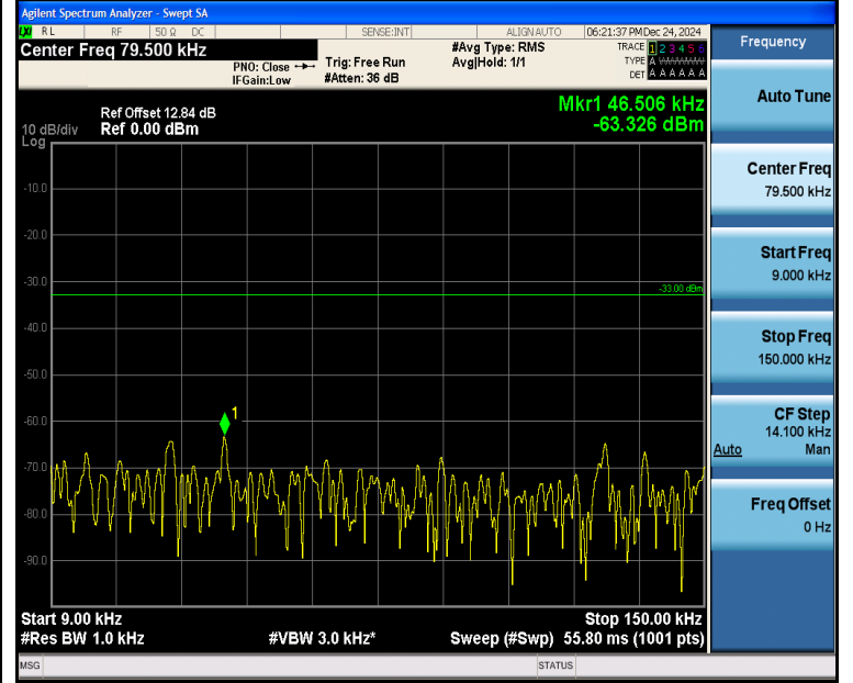
Band5_3MHz_16QAM_20525_1RB#14_0.009~0.15_0.009~0.15
