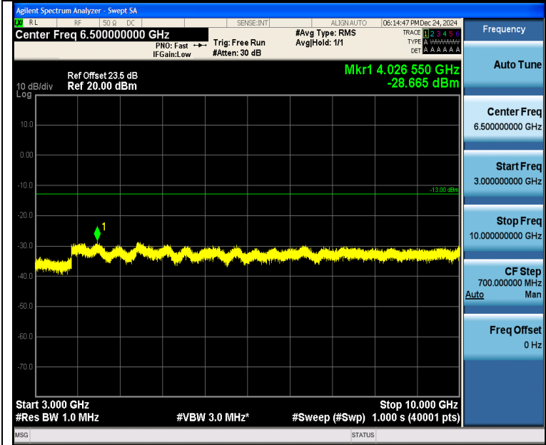
Band5_3MHz_QPSK_20415_1RB#14_3000~10000_3000~10000
