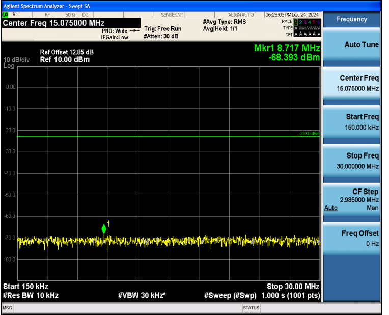
Band5_3MHz_QPSK_20635_1RB#0_0.15~30_0.15~30
