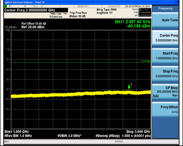
Band5_3MHz_QPSK_20525_1RB#0_1000~3000_1000~3000
