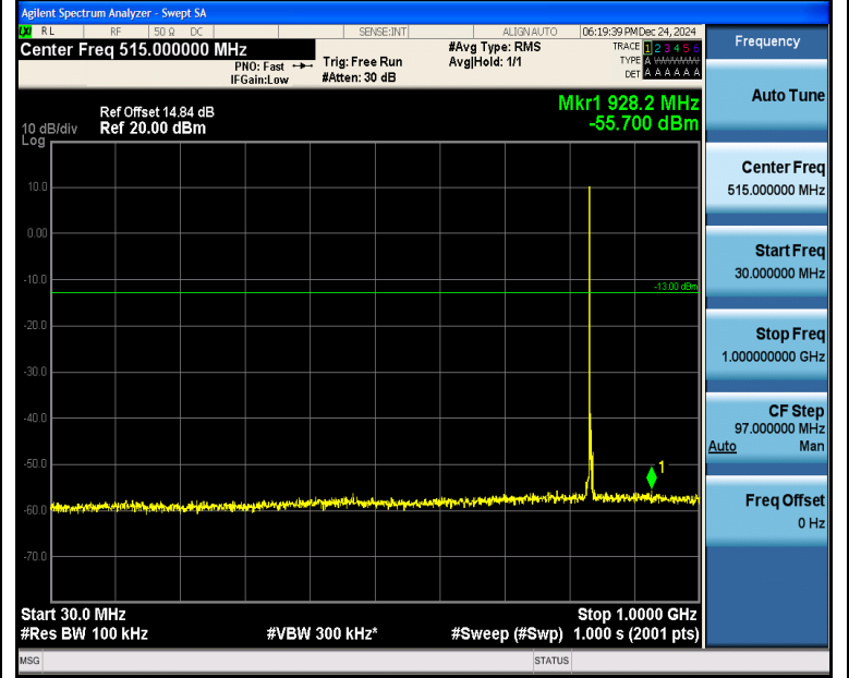
Band5_3MHz_16QAM_20525_1RB#0_30~1000_30~1000
