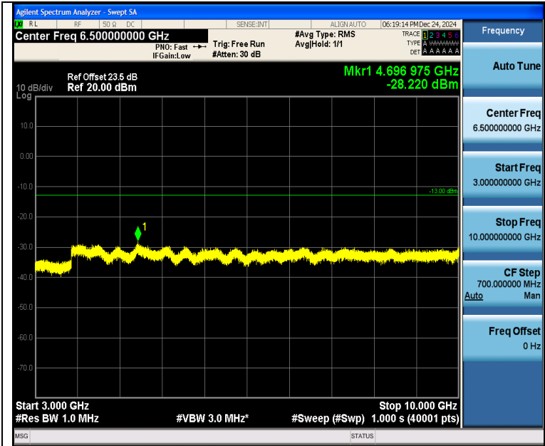
Band5_3MHz_QPSK_20525_1RB#0_3000~10000_3000~10000
