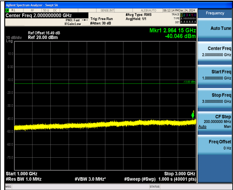
Band5_3MHz_QPSK_20415_1RB#0_1000~3000_1000~3000
