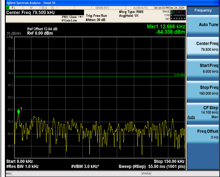
Band5_3MHz_QPSK_20415_15RB#0_0.009~0.15_0.009~0.15
