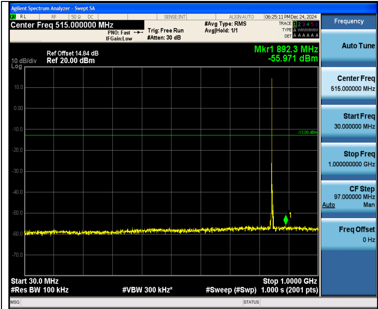
Band5_3MHz_QPSK_20635_1RB#0_30~1000_30~1000
