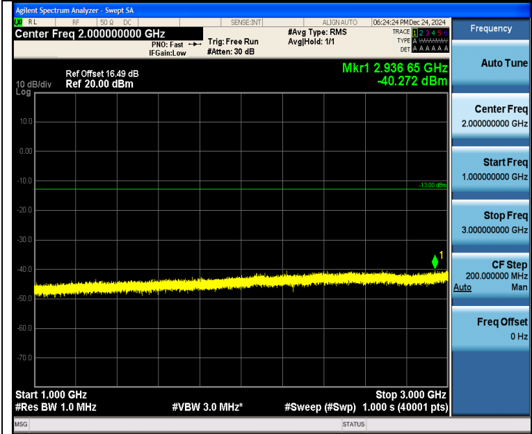
Band5_3MHz_16QAM_20525_15RB#0_1000~3000_1000~3000
