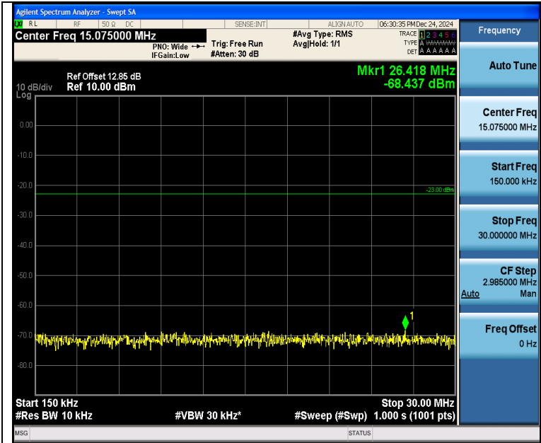
Band5_3MHz_16QAM_20635_15RB#0_0.15~30_0.15~30
