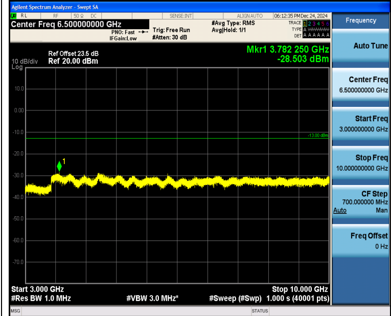
Band5_3MHz_QPSK_20415_1RB#0_3000~10000_3000~10000
