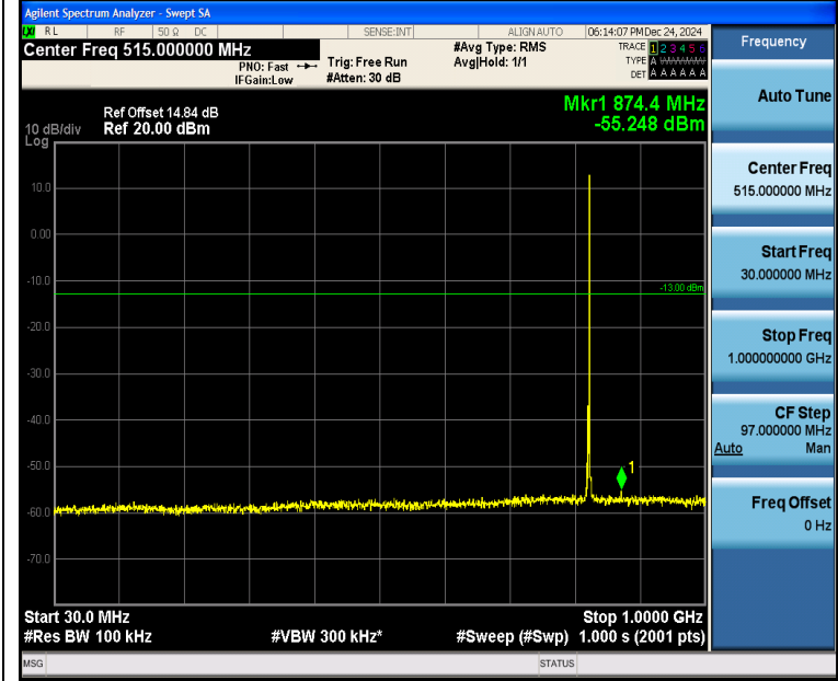
Band5_3MHz_QPSK_20415_1RB#14_30~1000_30~1000
