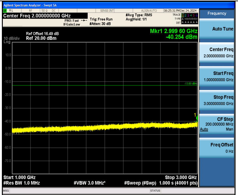
Band5_3MHz_QPSK_20635_1RB#0_1000~3000_1000~3000
