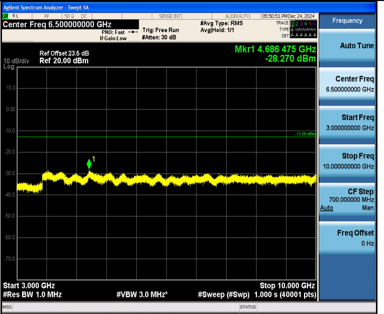
Band5_1.4MHz_16QAM_20643_6RB#0_3000~10000_3000~10000
