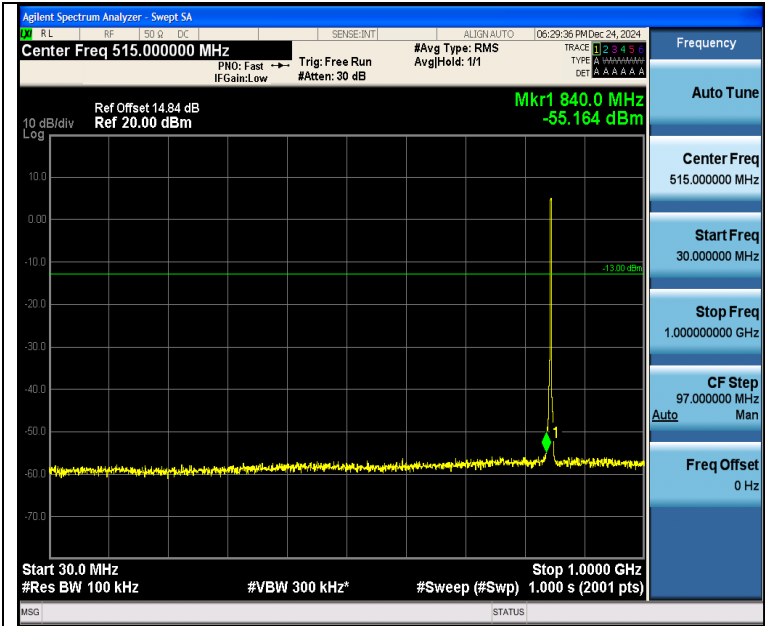
Band5_3MHz_QPSK_20635_15RB#0_30~1000_30~1000
