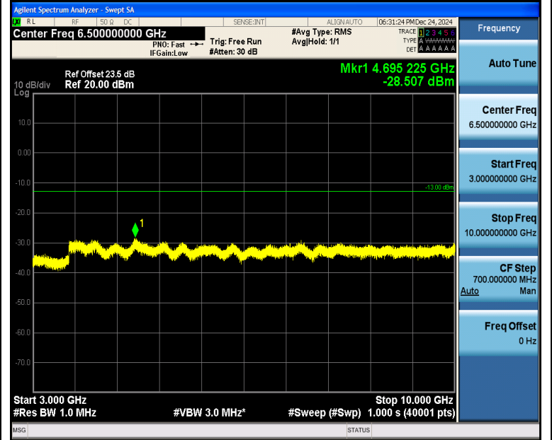
Band5_3MHz_16QAM_20635_15RB#0_3000~10000_3000~10000
