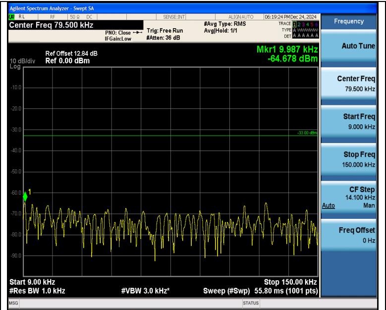
Band5_3MHz_16QAM_20525_1RB#0_0.009~0.15_0.009~0.15
