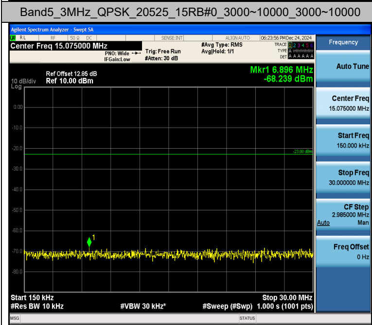
Band5_3MHz_QPSK_20525_15RB#0_3000~10000_3000~10000
