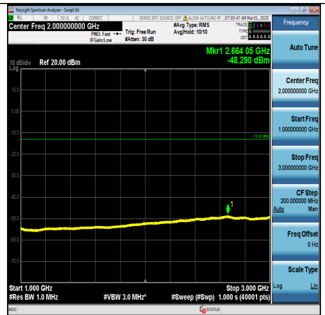
Band12-10MHz-QPSK-23130-1RB#0-1000~3000-PASS
