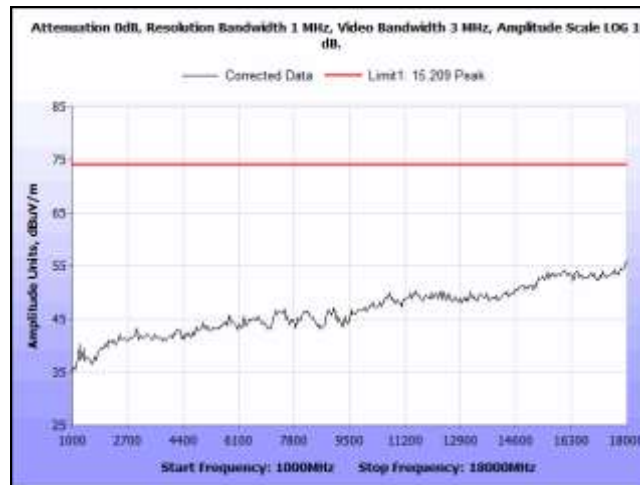
Plot 28. Radiated Emissions, NP20, 1 GHz – 18 GHz, Peak Bluetooth and FCC Cellular
