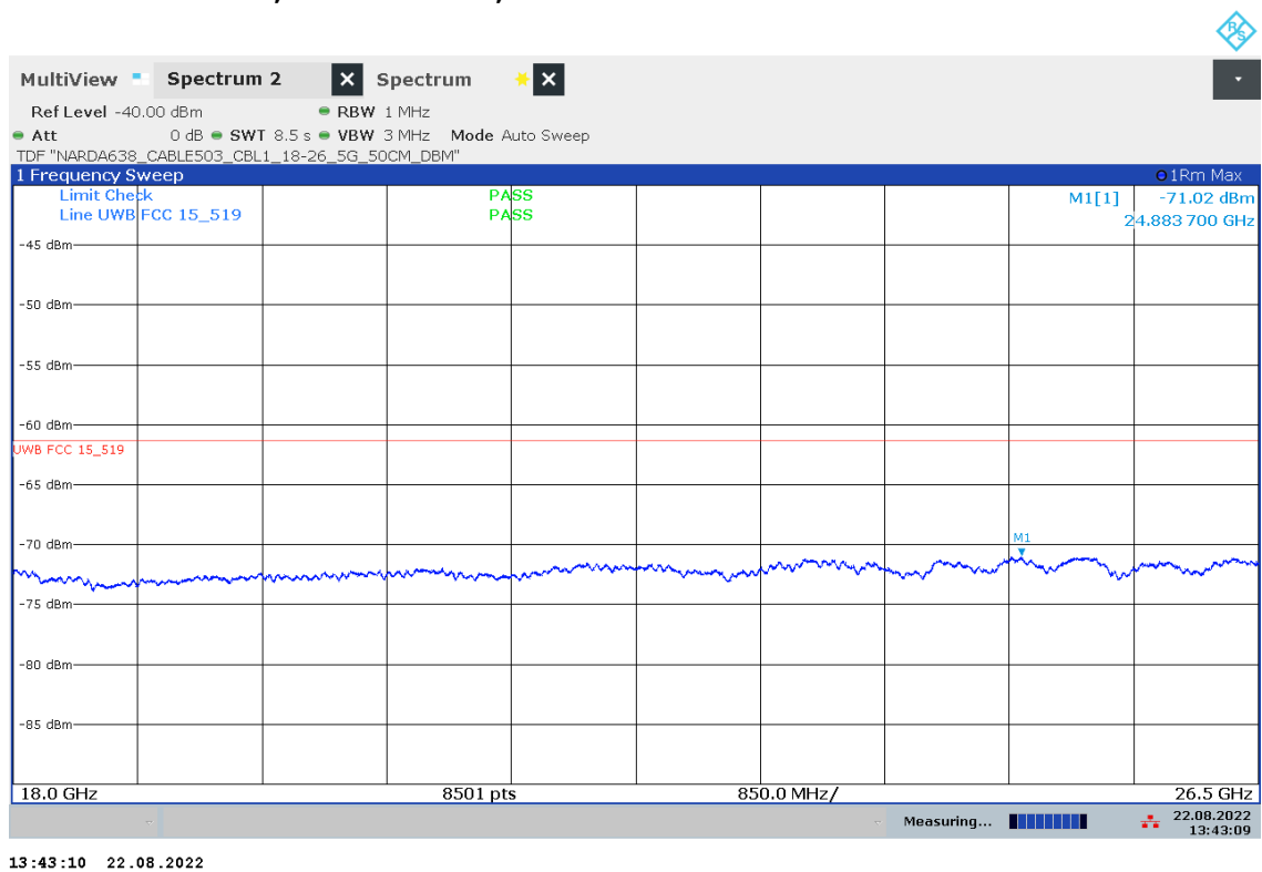
Plot 18: 18 GHz to 26.5 GHz, UWB test mode, Channel 2
