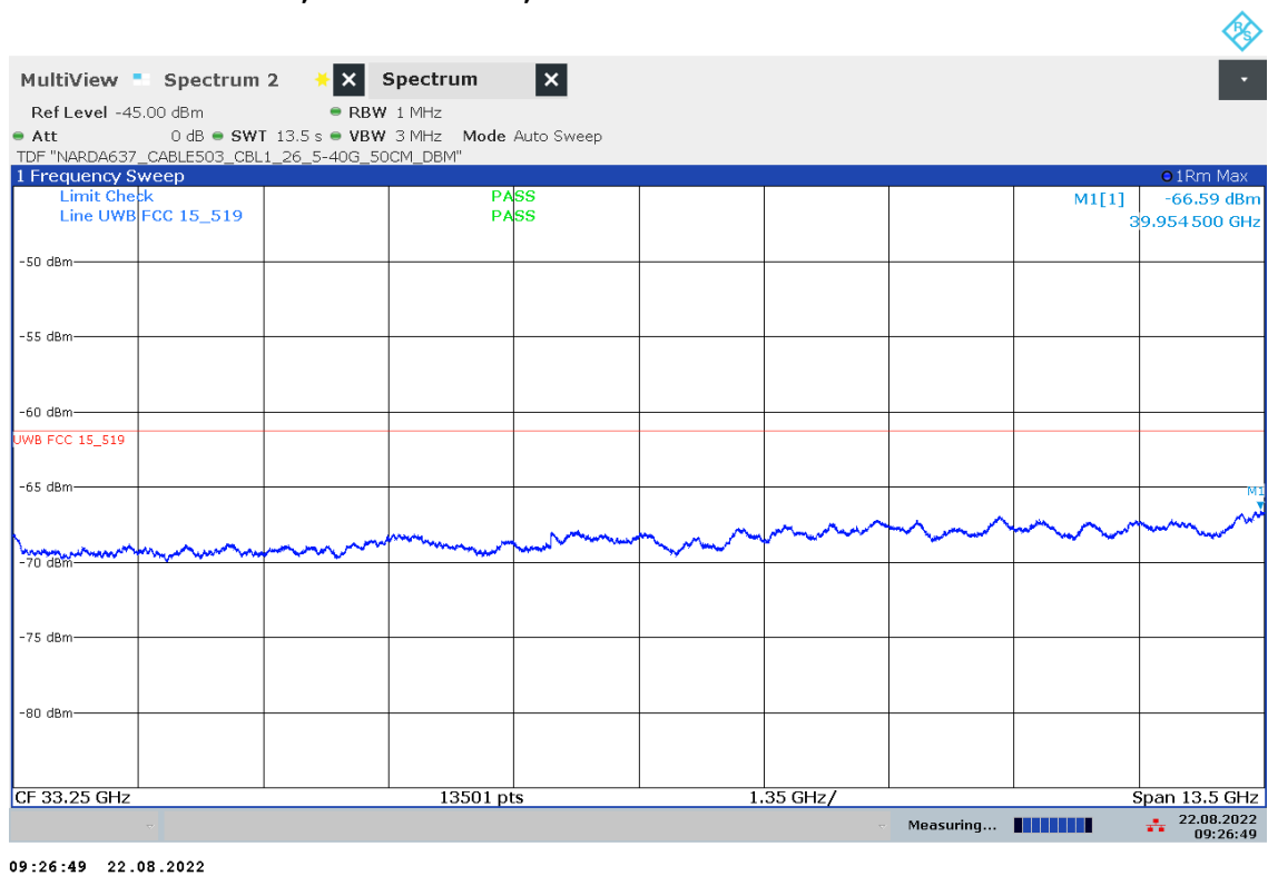
Plot 20: 26.5 GHz to 40.0 GHz, UWB test mode, Channel 2
