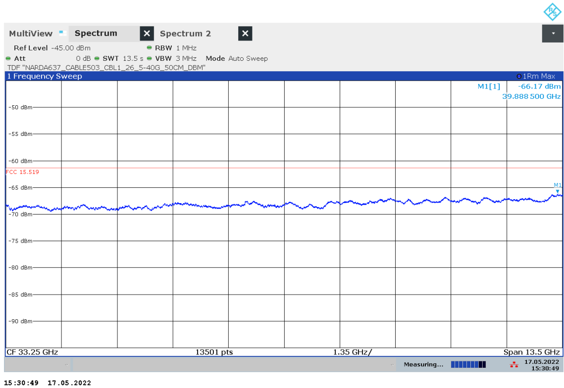
Plot 19: 26.5 GHz to 40.0 GHz, UWB test mode, Channel 1
