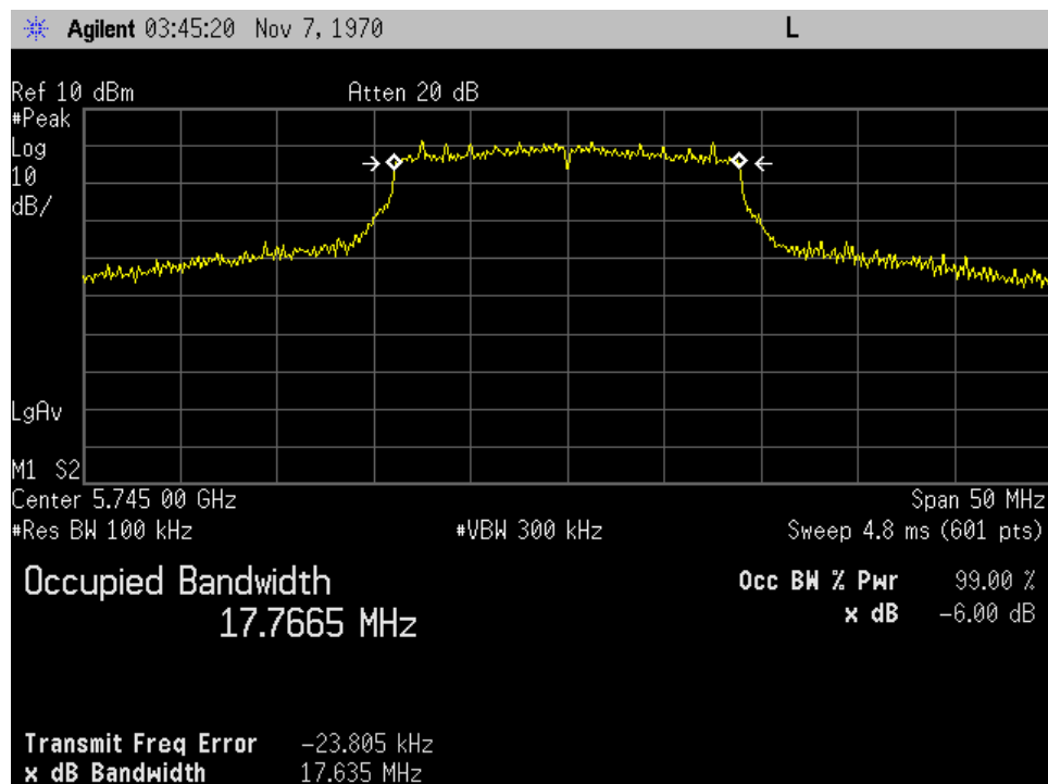
p20c0005_OCBW_20MHZ_Low Channel_UNII-3_AC_P1
