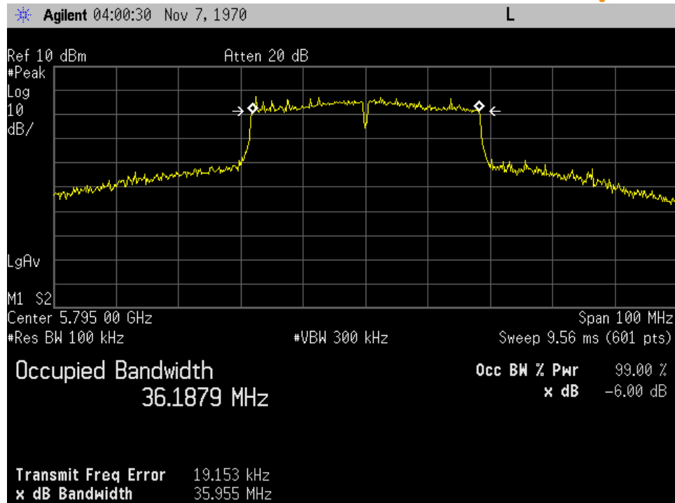
p20c0005_OCBW_40MHZ_High Channel_UNII-3_AC_P1
