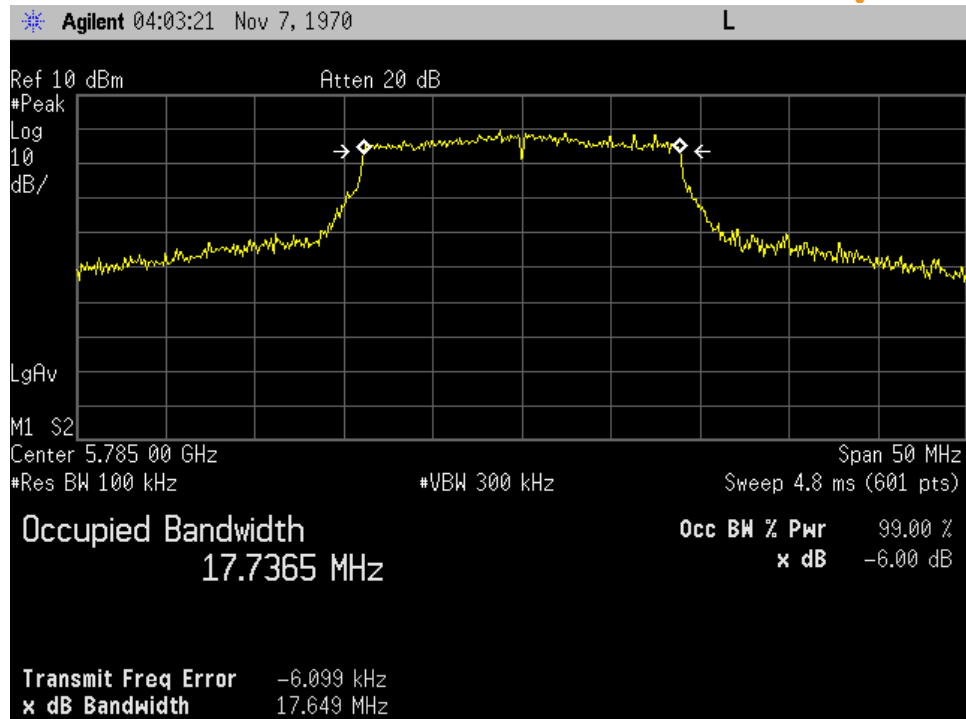
p20c0005_OCBW_20MHZ_Mid Channel_UNII-3_AC_P1
