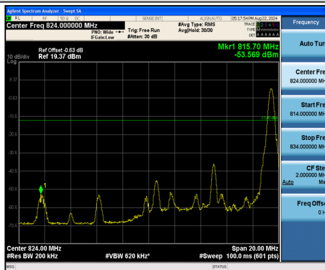
Band26-10MHz-16QAM-26840-27RB#0
