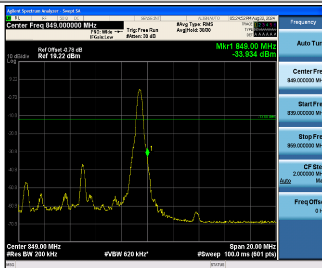
Band26-10MHz-16QAM-26990-27RB#0
