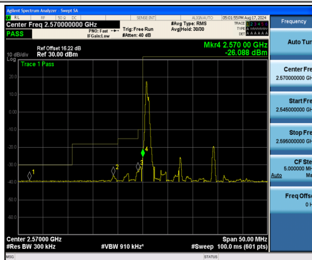
Band38-15MHz-16QAM-37825-27RB#0
