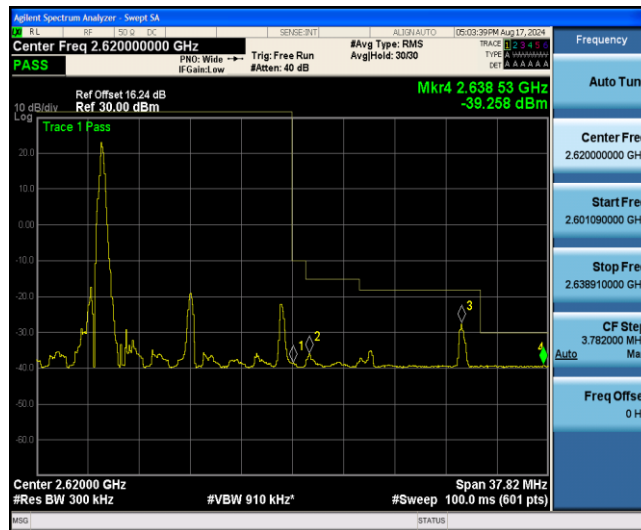
Band38-15MHz-16QAM-38175-27RB#0
