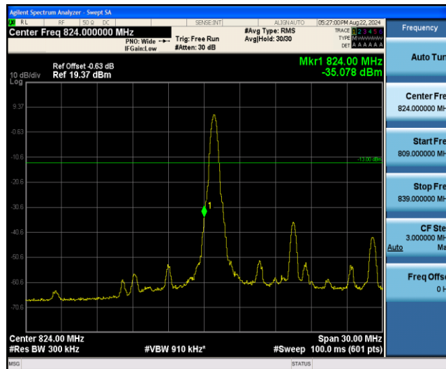
Band26-15MHz-QPSK-26865-1RB#74
