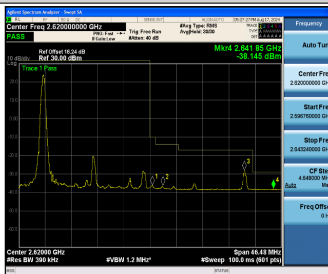
Band38-20MHz-16QAM-38150-27RB#0
