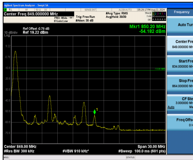
Band26-15MHz-16QAM-26965-27RB#0
