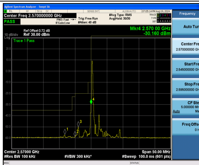
Band38-5MHz-QPSK-37775-1RB#24
