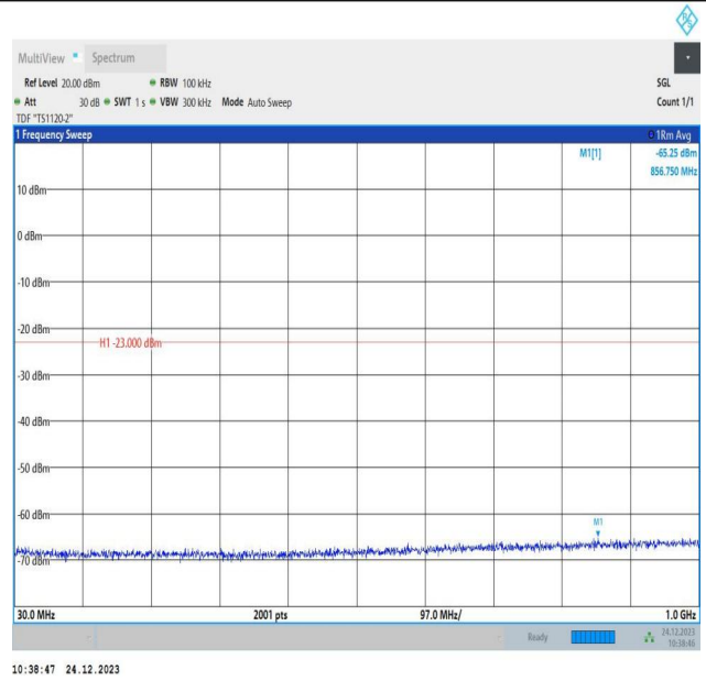
2-2-15MHz-20MHz-QPSK-QPSK-18929-19100-75RB#0-100R B#0-30~1000MHz-PASS
