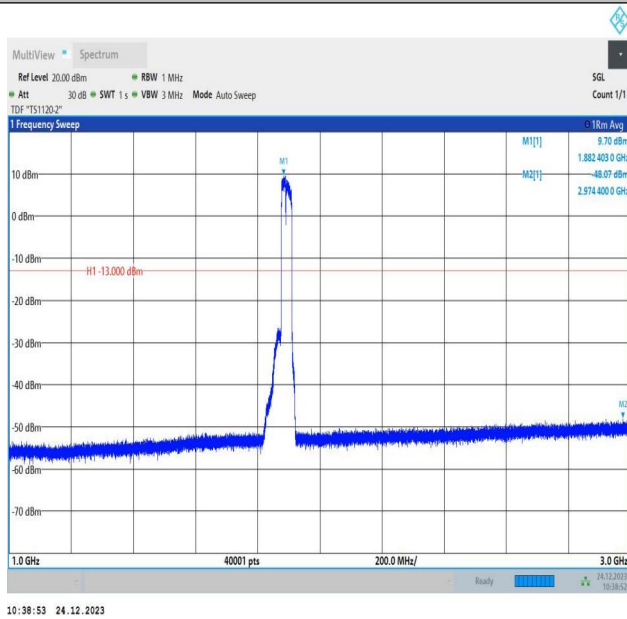
2-2-15MHz-20MHz-QPSK-QPSK-18929-19100-75RB#0-100R B#0-1000~3000MHz-PASS
