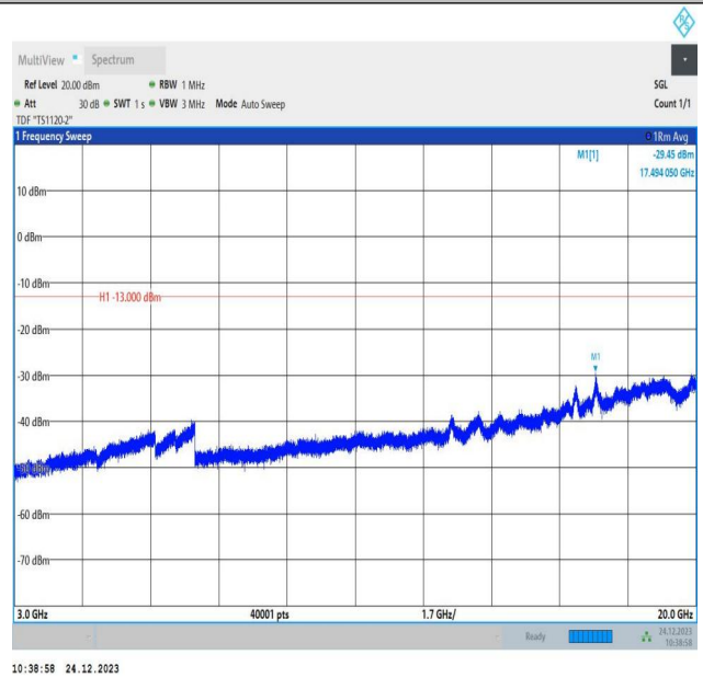
2-2-15MHz-20MHz-QPSK-QPSK-18929-19100-75RB#0-100R B#0-3000~20000MHz-PASS
