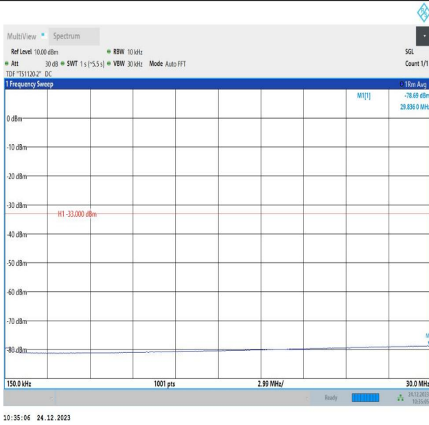
2-2-15MHz-20MHz-QPSK-QPSK-18803-18974-75RB#0-100R B#0-0.15~30MHz-PASS
