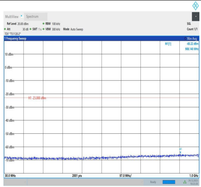
2-2-15MHz-20MHz-QPSK-QPSK-18678-18849-75RB#0-100R B#0-30~1000MHz-PASS
