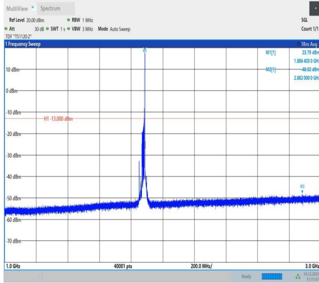
2-2-20MHz-5MHz-QPSK-QPSK-18875-18992-1RB#99-0RB#0 -1000~3000MHz-PASS
