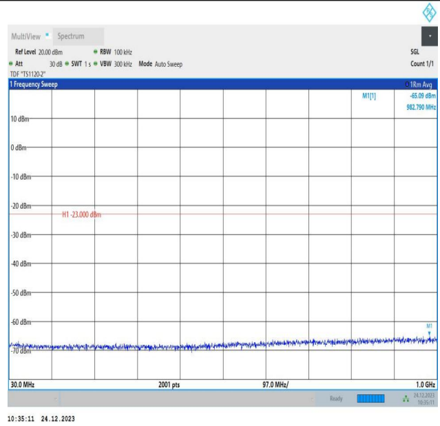
2-2-15MHz-20MHz-QPSK-QPSK-18803-18974-75RB#0-100R B#0-30~1000MHz-PASS
