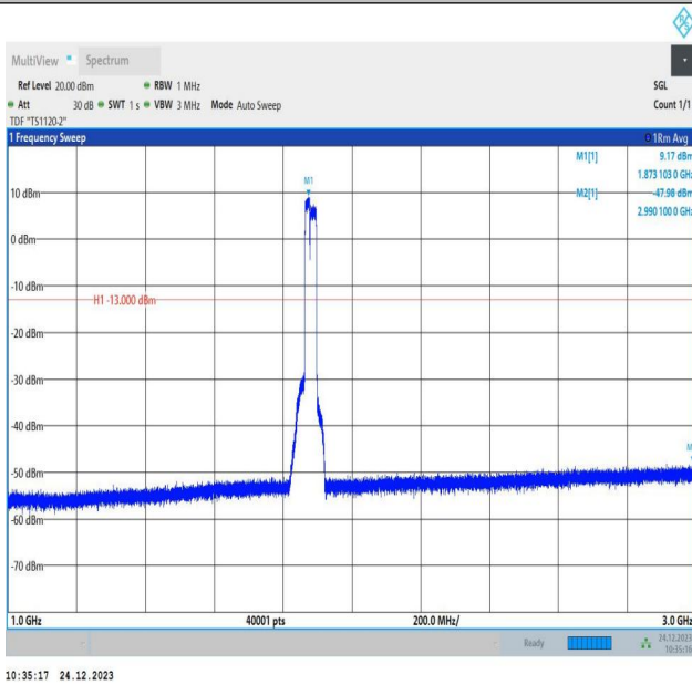
2-2-15MHz-20MHz-QPSK-QPSK-18803-18974-75RB#0-100R B#0-1000~3000MHz-PASS
