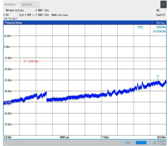
2-2-20MHz-5MHz-QPSK-QPSK-18875-18992-1RB#99-0RB#0 -3000~20000MHz-PASS
