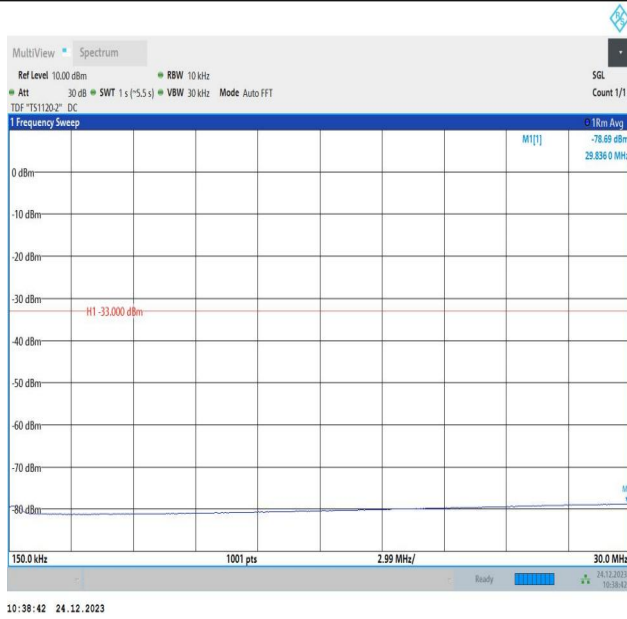
2-2-15MHz-20MHz-QPSK-QPSK-18929-19100-75RB#0-100R B#0-0.15~30MHz-PASS
