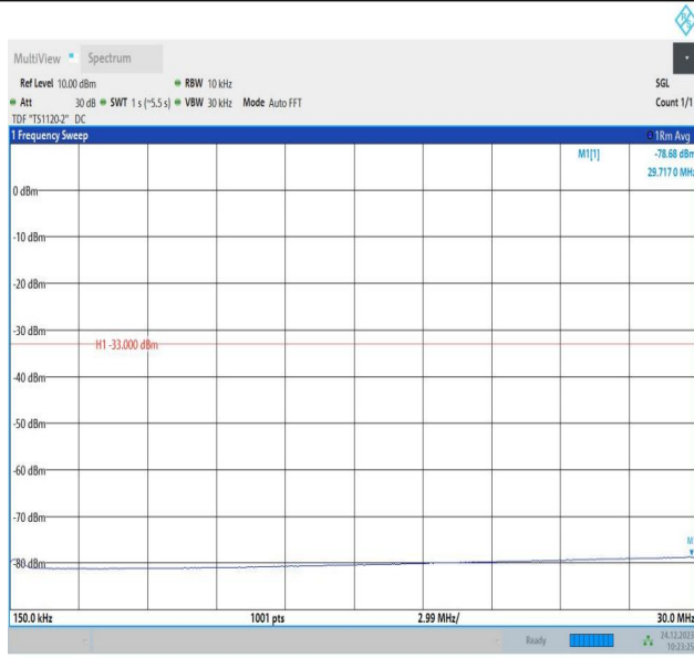
2-2-15MHz-20MHz-QPSK-QPSK-18678-18849-75RB#0-100R B#0-0.15~30MHz-PASS
