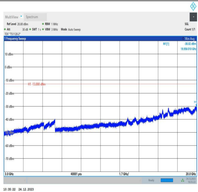
2-2-15MHz-20MHz-QPSK-QPSK-18803-18974-75RB#0-100R B#0-3000~20000MHz-PASS
