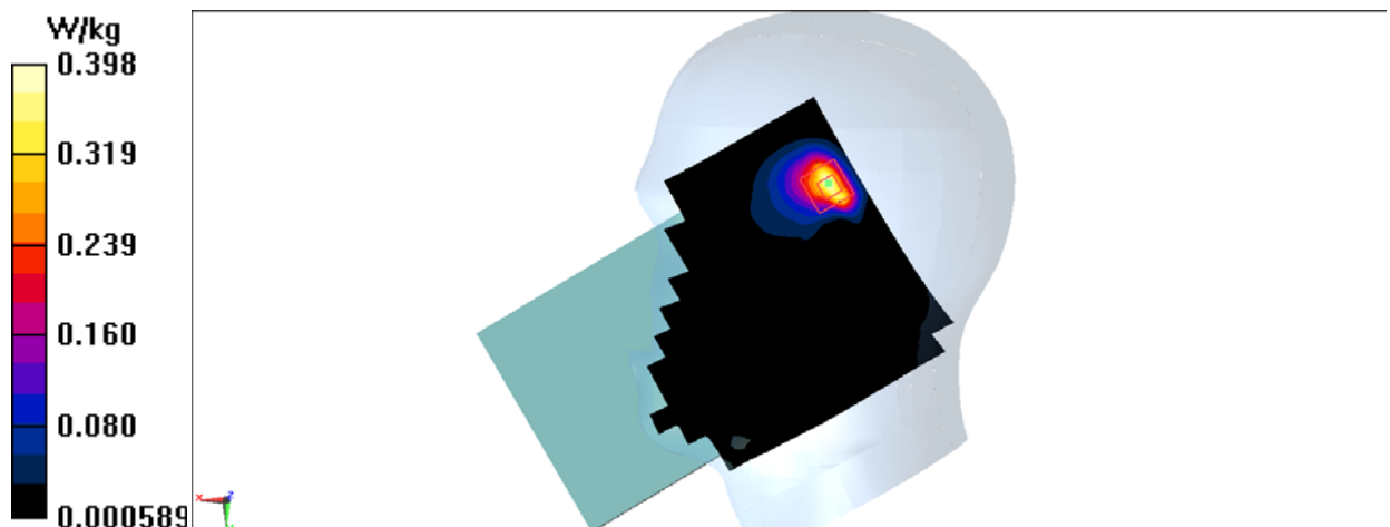
Fig.21 LTE Band 41
