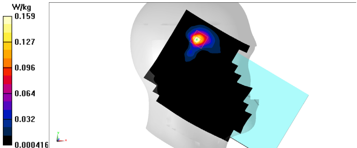
Fig.23 2450 MHz
