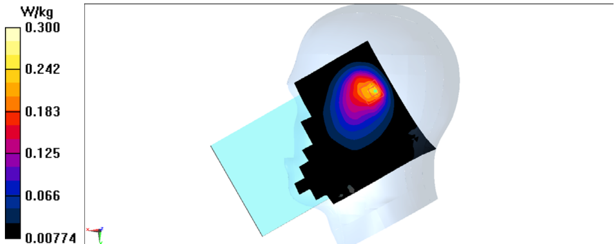
Fig.1 850MHz
