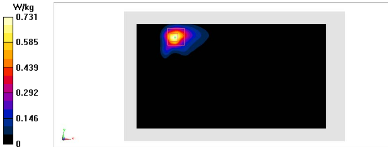
Fig.22 LTE Band 41
