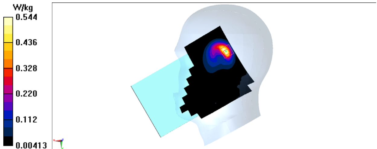
Fig.3 1900 MHz
