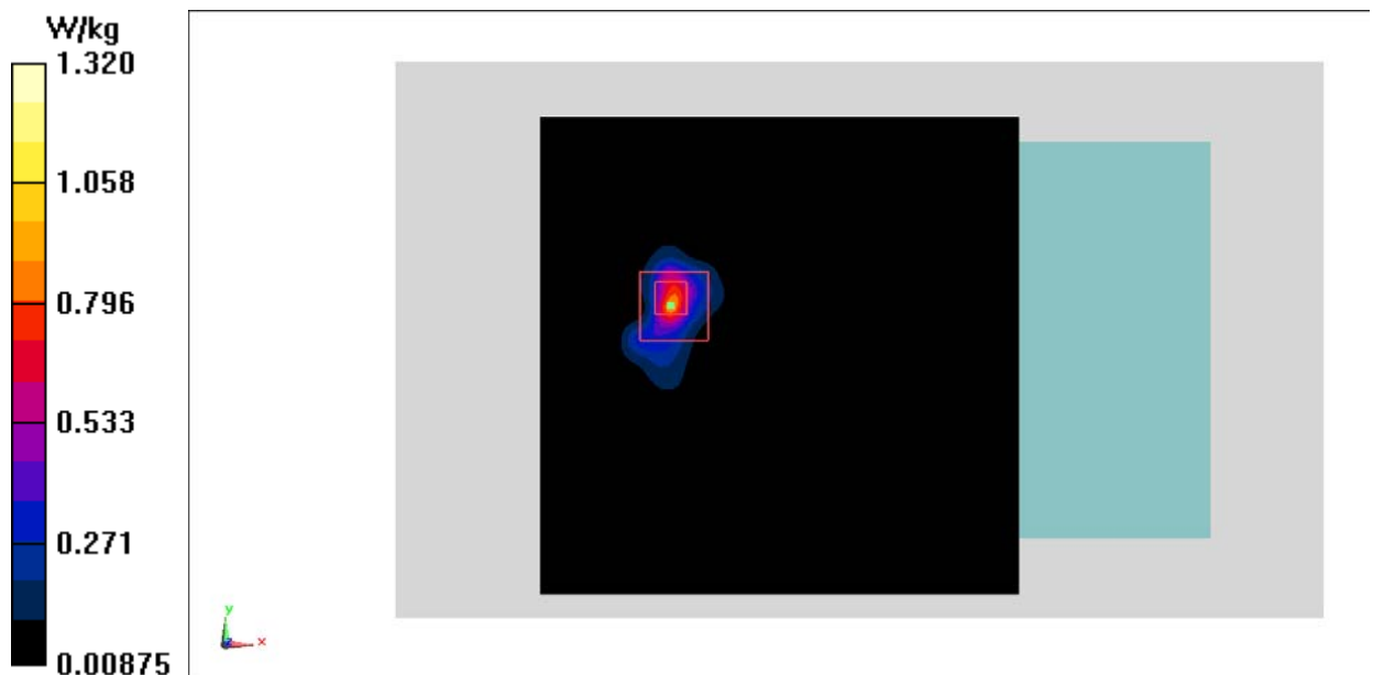
Fig.26 5GHz
