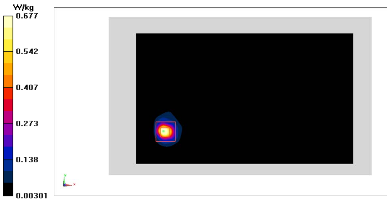
Fig.24 2450 MHz
