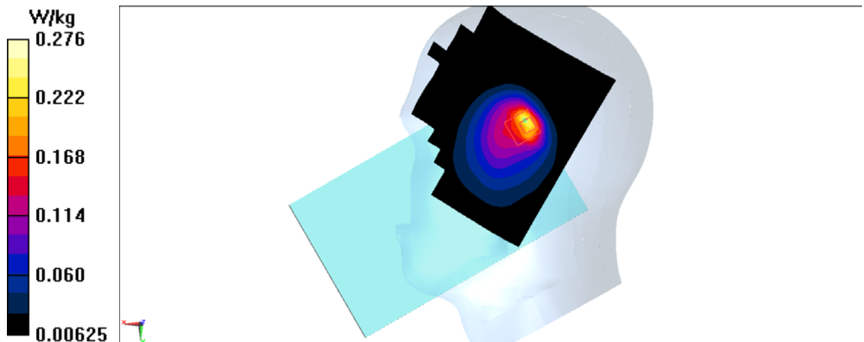
Fig.19 LTE Band12
