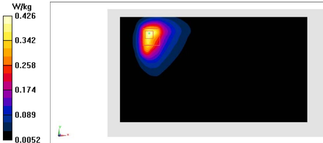
Fig.20 LTE Band12
