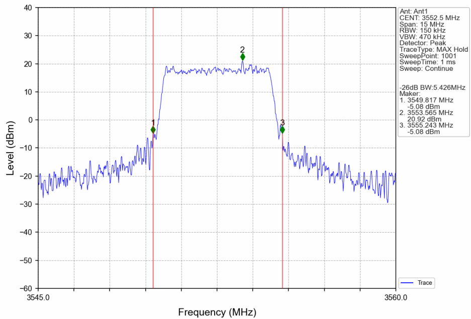
Band42c 5MHz 16QAM LCH 3552.5MHz RB 25 0 NTNV
