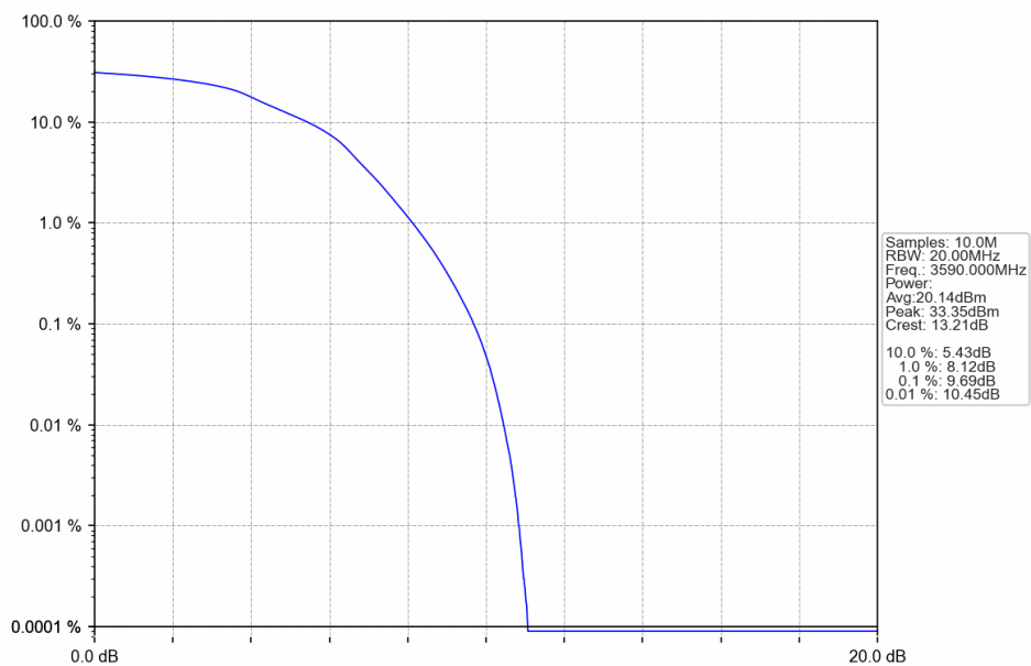
Band42c 20MHz 16QAM HCH 3590MHz RB 100 0 NTNV
