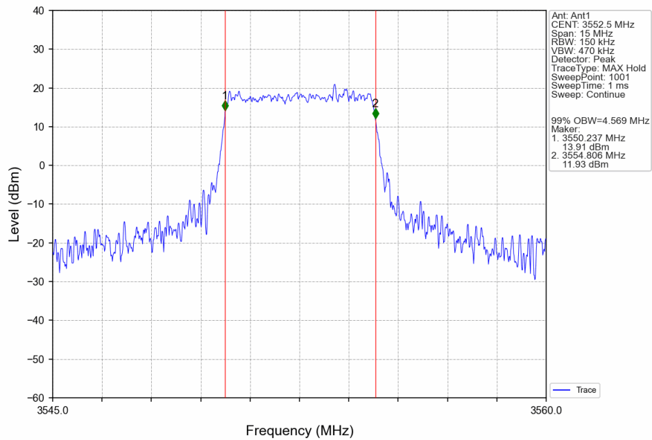
Band42c 5MHz 16QAM LCH 3552.5MHz RB 25 0 NTN
