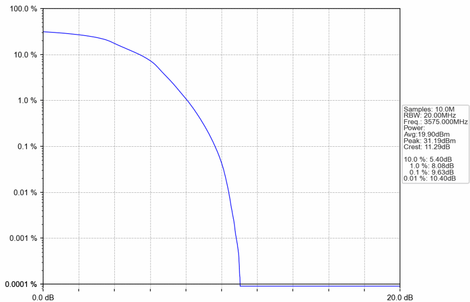
Band42c 20MHz 16QAM MCH 3575MHz RB 100 0 NTNV
