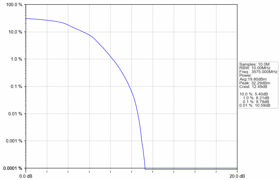
Band42c 10MHz 16QAM MCH 3575MHz RB 50 0 NTNV
