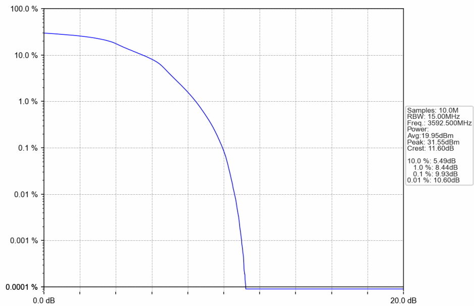
Band42c 15MHz 16QAM HCH 3592.5MHz RB 75 0 NTNV
