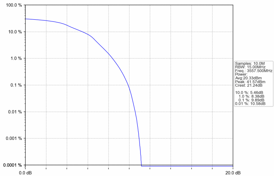
Band42c 15MHz 16QAM LCH 3557.5MHz RB 75 0 NTV
