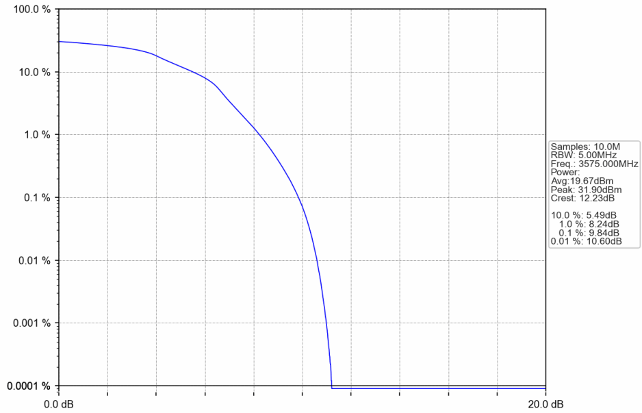
Band42c 5MHz 16QAM MCH 3575MHz RB 25 0 NTNV
