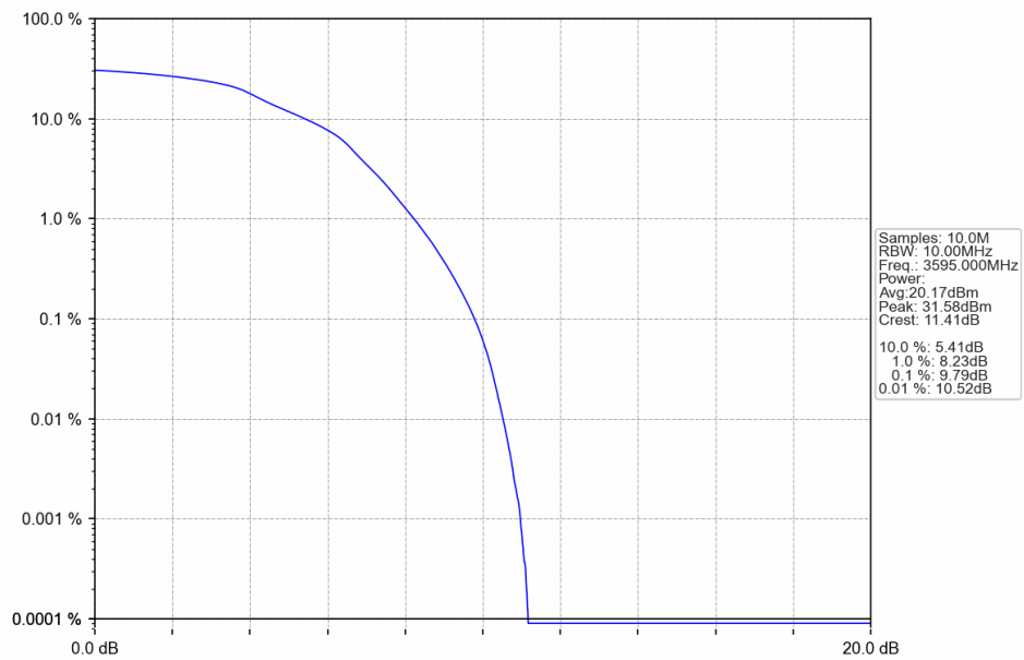
Band42c 10MHz 16QAM HCH 3595MHz RB 50 0 NTNV
