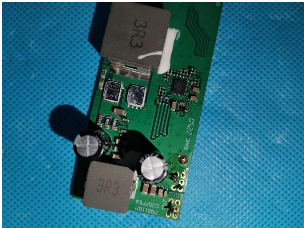
INTERNAL VIEW-13 OF EUT
