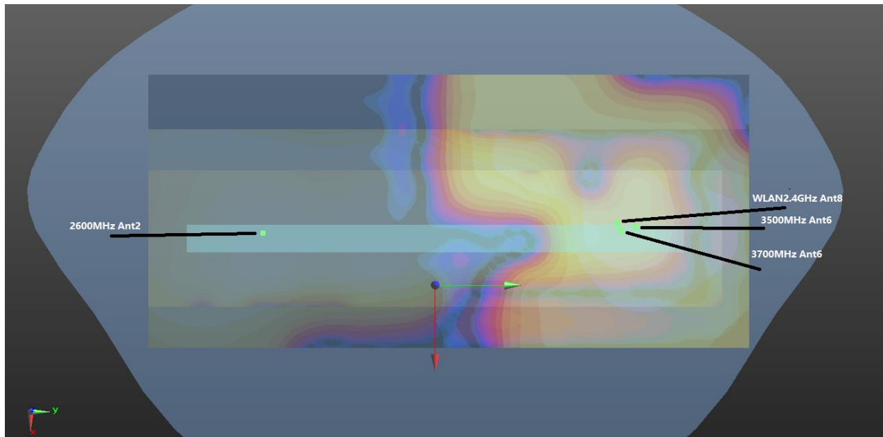
WWAN+NR+WLAN2.4GHz_Left Side 10mm
