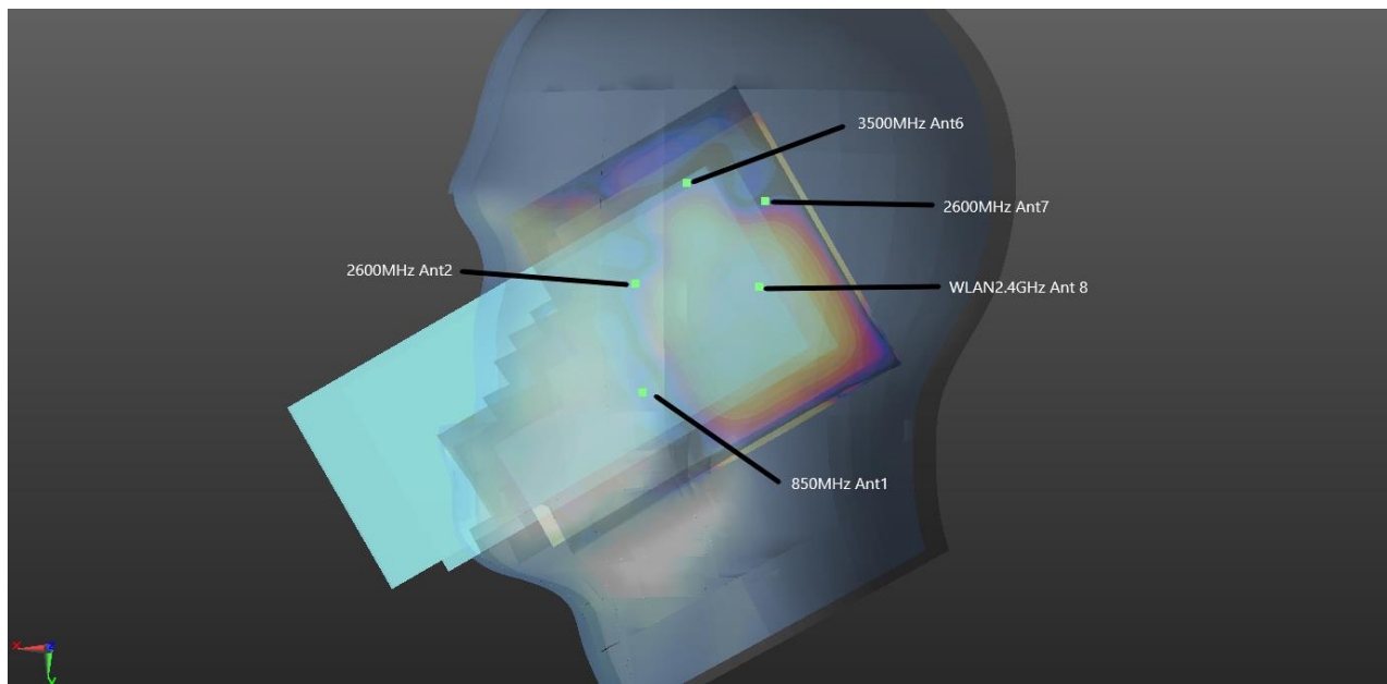
WWAN+NR+WLAN2.4GHz_Right Cheek 0mm
