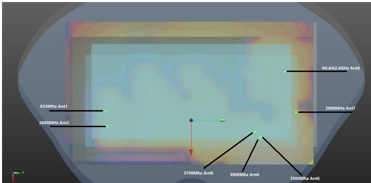
WWAN+NR+WLAN2.4GHz_Back 10mm
