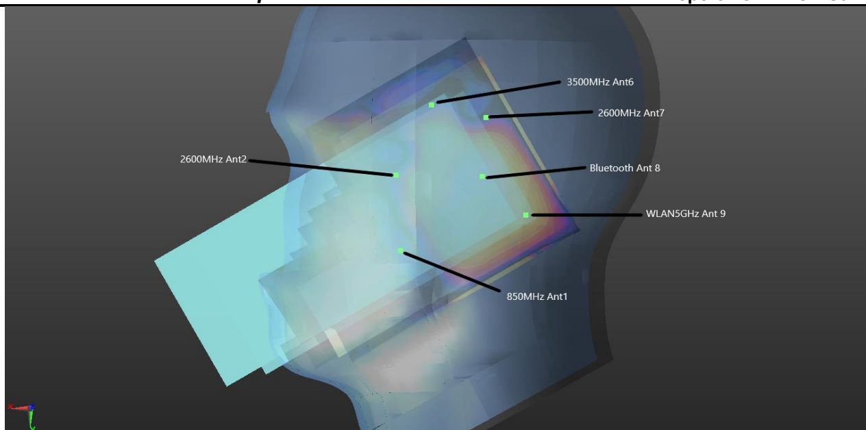
WWAN+NR+WLAN5GHz+BT_Right Cheek 0mm
