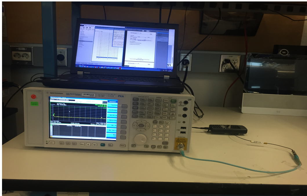
Title: RF Conducted Test Setup
