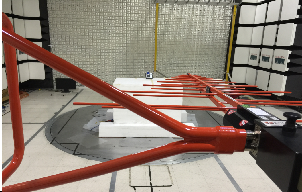
Title: Radiated Emissions Below 1 GHz
