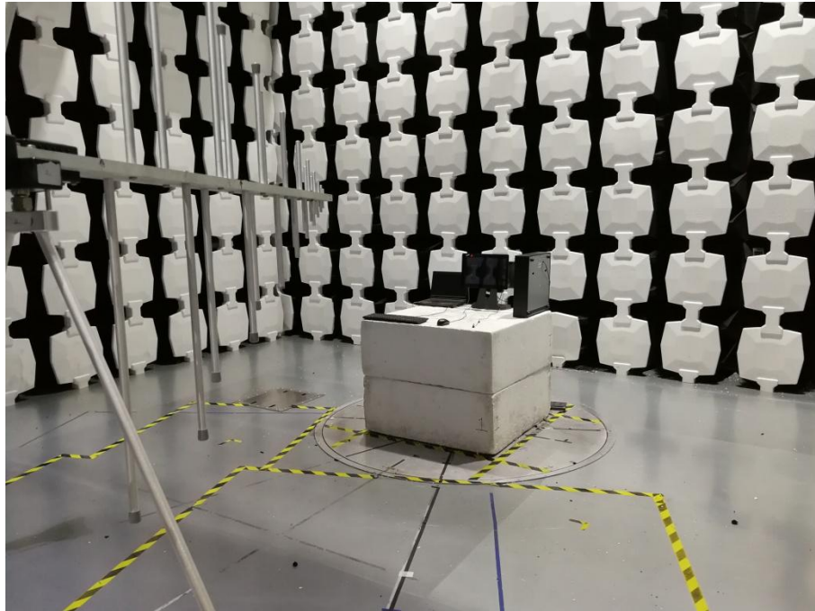
Description: Front view of Radiated Emission Test Setup
