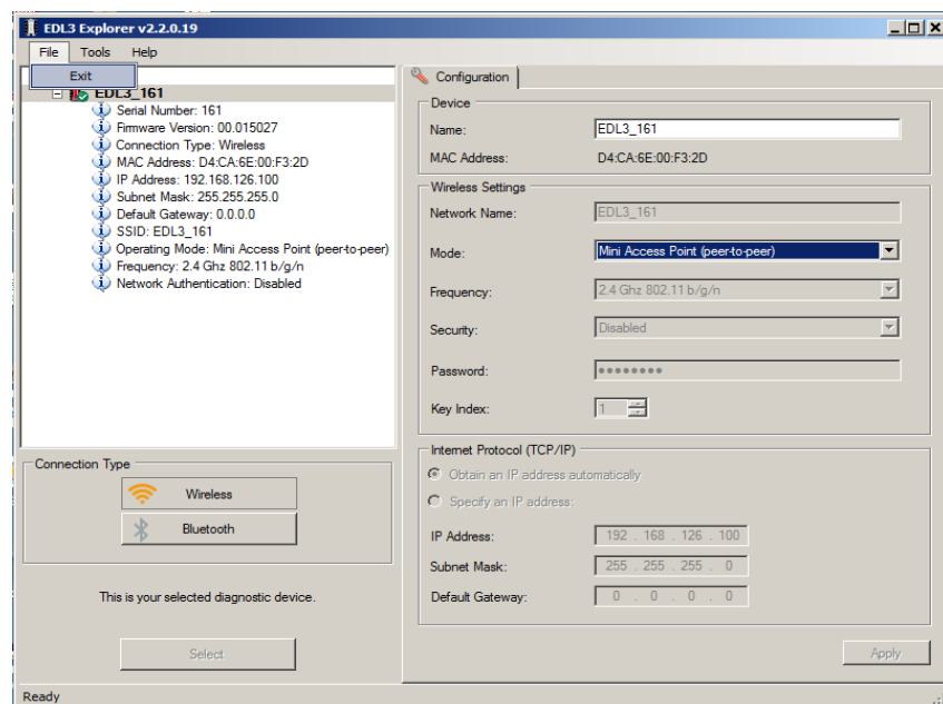
Figure 3.22 Exit Selected
