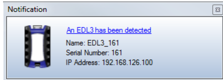
Figure 3.25 Notification Box
