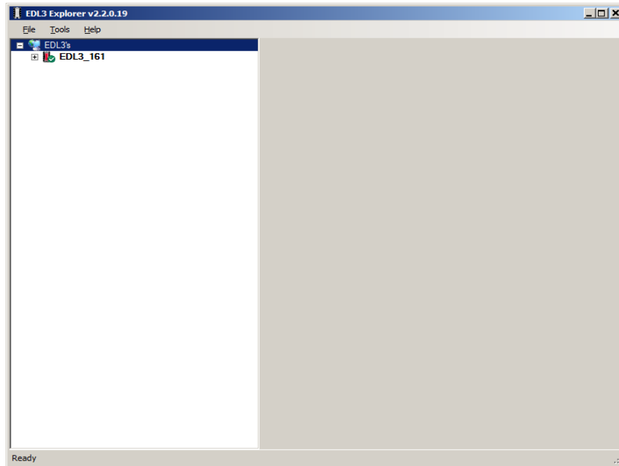
Figure 3.19 EDL3 Explorer
