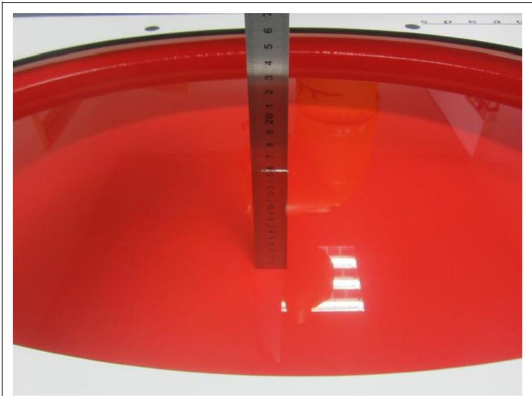
Liquid depth in the ELI Phantom
