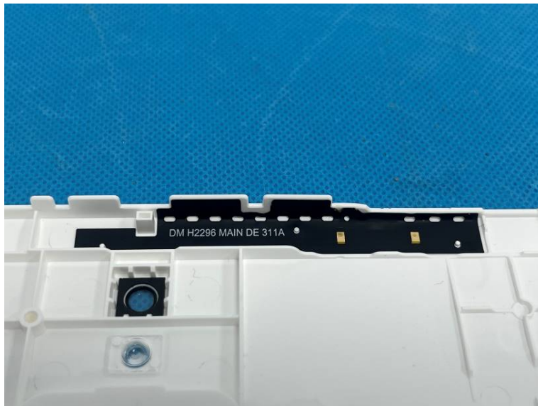
GSM/WCDMA/LTE Main Antenna
