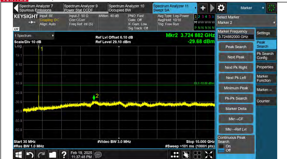
Band26-10MHz-QPSK-26840-1RB#0-Range1:30~10000MHz
