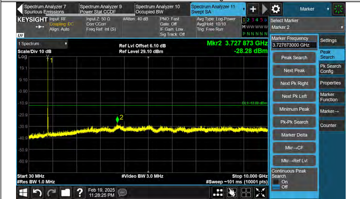
Band26-3MHz-QPSK-26915-1RB#0-Range1:30~10000MHz
