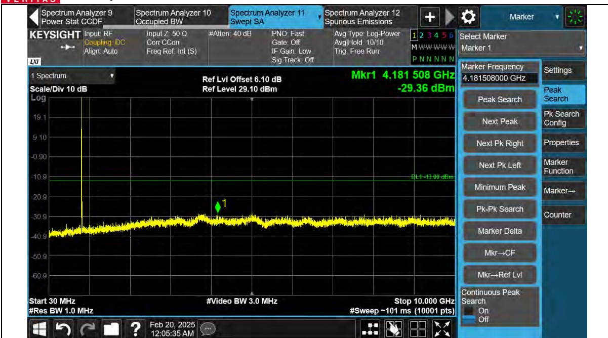
Band26-10MHz-QPSK-26990-1RB#0-Range1:30~10000MHz
