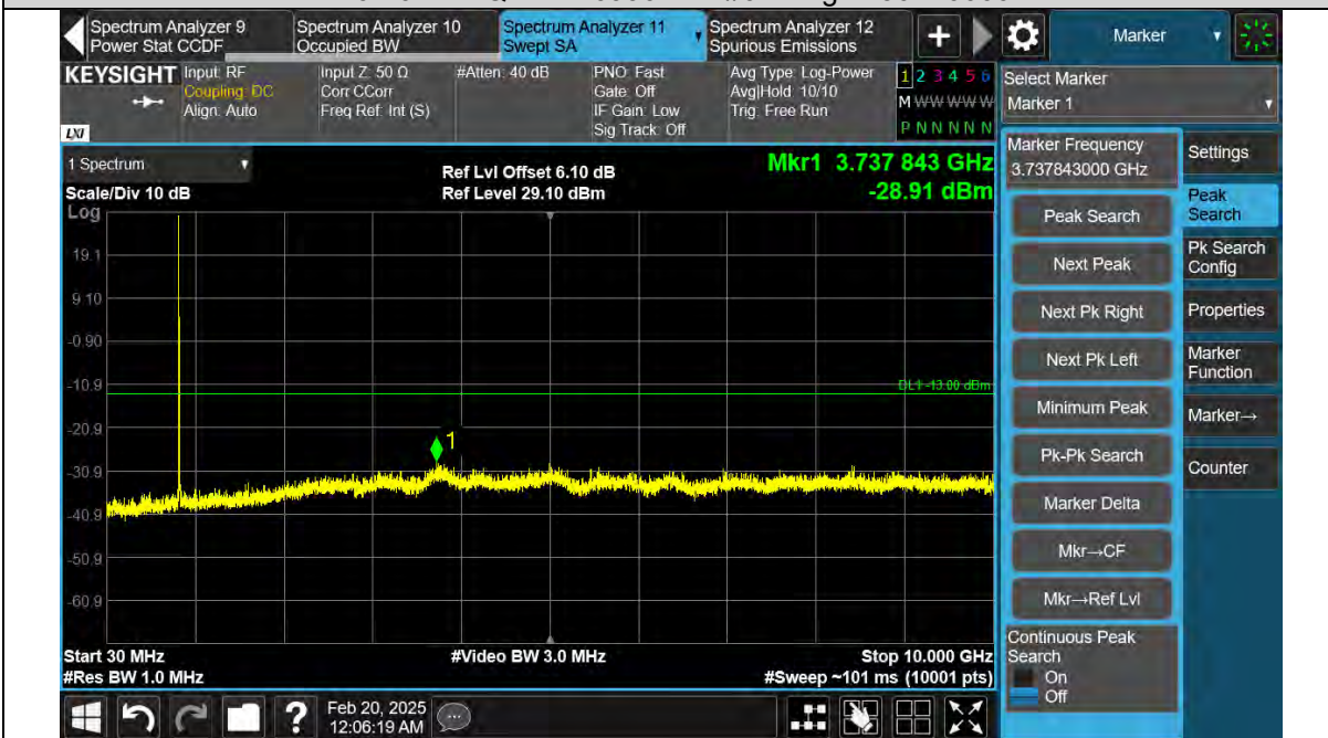
Band26-15MHz-QPSK-26865-1RB#0-Range1:30~10000MHz
