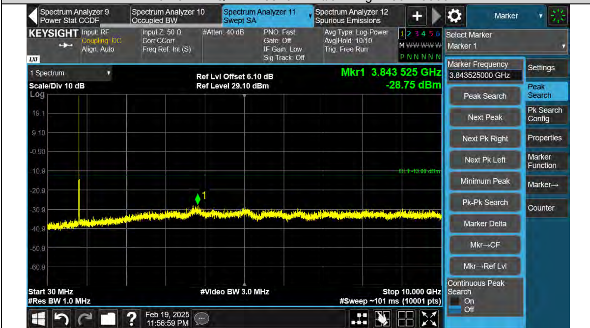
Band26-10MHz-QPSK-26915-1RB#0-Range1:30~10000MHz
