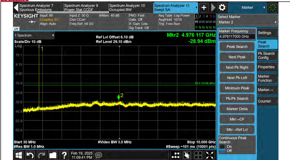
Band26-3MHz-QPSK-26805-1RB#0-Range1:30~10000MHz
