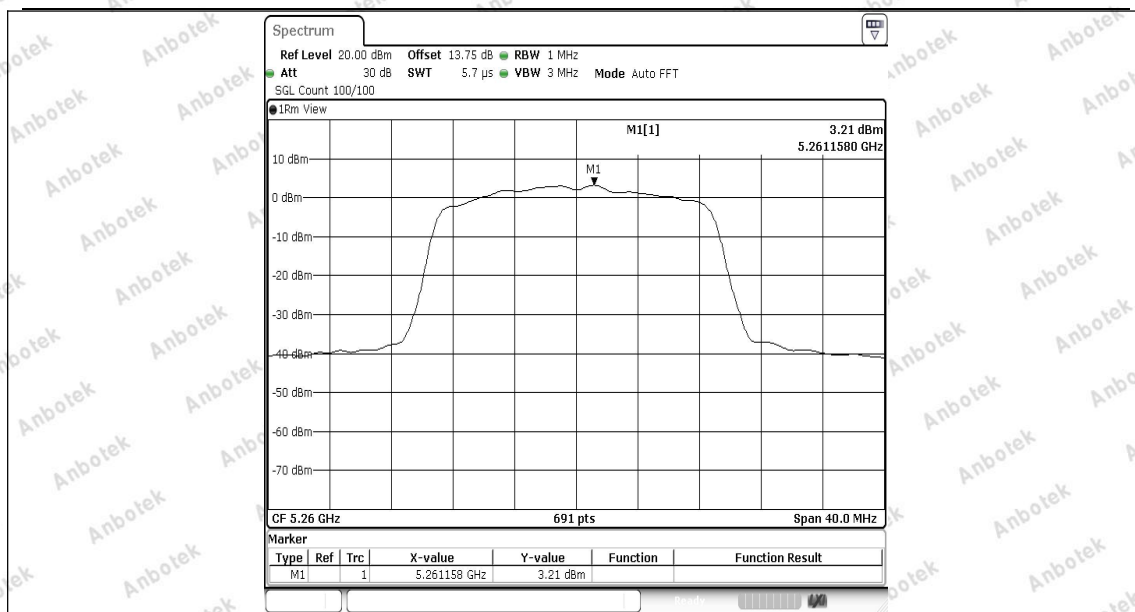
11AC20SISO-Ant1-5260-PASS
