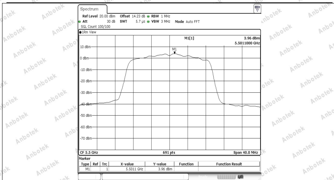
11N20SISO-Ant1-5500-PASS
