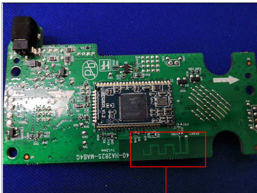
BT Antenna
