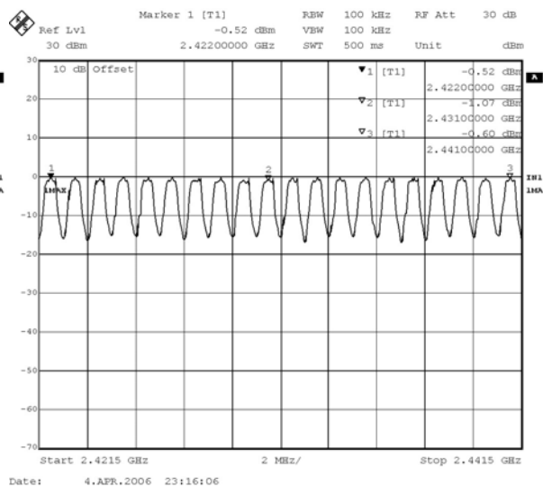
2422-2441MHz
