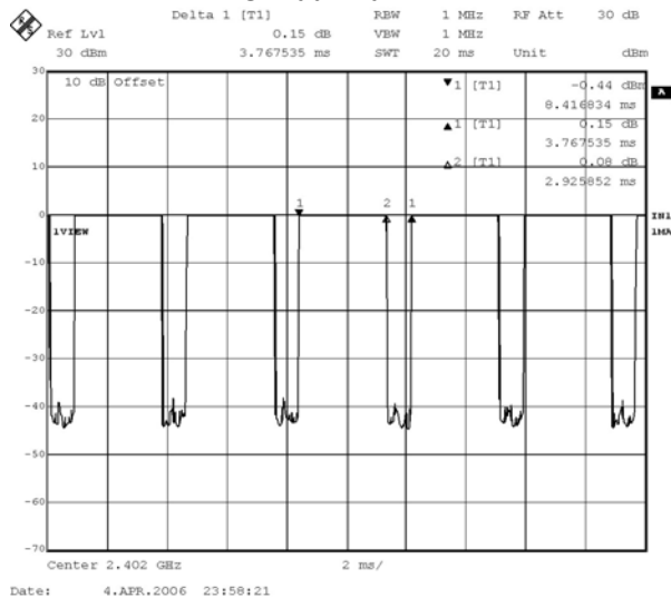
CH 00 2402MHz
