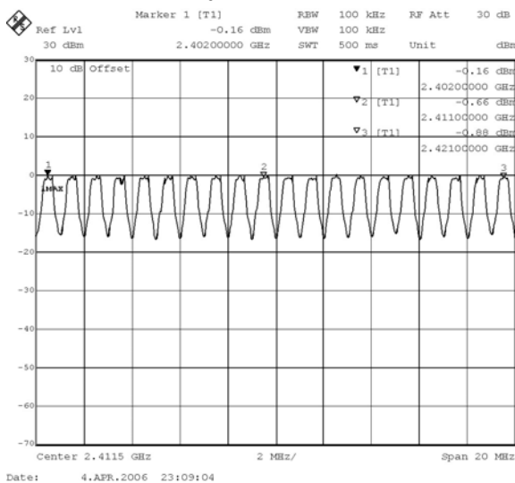
2402-2421MHz
