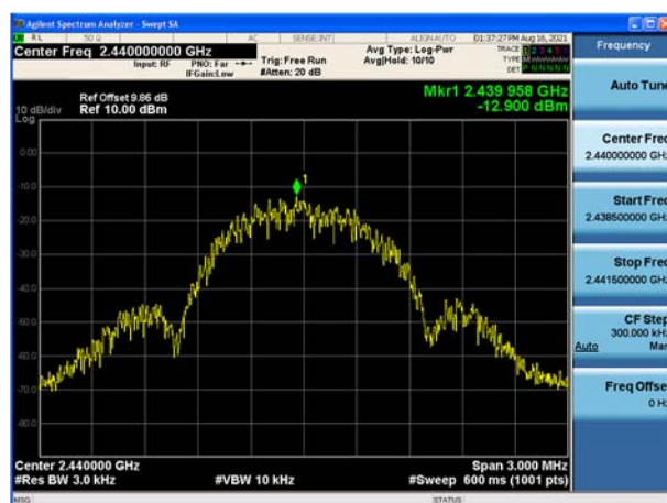
Modulation: 1Mbps 2440MHz
