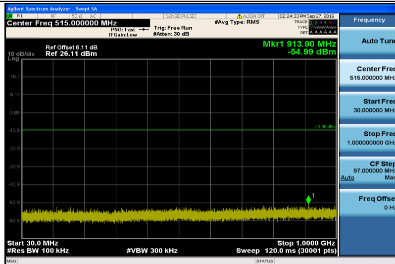
Band4-3MHz-16QAM-19965-1RB#0-30~1000MHz
