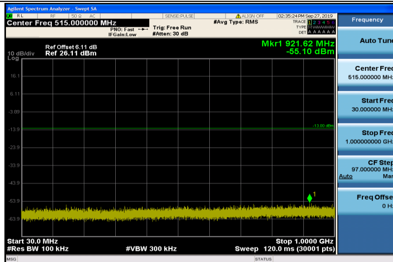
Band4-5MHz-16QAM-19975-1RB#0-30~1000MHz
