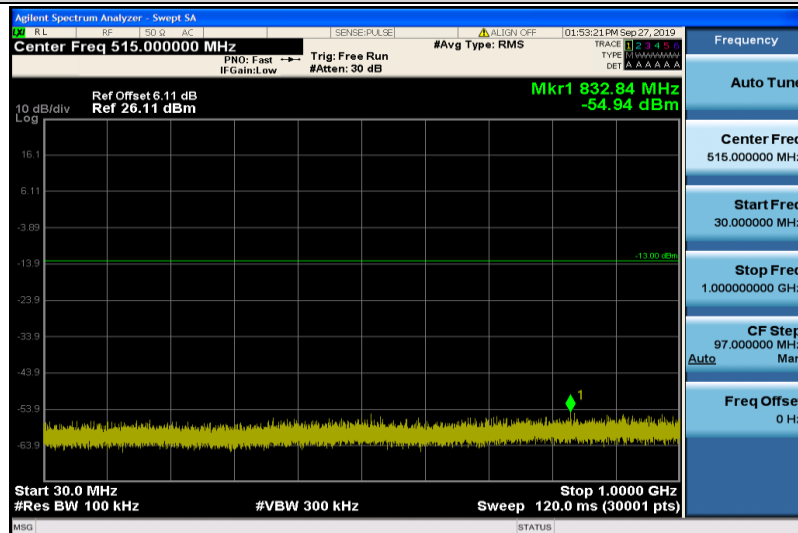
Band2-10MHz-16QAM-18650-1RB#0-30~1000MHz
