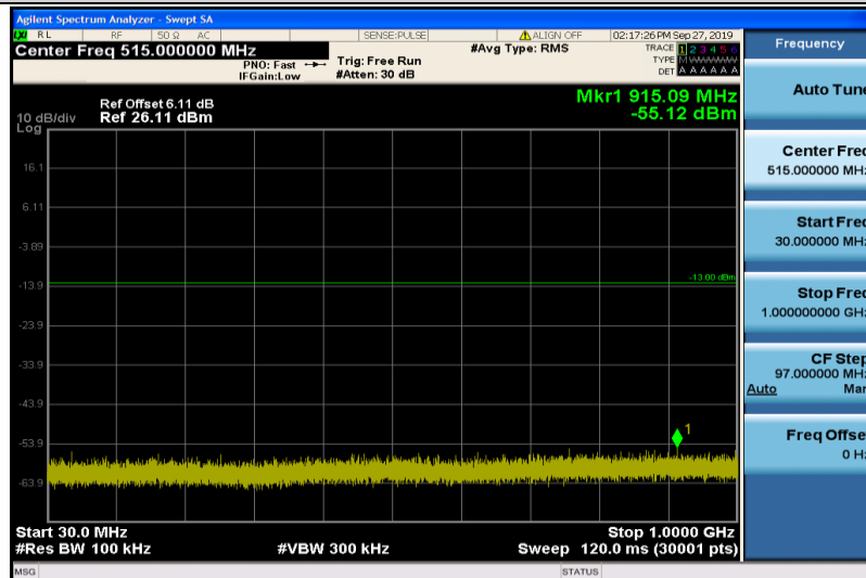
Band4-1.4MHz-16QAM-19957-1RB#0-30~1000MHz
