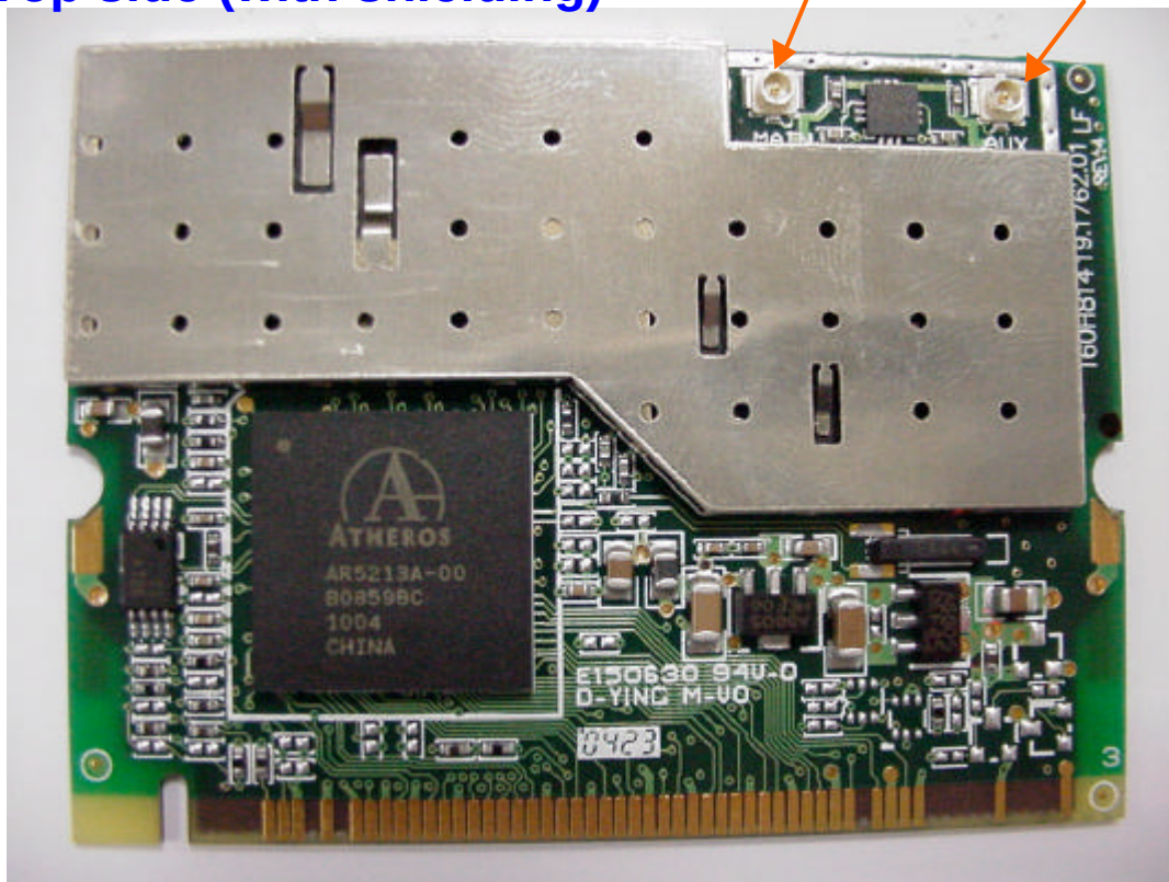
Top side (with shielding)
