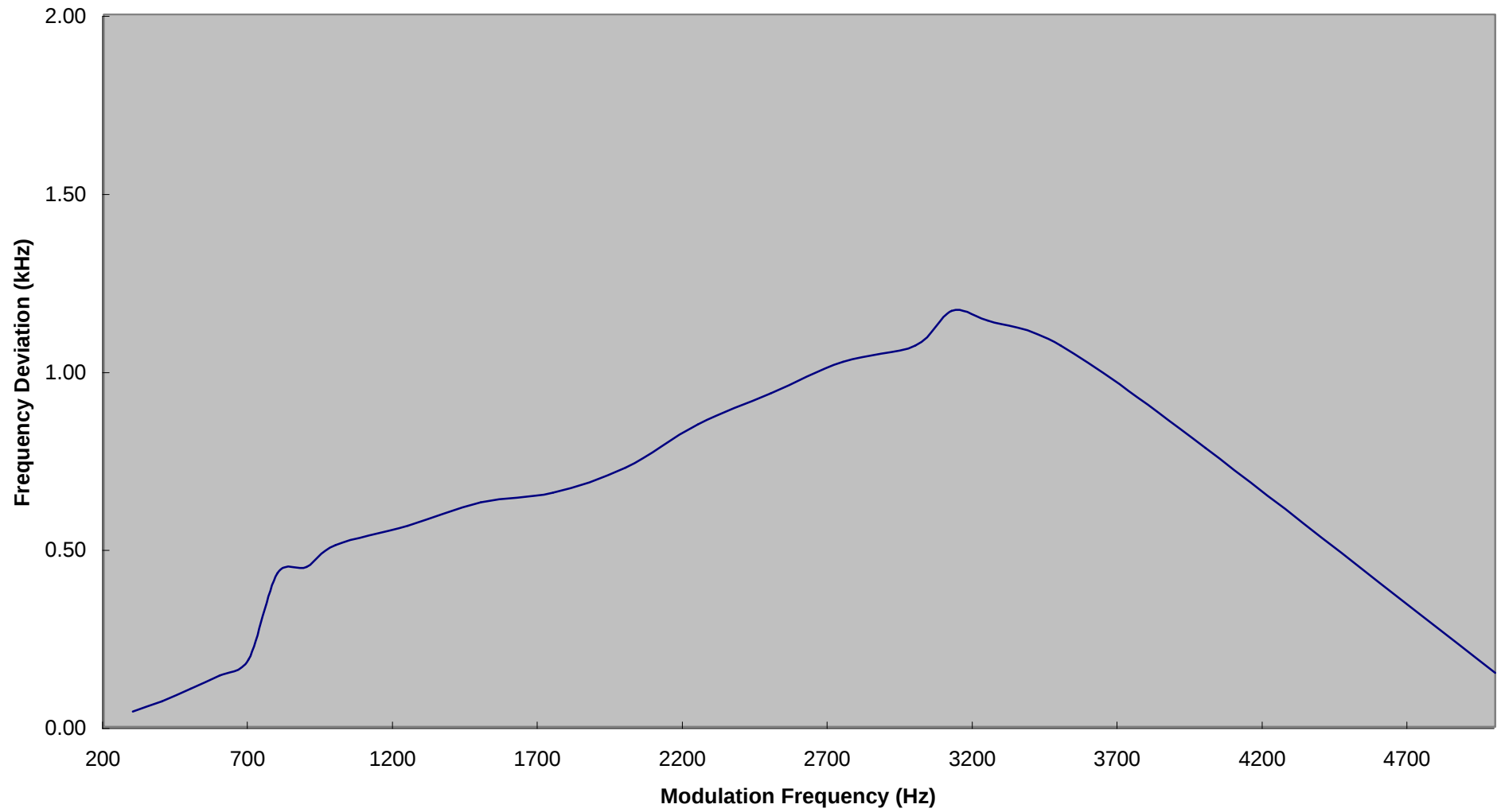
Modulation Frequency Response (T5950)
