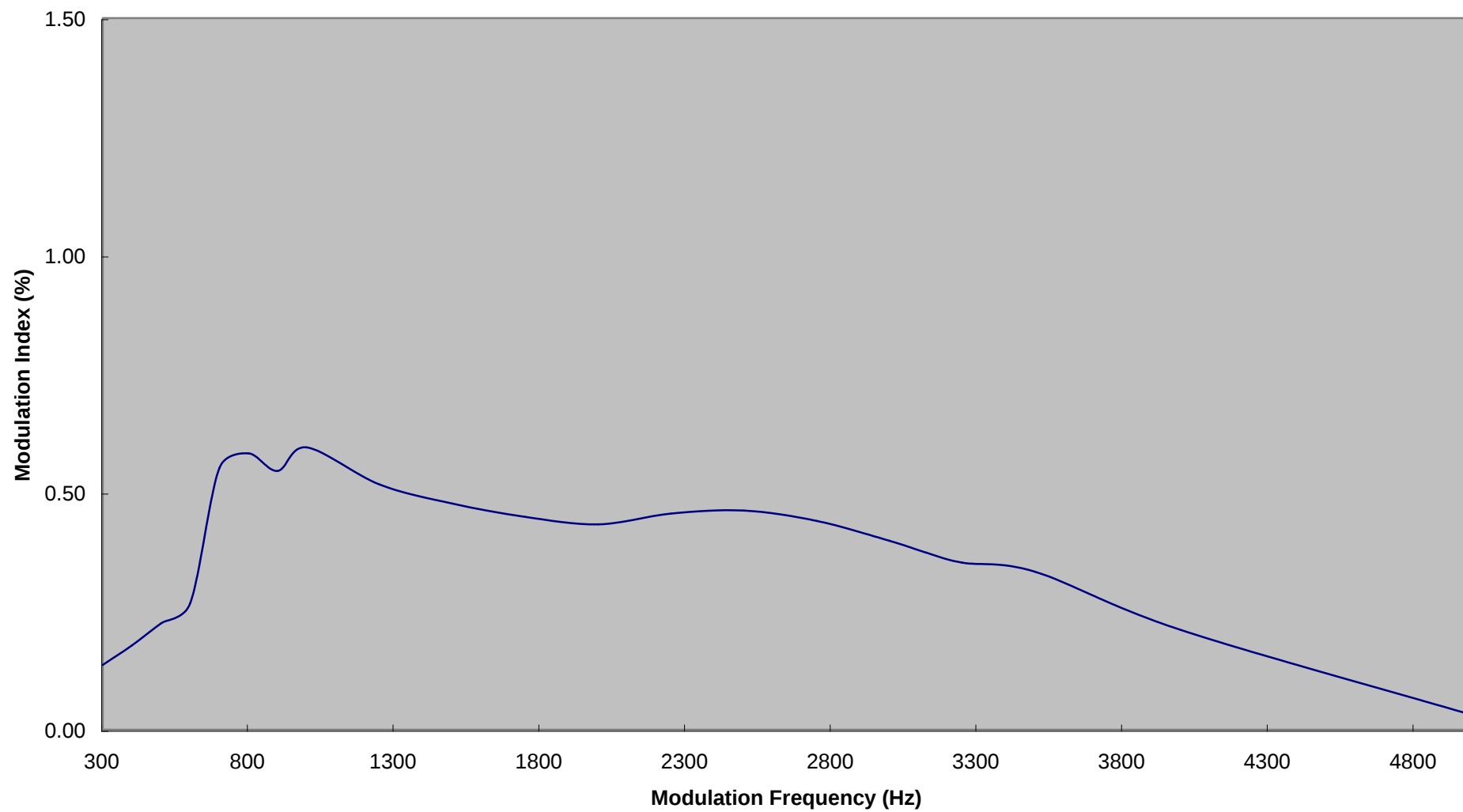
Modulation Frequency Response (T5900)
