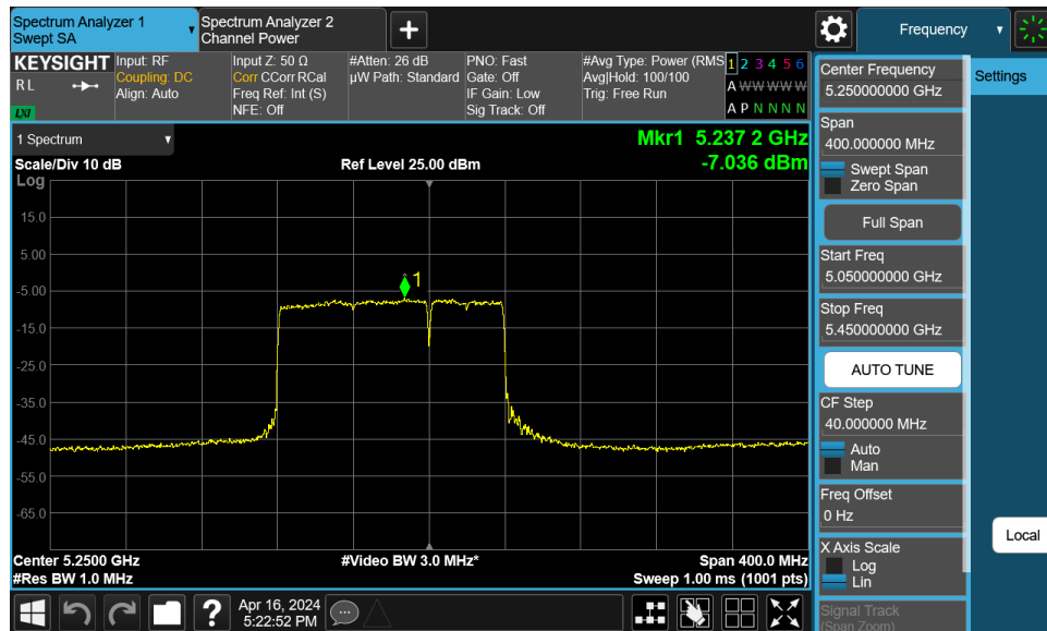
Plot 7-166. Power Spectral Density Plot MIMO ANT1 (160MHz BW 802.11be (UNII Band 1/2A) – Ch. 50)
