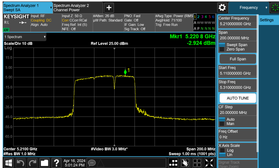
Plot 7-165. Power Spectral Density Plot MIMO ANT1 (80MHz BW 802.11be (UNII Band 1) – Ch. 42)
