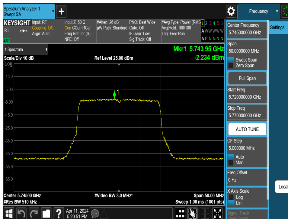
Plot 7-151. Power Spectral Density Plot MIMO ANT2 (20MHz BW 802.11ax/be (UNII Band 3) – Ch. 149)
