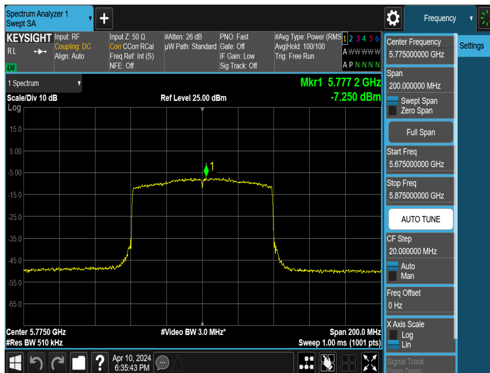
Plot 7-114. Power Spectral Density Plot MIMO ANT1 (80MHz BW 802.11ax/be (UNII Band 3) – Ch. 155)
