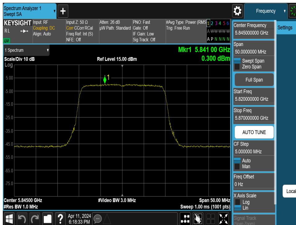
Plot 7-158. Power Spectral Density Plot MIMO ANT2 (20MHz BW 802.11ax/be (UNII Band 3/4) – Ch. 169)
