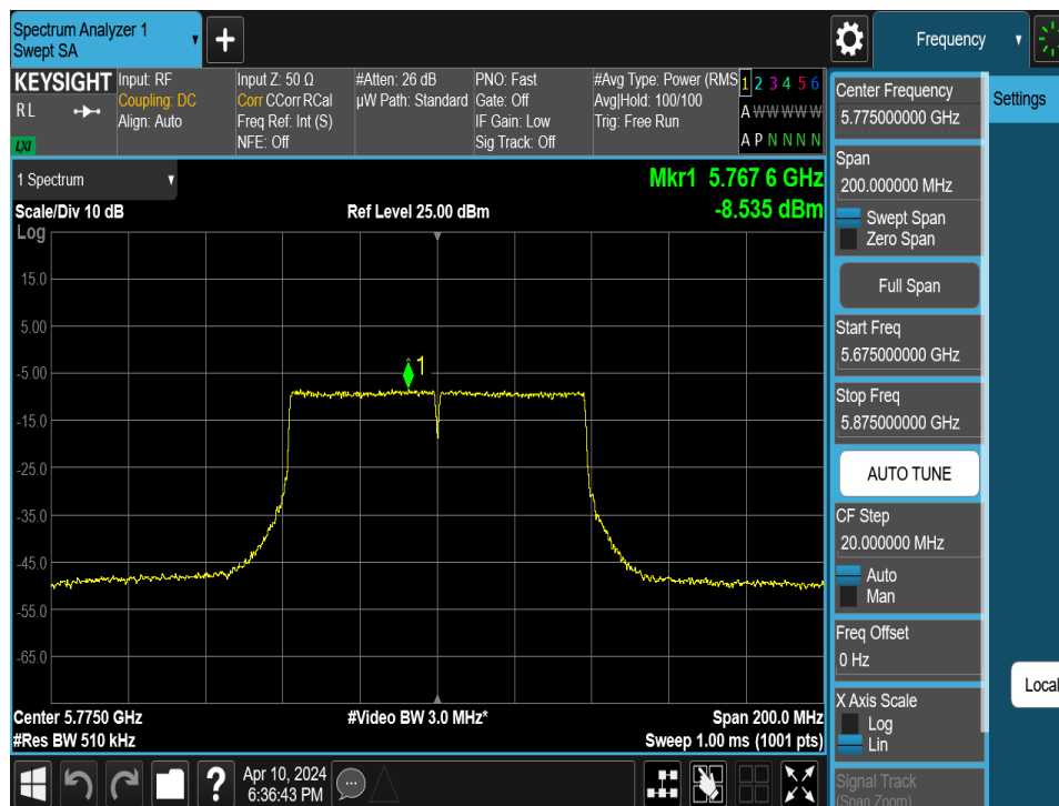
Plot 7-113. Power Spectral Density Plot MIMO ANT1 (80MHz BW 802.11ac (UNII Band 3) – Ch. 155)
