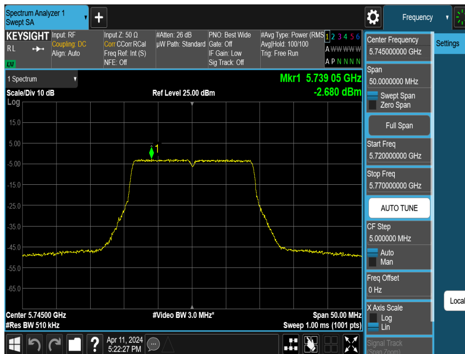
Plot 7-150. Power Spectral Density Plot MIMO ANT2 (20MHz BW 802.11n (UNII Band 3) – Ch. 149)
