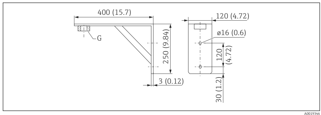
37 Dimensions of angle bracket, engineering unit: mm (in)
