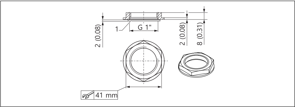
28 Dimensions of counter nut for process connection rear side, engineering unit: mm (in)
