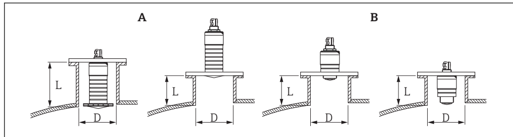
10 FMR20 nozzle installation
