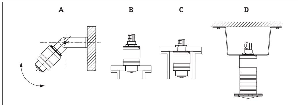
9 Wall, ceiling or nozzle installation
