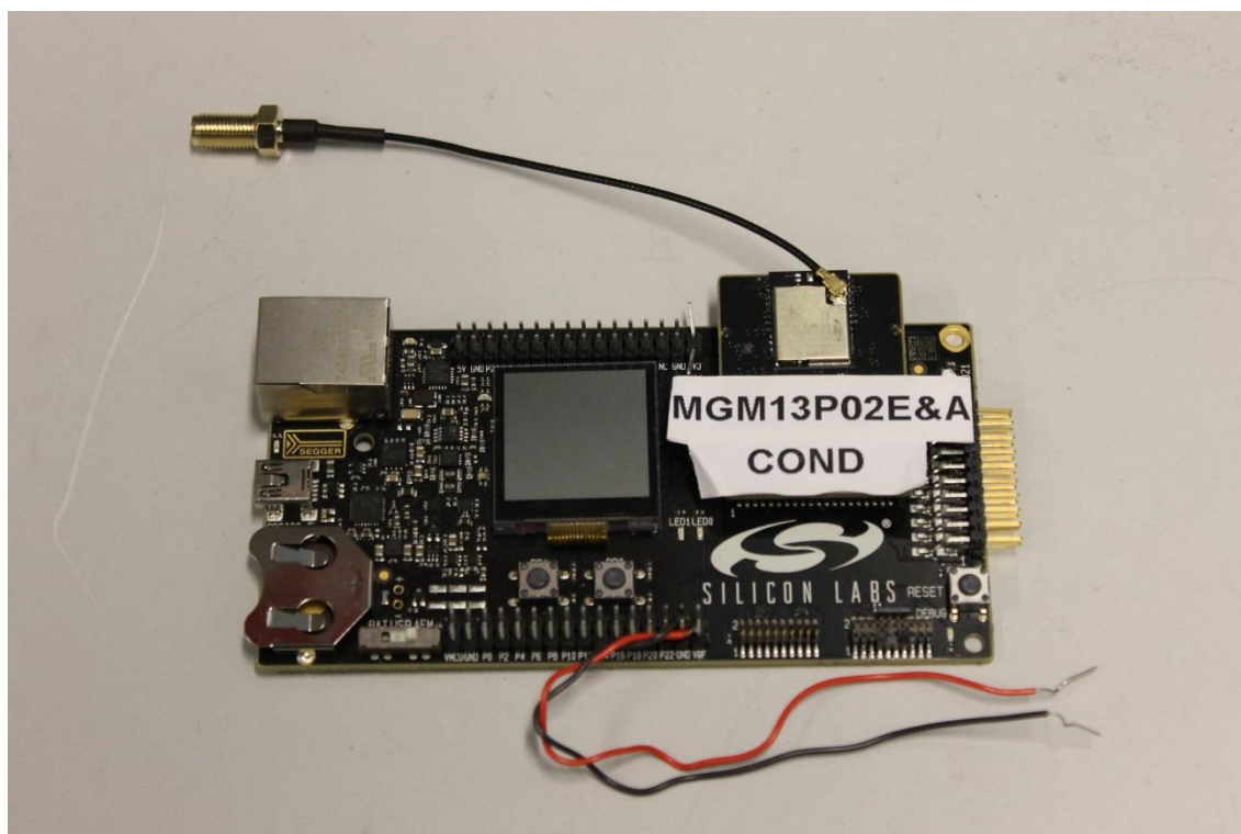
Photograph 1. The equipment under test (EUT) and supportive board
