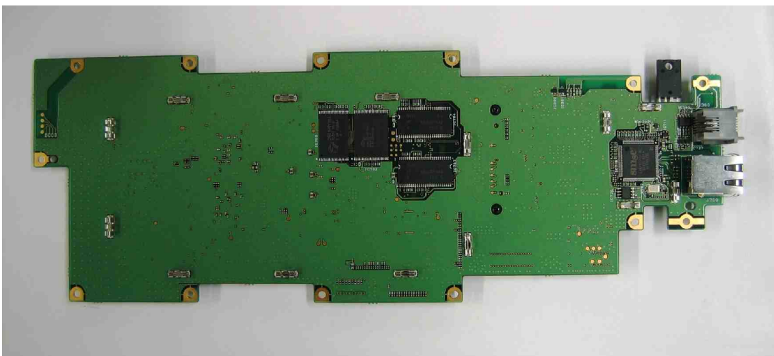
Control2 Foil Side View
