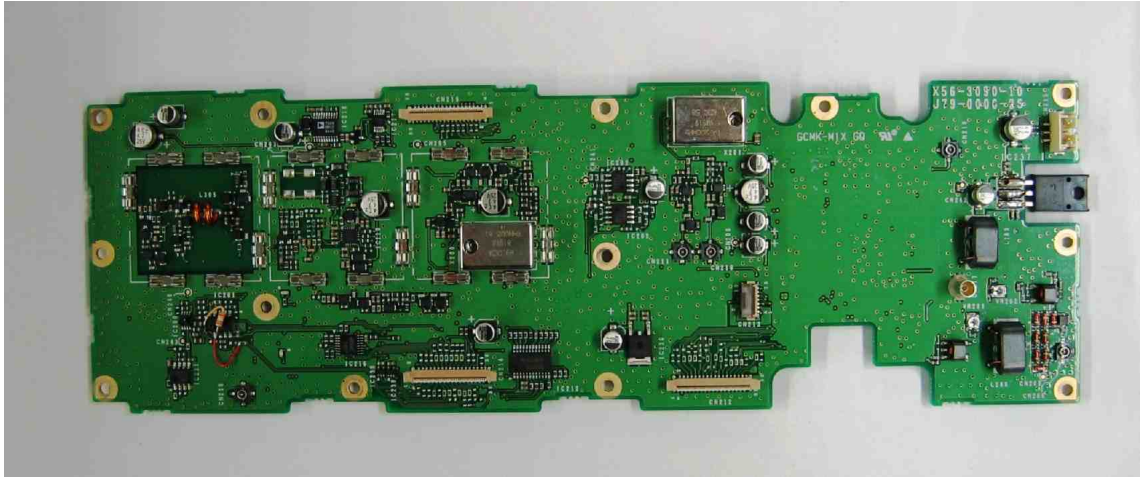
TX Component Side View
