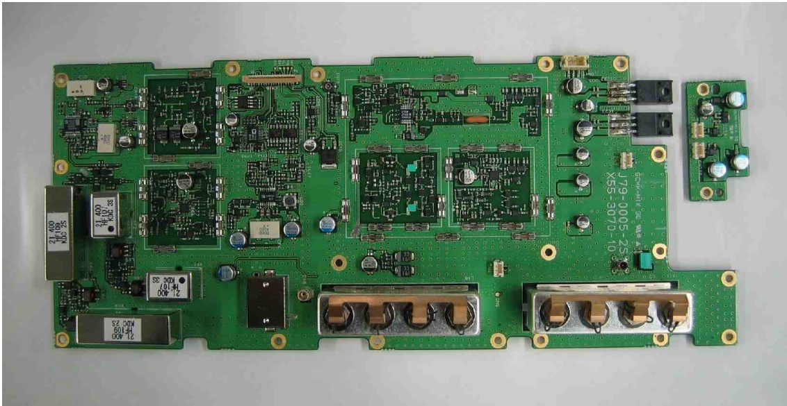
RX Component Side View
