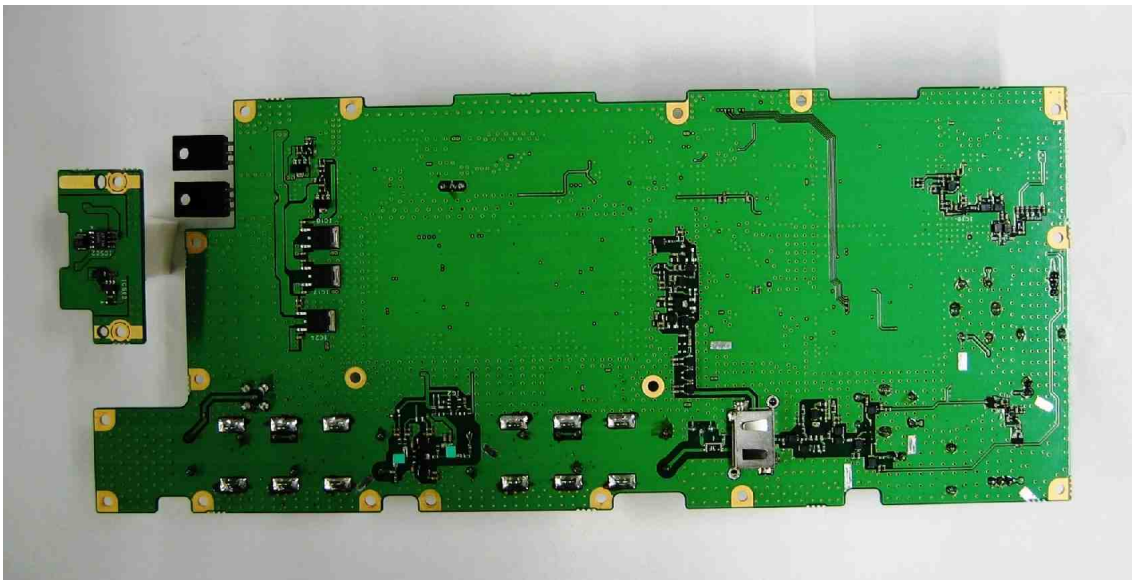
RX Foil Side View
