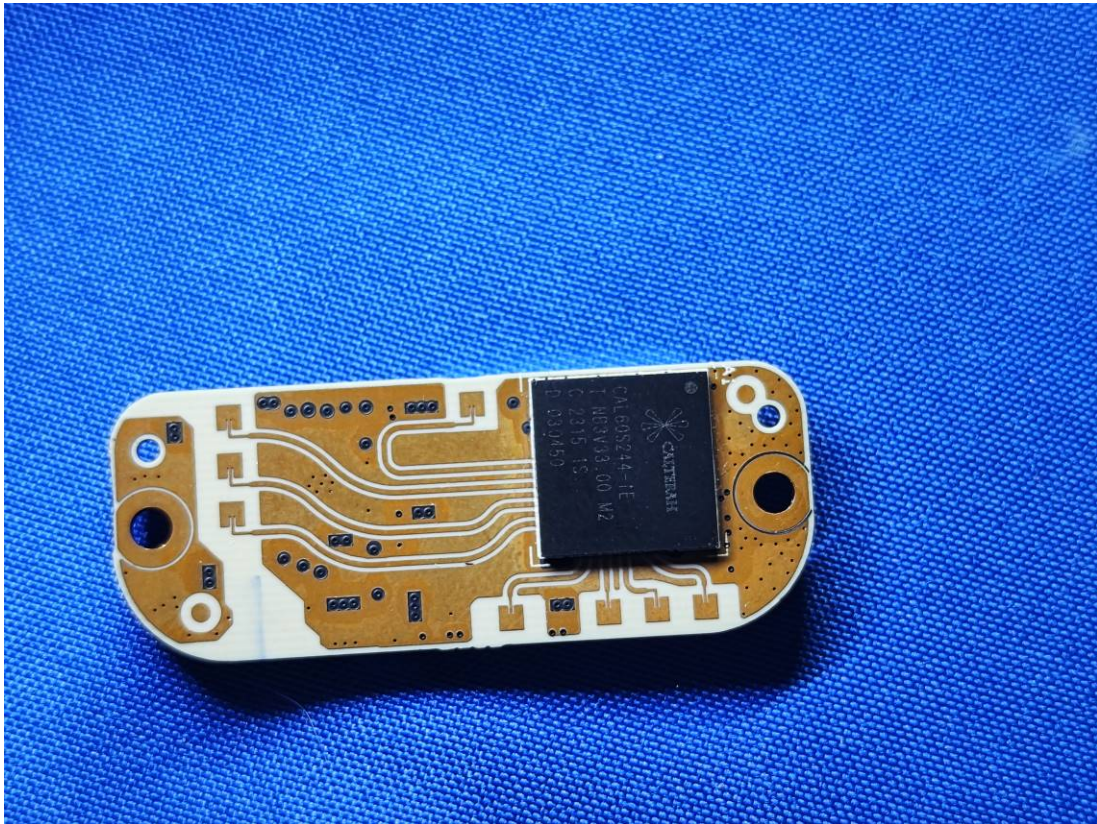
Top radar
