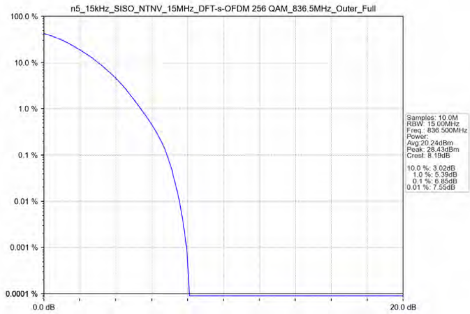
n5_15kHz_SISO_NTNV_15MHz_DFT-s-OFDM_256_QAM_836.5MHz_Outer_Full_Ant11
