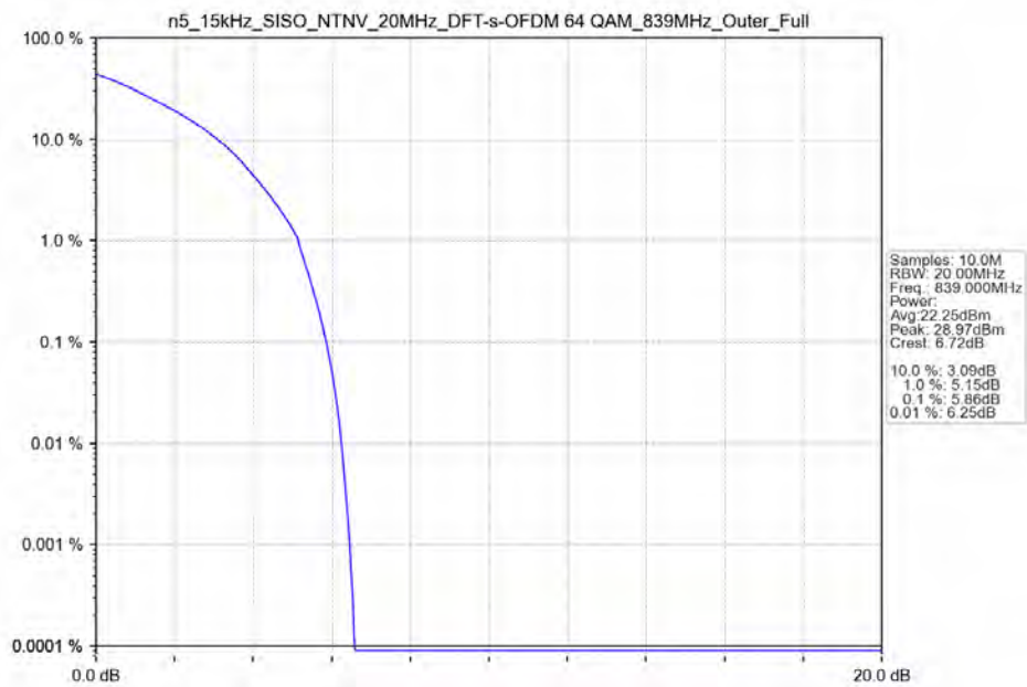
n5_15kHz_SISO_NTNV_20MHz_DFT-s-OFDM_64_QAM_839MHz_Outer_Full_Ant11
