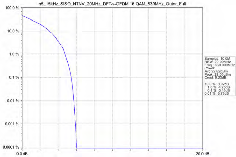
n5_15kHz_SISO_NTNV_20MHz_DFT-s-OFDM 16 QAM_839MHz_Outer_Full_Ant11
