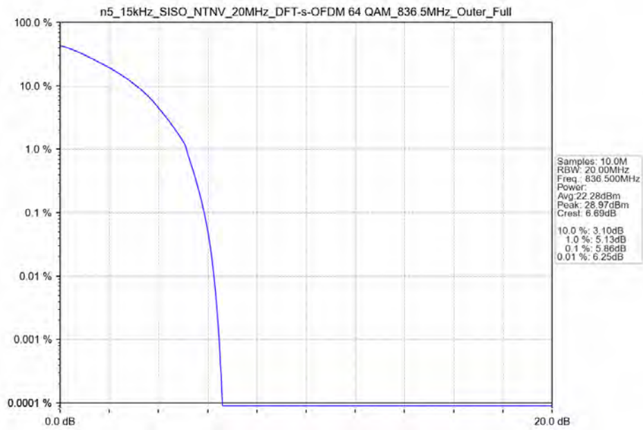
n5_15kHz_SISO_NTNV_20MHz_DFT-s-OFDM_64_QAM_836.5MHz_Outer_Full_Ant11
