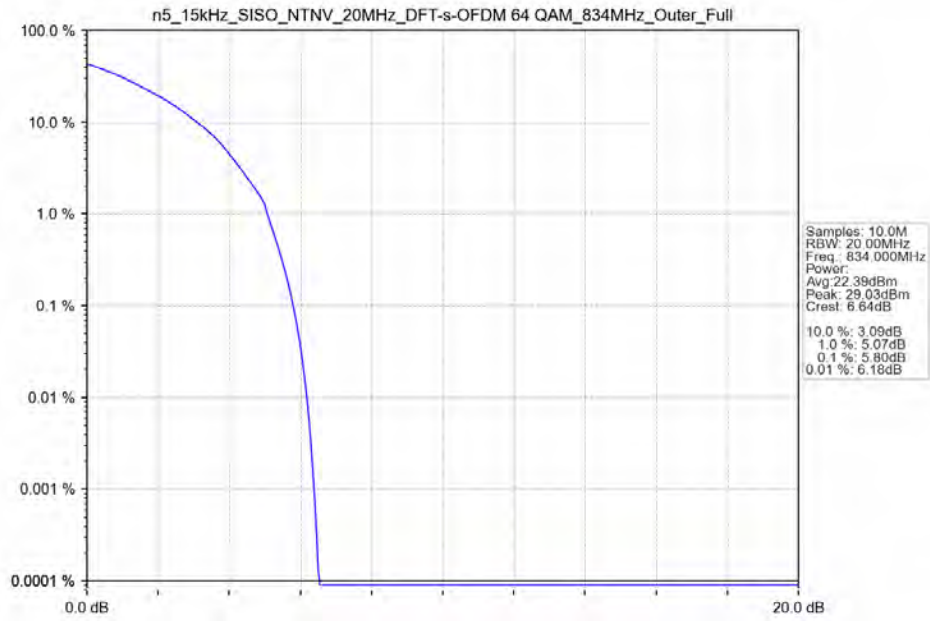
n5_15kHz_SISO_NTNV_20MHz_DFT-s-OFDM 64 QAM_834MHz_Outer_Full_Ant11
