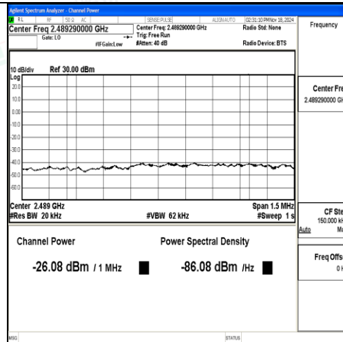
Band41_15MHz_QPSK_39725_75RB#0_Final1
