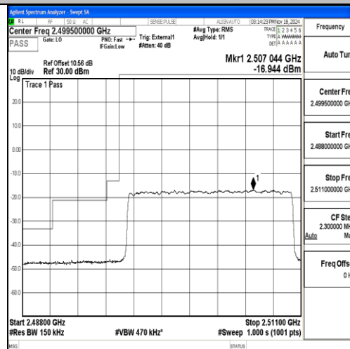
Band41_15MHz_16QAM_39725_75RB#0
