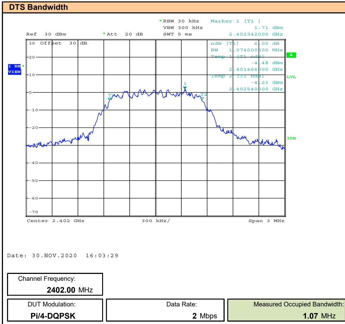
Plot 8.5 – 6dB DTS Bandwidth BT EDR 2MB, 2402MHz
