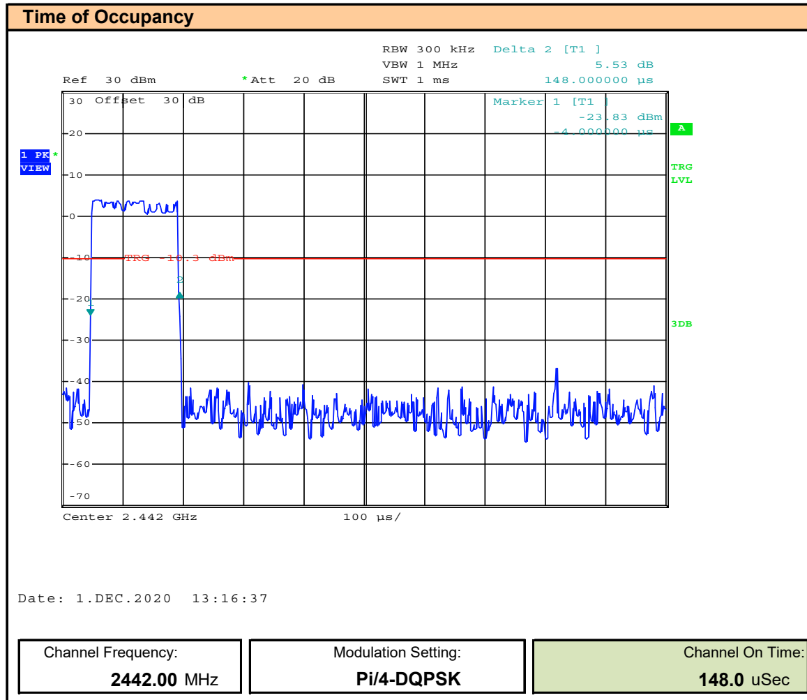
Plot 15.1 – Time of Occupancy, BT EDR 2MB
