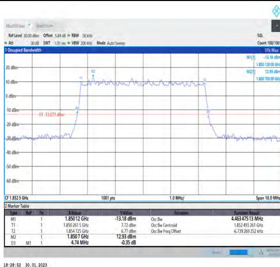
1-N2-PC3-15-5-L-3-DFT-16QAM-Outet_Full-25@0-A Ant1-4.463-4.740-≤5-PASS
