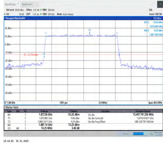
1-N2-PC3-15-15-M-3-DFT-16QAM-Outer_Full-75@0 -Ant1-13.448-14.250-≤15-PASS
