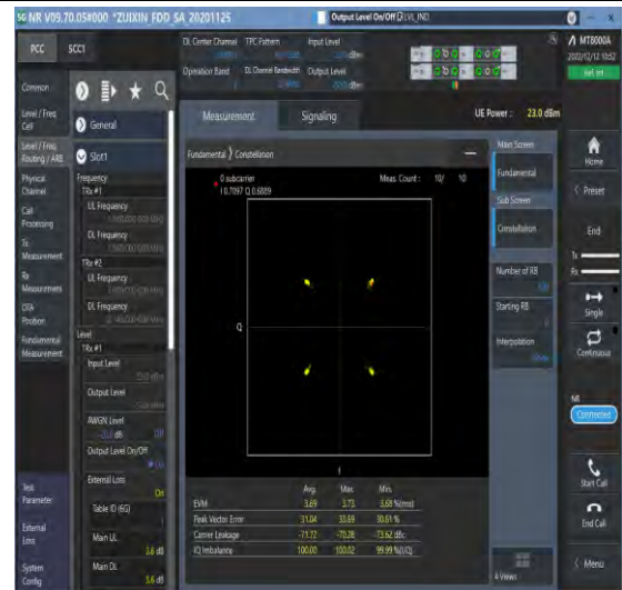
1-N2-PC3-15-20-M-2-DFT-QPSK-Outter_Full-100@ 0-Ant1-see graph-PASS
