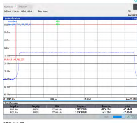
1-N2-PC3-15-10-L-6-CP-QPSK-Outer_Full-52@0-Ant1-1-seegraph-PASS-see graph
