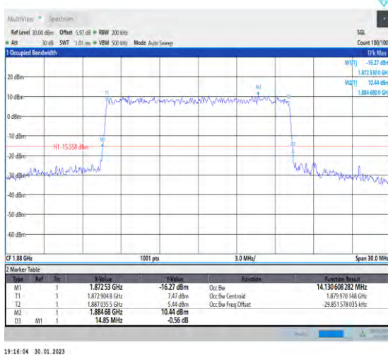
1-N2-PC3-15-15-M-8-CP-64QAM-Outer_Full-79@0- Ant1-14.131-14.850-≤15-PASS
