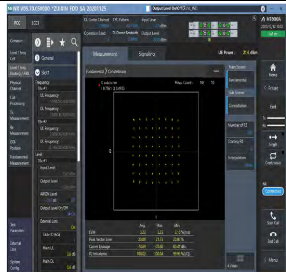
1-N2-PC3-15-20-M-4-DFT-64QAM-Outter_Full-100 @0-Ant1-see graph-PASS
