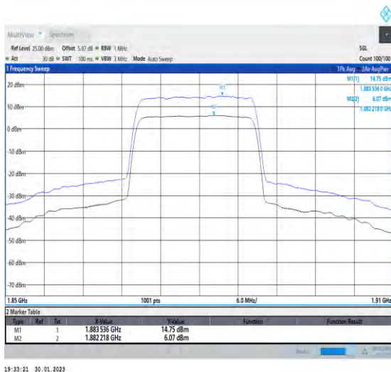
1-N2-PC3-15-20-M-1-DFT-256QAM-Outter_Full-100 @0-Ant1-8.68-100%-0.00-8.68-PASS-≤13
