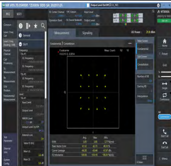
1-N2-PC3-15-20-M-3-DFT-16QAM-Outter_Full-100@ 0-Ant1-see graph-PASS
