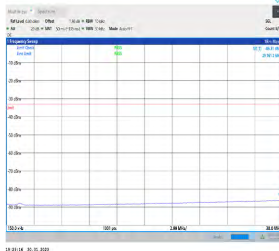
1-N2-PC3-15-20-L-1-DFT-PI2BPSK-Inner_1RB_Left- 1@1-0.15-30-Ant1-29.76--86.31--33-PASS
