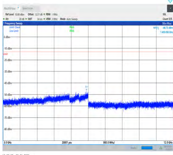
1-N2-PC3-15-20-M-1-DFT-PI2BPSK-Inner_1RB_Lef t-1@1-3000-12000-Ant1-7405.05--46.73--13-PASS
