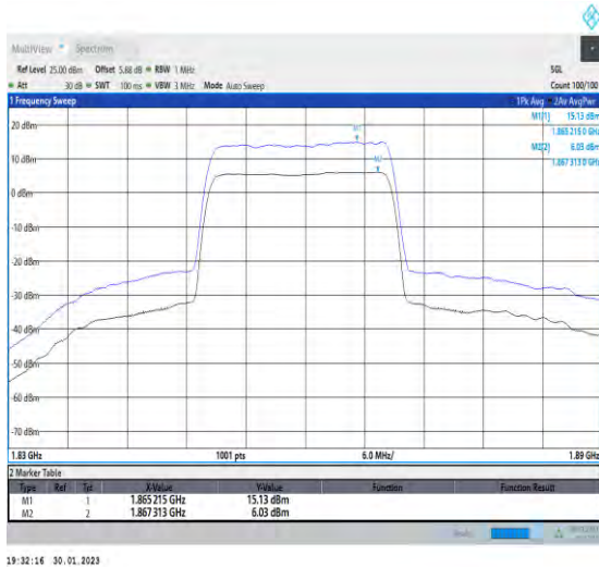
1-N2-PC3-15-20-L-1-DFT-256QAM-Outter_Full-100@ 0-Ant1-9.10-100%-0.00-9.10-PASS-≤13
