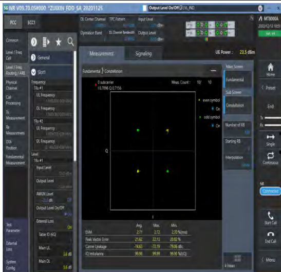
1-N2-PC3-15-20-M-1-DFT-PI2BPSK-Outter_Full-100 @0-Ant1-see graph-PASS
