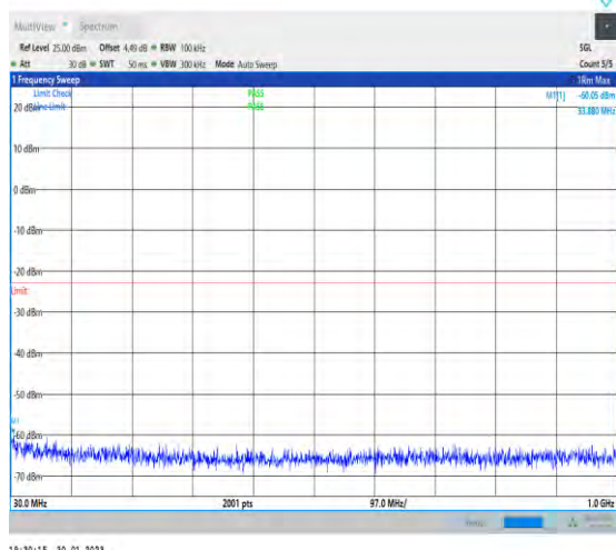
1-N2-PC3-15-20-M-1-DFT-PI2BPSK-Inner_1RB_Lef t-1@1-30-1000-Ant1-33.88--60.05--23-PASS
