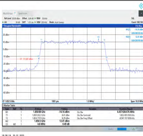
1-N2-PC3-15-5-L-1-DFT-QPSK-Outet_Full-25@0-An t1-4.458-4.800-≤5-PASS
