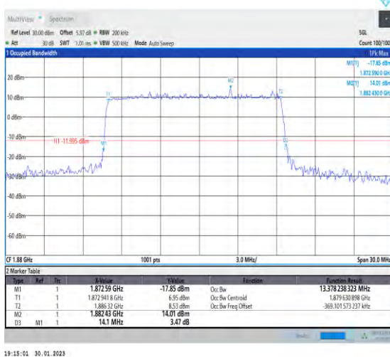
1-N2-PC3-15-15-M-4-DFT-64QAM-Outer_Full-75@0 -Ant1-13.378-14.100-≤15-PASS
