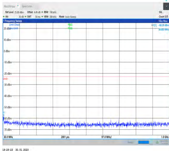
1-N2-PC3-15-20-L-1-DFT-PI2BPSK-Inner_1RB_Left -1@1-30-1000-Ant1-34.85--58.29--23-PASS
