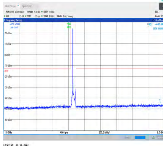
1-N2-PC3-15-20-L-1-DFT-PI2BPSK-Inner_1RB_Left- 1@1-1000-3000-Ant1-2938.00--44.80--13-PASS
