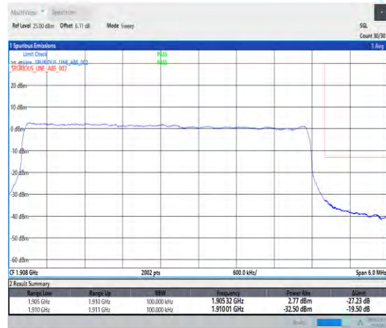
1-N2-PC3-15-5-H-3-DFT-PI2BPSK-Outer_Full-25 @0-Ant1-1-seegraph-PASS-see graph
