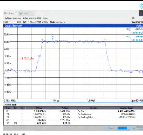
1-N2-PC3-15-5-L-2-DFT-PI2BPSK-Outet_Full-25@0 -Ant1-4.461-4.880-≤5-PASS
