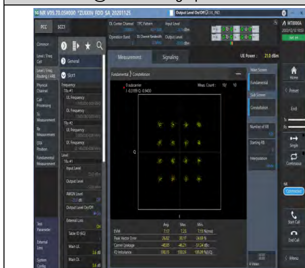
1-N2-PC3-15-20-M-7-CP-16QAM-Outer_Full-106@0- Ant1-see graph-PASS
