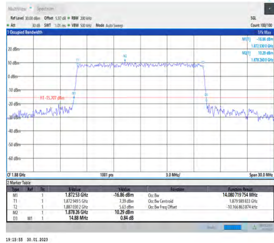
1-N2-PC3-15-15-M-7-CP-16QAM-Outer_Full-79@0- Ant1-14.081-14.880-≤15-PASS
