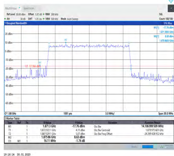
1-N2-PC3-15-15-M-9-CP-256QAM-Outer_Full-79@0- -Ant1-14.107-16.110-≤15-PASS
