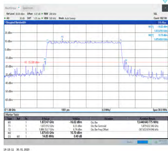
1-N2-PC3-15-15-M-5-DFT-256QAM-Outer_Full-75@ 0-Ant1-13.441-14.850-≤15-PASS
