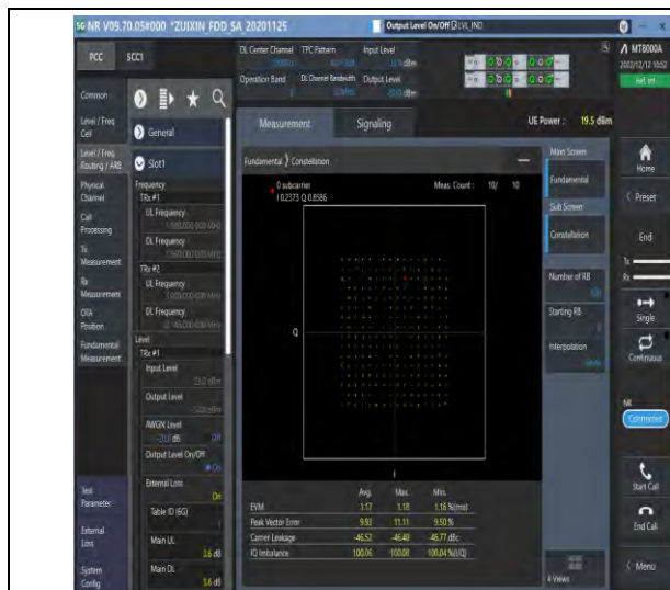
1-N2-PC3-15-20-M-5-DFT-256QAM-Outer_Full-100 @0-Ant1-see graph-PASS
