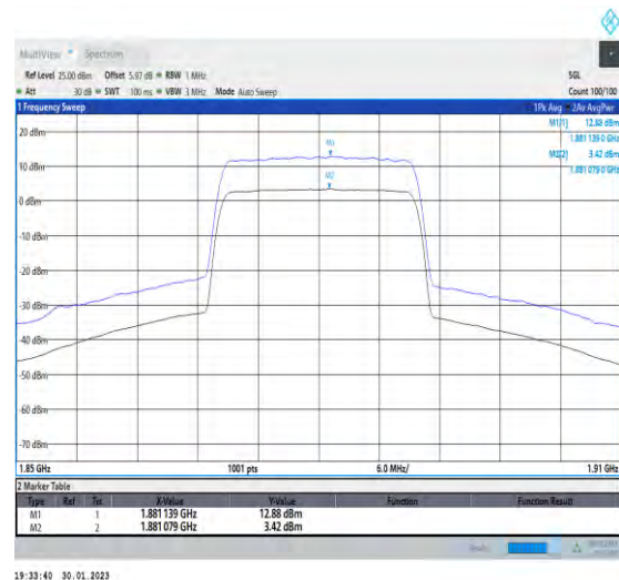
1-N2-PC3-15-20-M-2-CP-256QAM-Outter_Full-106 @0-Ant1-9.46-100%-0.00-9.46-PASS-≤13
