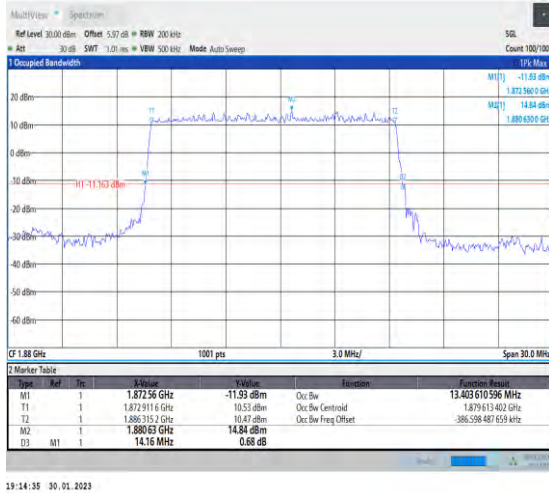
1-N2-PC3-15-15-M-2-DFT-PI2BPSK-Outer_Full-75 @0-Ant1-13.404-14.160-≤15-PASS
