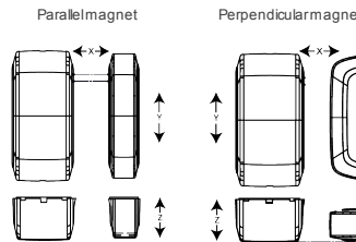
Figure 5: Range coverage directions
