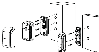
Figure 2: Mounting on a flat surface
