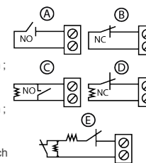
Figure 6: Auxiliary wiring options
