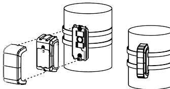
Figure 3: Mounting on a curved surface with straps
