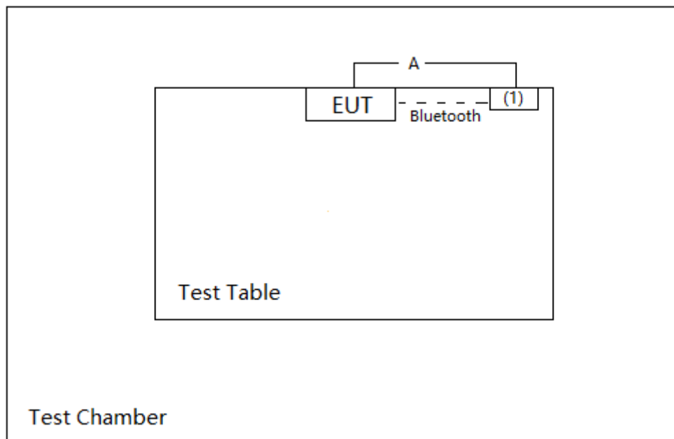
Connection Diagram
