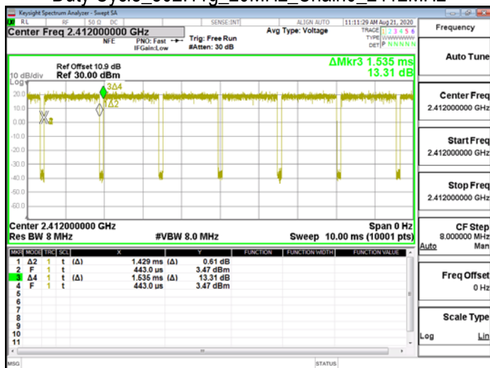
Duty Cycle_802.11g_20MHz_Chain0_2412MHz
