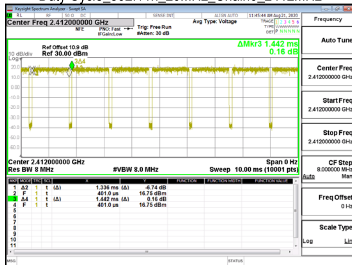
Duty Cycle_802.11n_20MHz_Chain0_2412MHz
