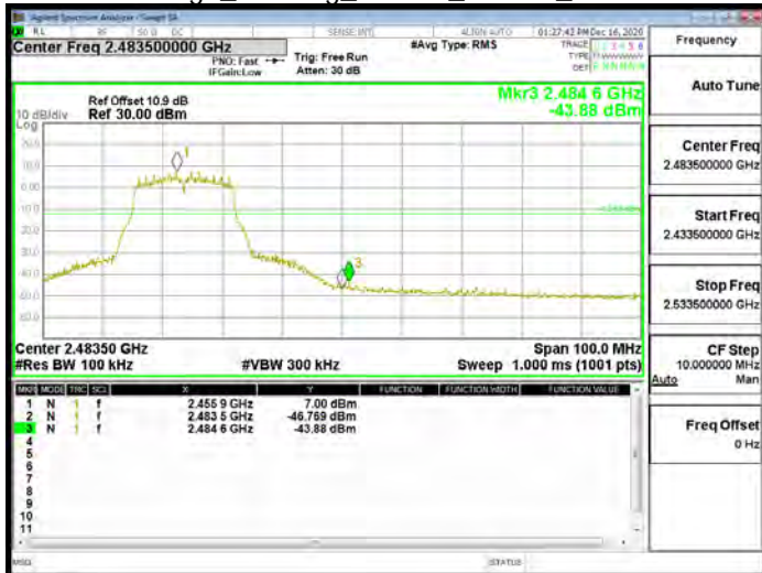
Band Edge_802.11g_20MHz_Chain0_2462MHz
