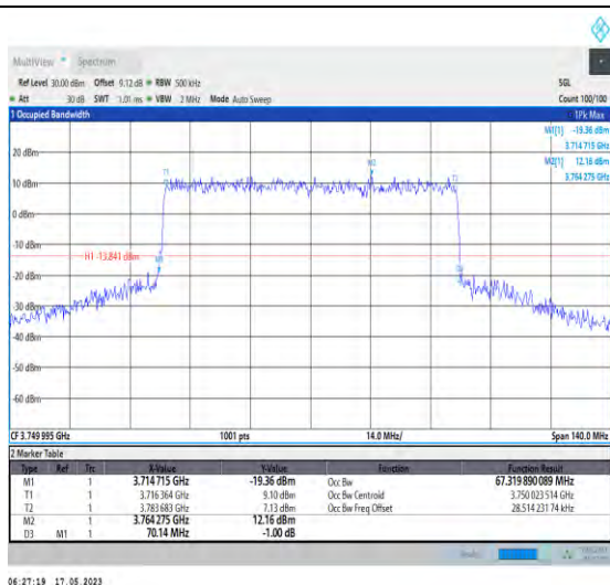
1-N78-3700-3800-PC1-30-70-M-7-CP-16QAM-Outer _Full-189@0-Ant0-67.32-70.140-≤70-PASS
