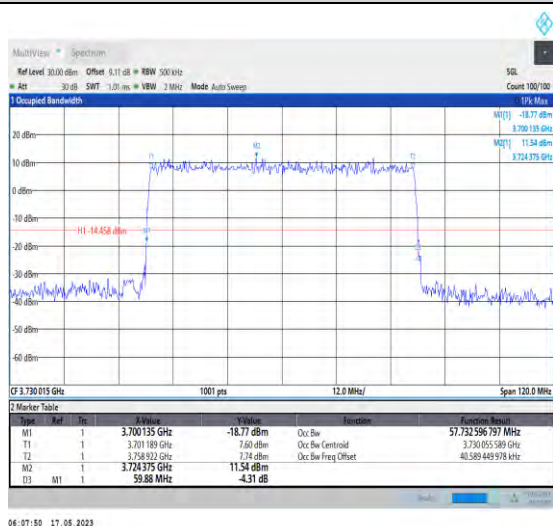
1-N78-3700-3800-PC1-30-60-L-5-DFT-256QAM-Outer_Full-162@0-Ant0-57.733-59.880-≤60-PASS
