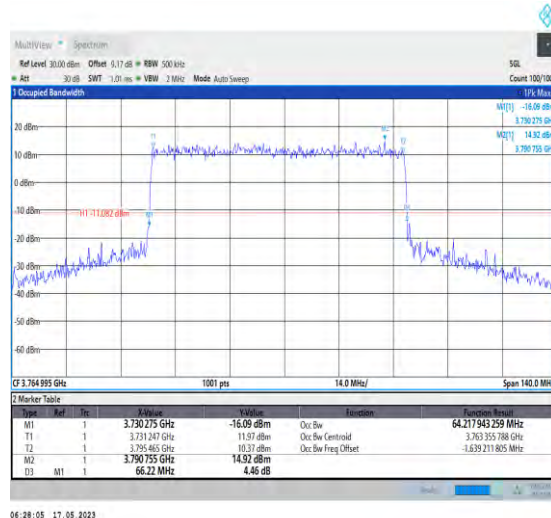
1-N78-3700-3800-PC1-30-70-H-1-DFT-QPSK-Outer _Full-180@0-Ant0-64.218-66.220-≤70-PASS
