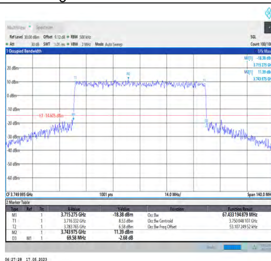
1-N78-3700-3800-PC1-30-70-M-8-CP-64QAM-Outer _Full-189@0-Ant0-67.433-69.580-≤70-PASS
