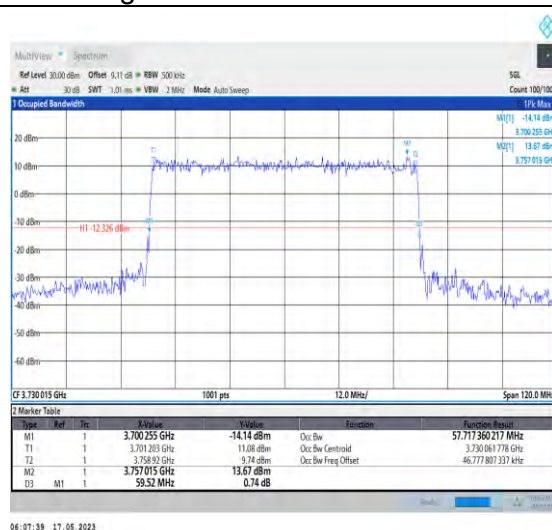
1-N78-3700-3800-PC1-30-60-L-4-DFT-64QAM-Outer_Full-162@0-Ant0-57.717-59.520-≤60-PASS
