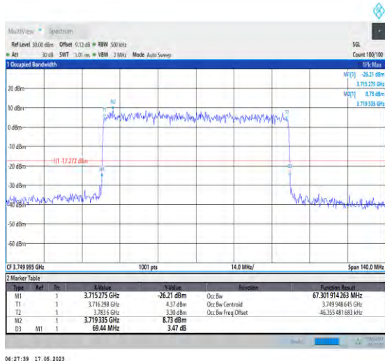
1-N78-3700-3800-PC1-30-70-M-9-CP-256QAM-Outer _Full-189@0-Ant0-67.302-69.440-≤70-PASS
