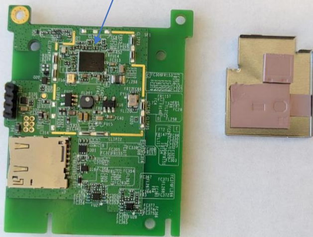
WiFi Chip
