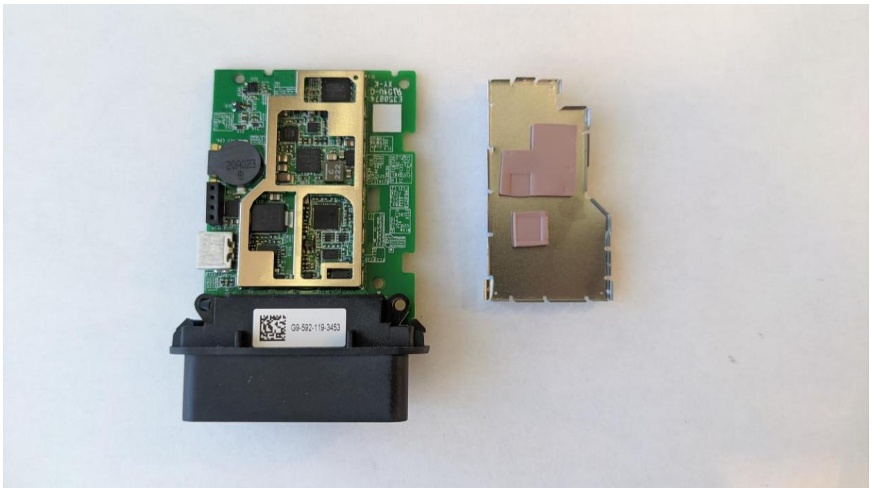
Mainboard with shielding removed
