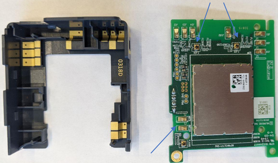
WiFi Antenna PCB Contact Points
