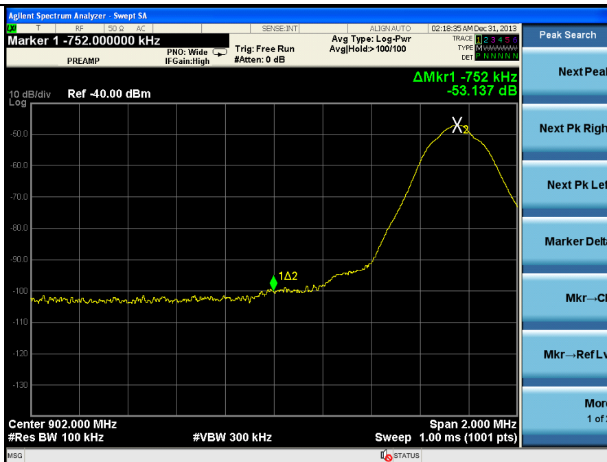
100 KHz Bandwidth of Frequency Band Edge-Low Channel
