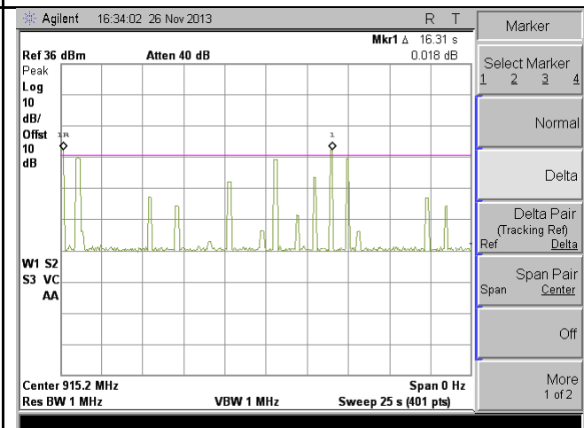
FCC-15.247-DwT-Cycle-915.25M
