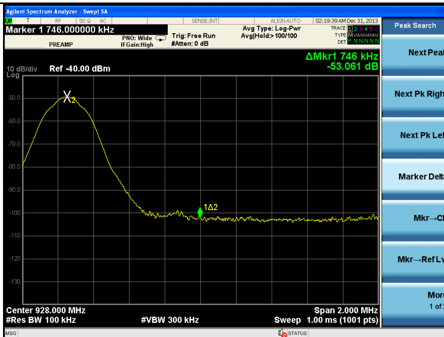
100 KHz Bandwidth of Frequency Band Edge -High Channel
