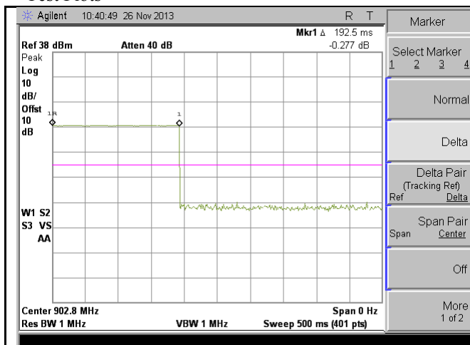
FCC-15.247-DwT-902.75M
