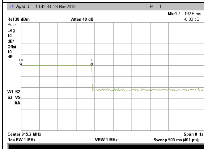
FCC-15.247-DwT-915.25M
