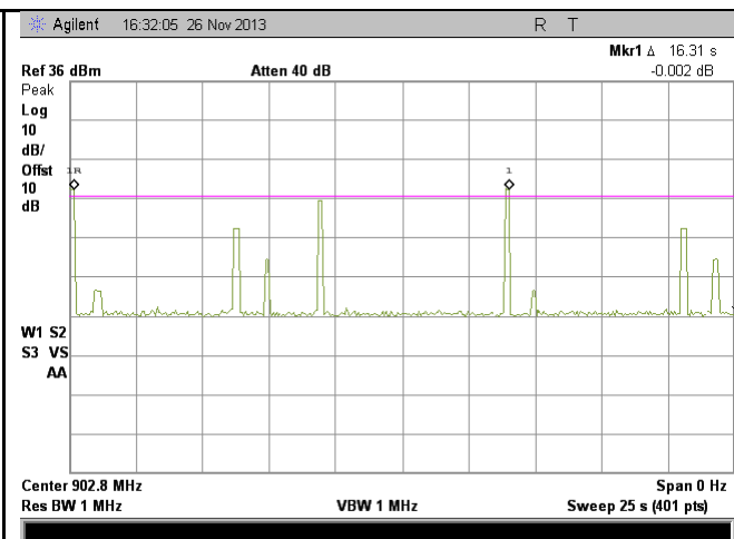
FCC-15.247-DwT-Cycle-902.75M
