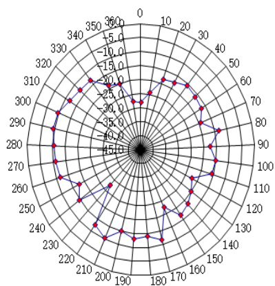
Vertical at 2440MHz
