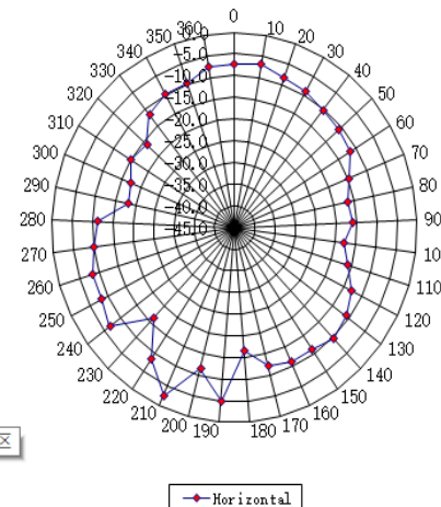
Horizontal at 2402MHz
