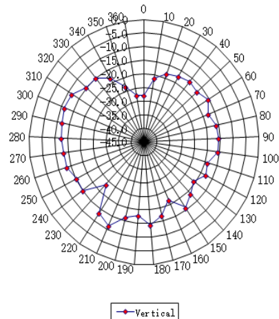
Vertical at 2402MHz
