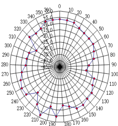
Horizontal at 2480MHz
