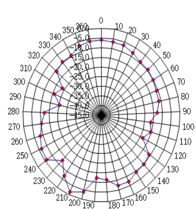
Horizontal at 2440MHz
