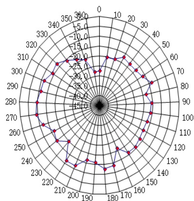
Vertical at 2480MHz
