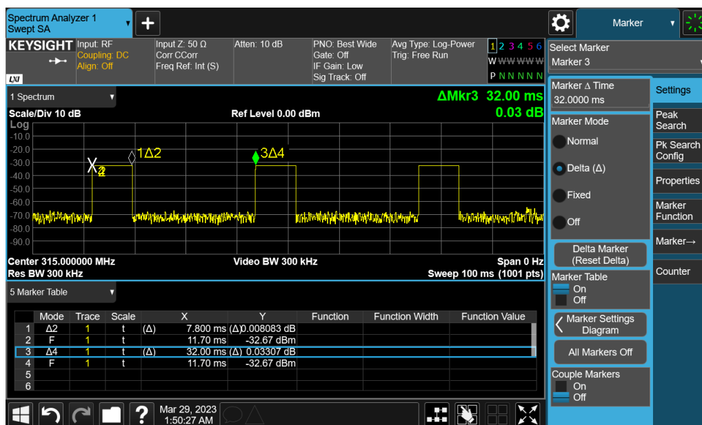
315MHz on time Plot
