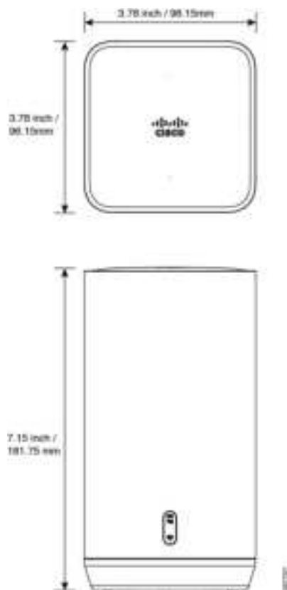
Figure 12: Product Dimensions
