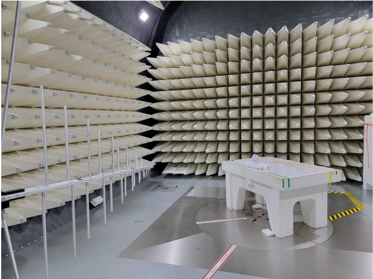
Photograph 1: View Test Set Up Radiated Emissions 30 – 1000 MHz
