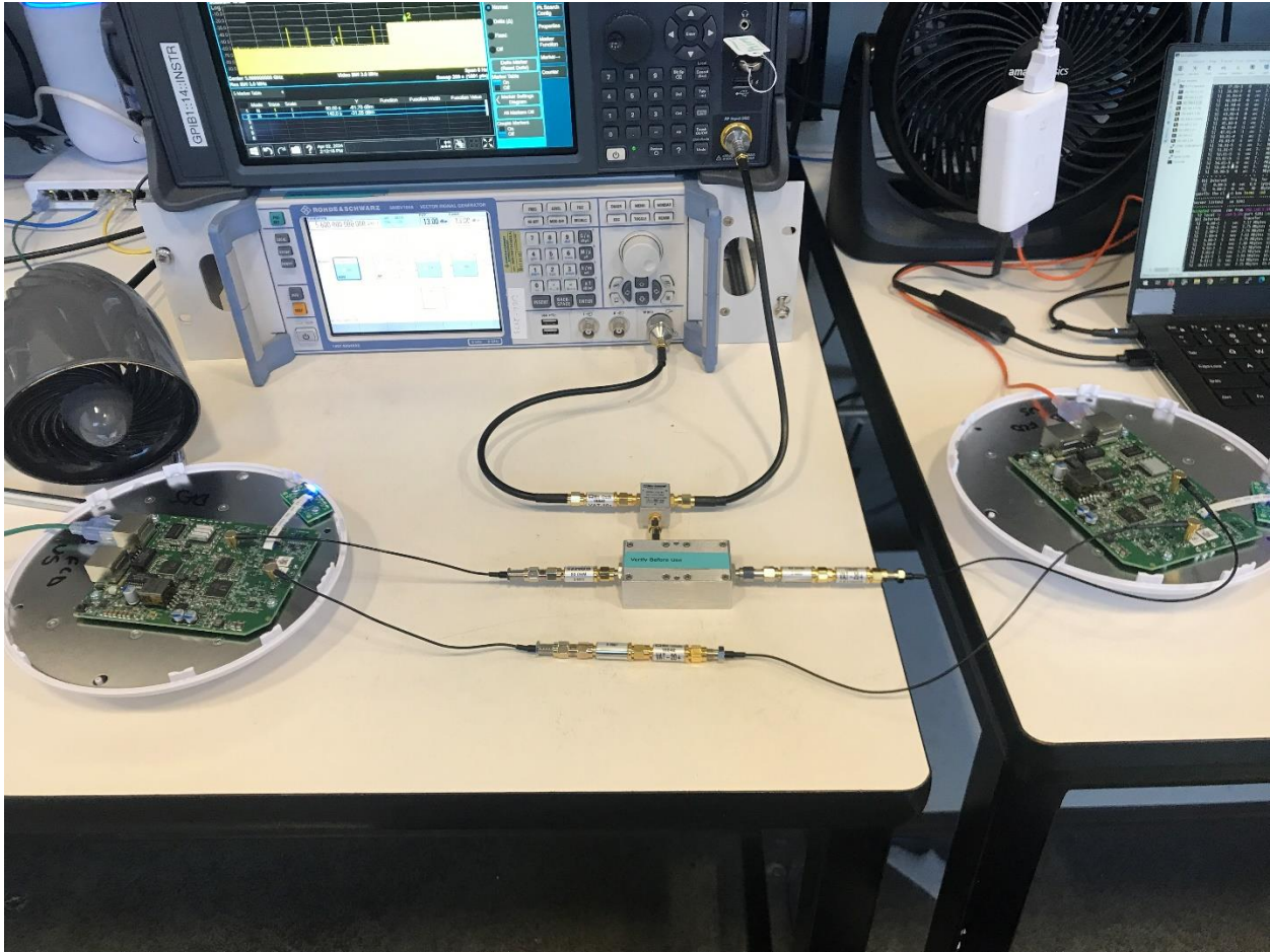
Photograph 5: View Test Set Up DFS Conducted
