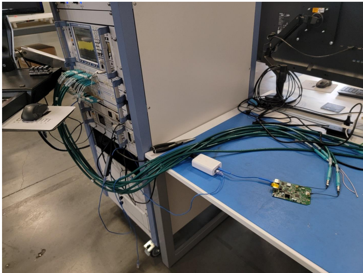
Photograph 4: View Test Set Up RF Conducted
